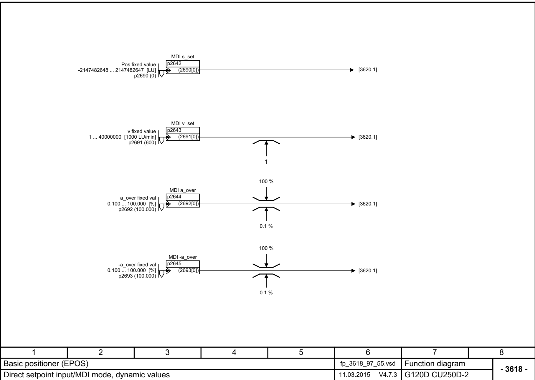
Fig. 3-91 3618 – Direct setpoint specification / MDI mode, dynamic values
