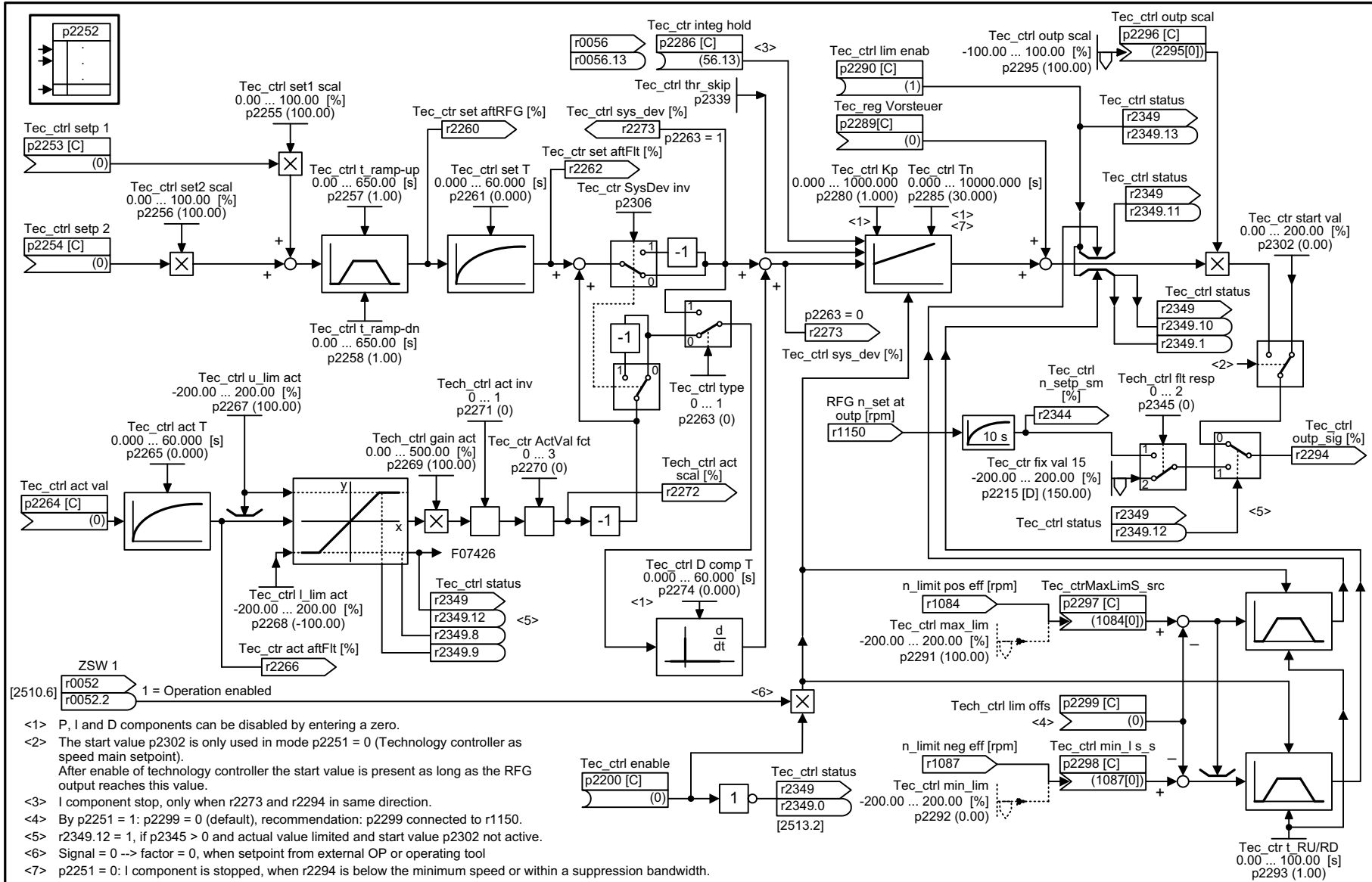
Fig. 3-158 7958 – Closed-loop control
