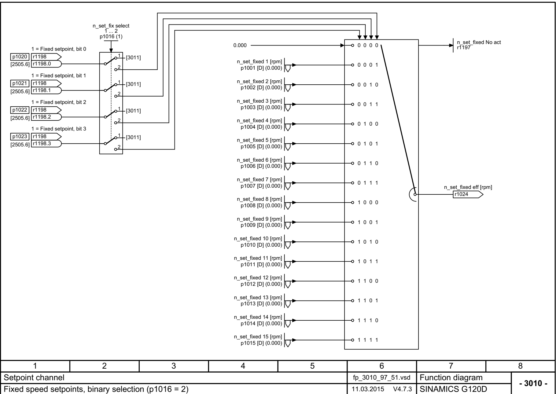
Fig. 3-76 3010 – Fixed speed setpoints, binary selection (p1016 = 2)
