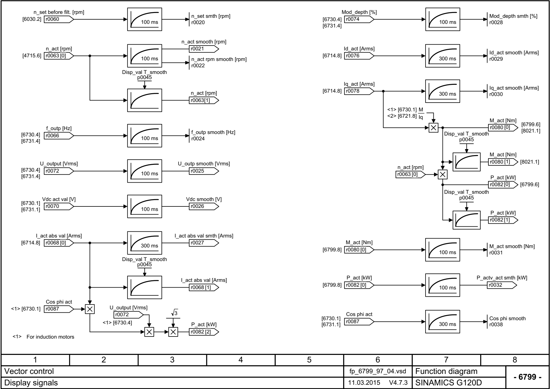
Fig. 3-133 6799 – Display signals
