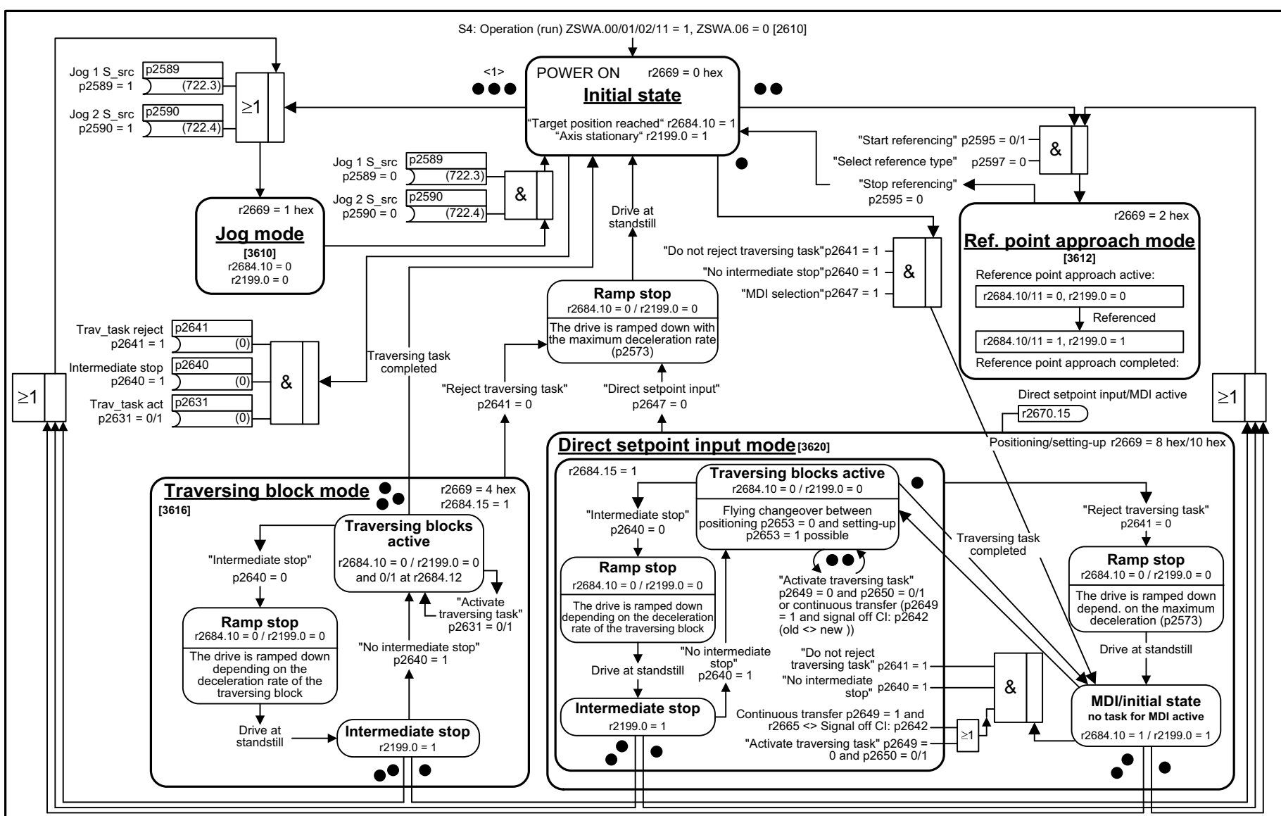
Fig. 3-93 3625 – Mode control
