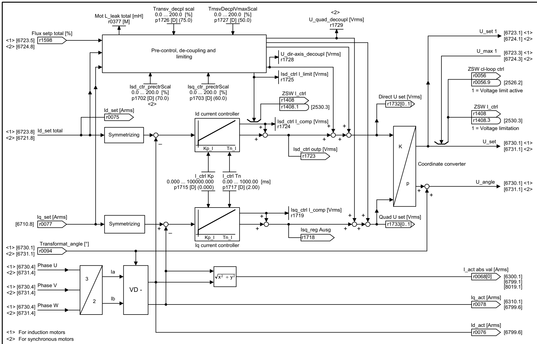
Fig. 3-126 6714 – Iq and Id controllers
