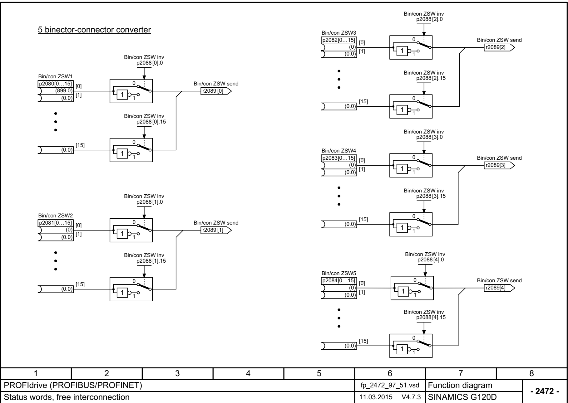
Fig. 3-34 2472 – Status words, free interconnection
