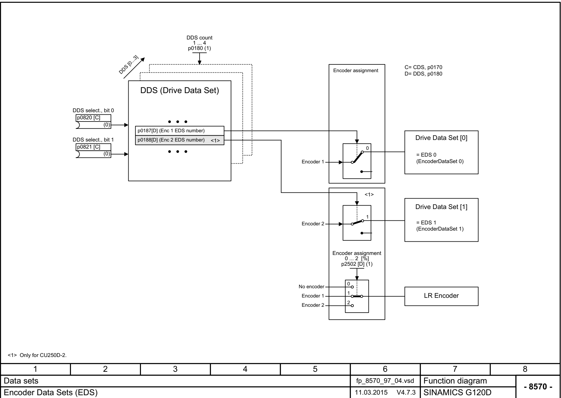
Fig. 3-176 8570 – Encoder Data Sets (EDS)
