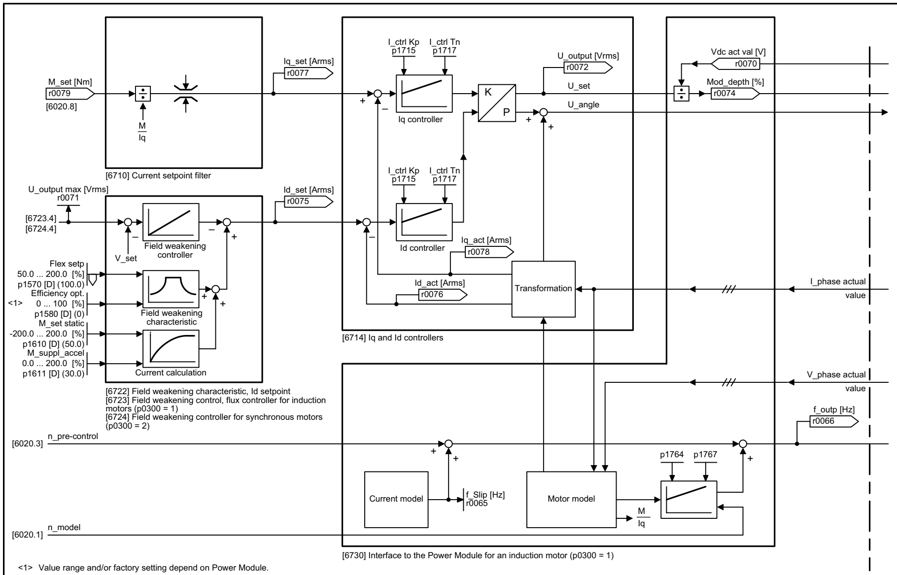
Fig. 3-124 6700 – Current control, overview
