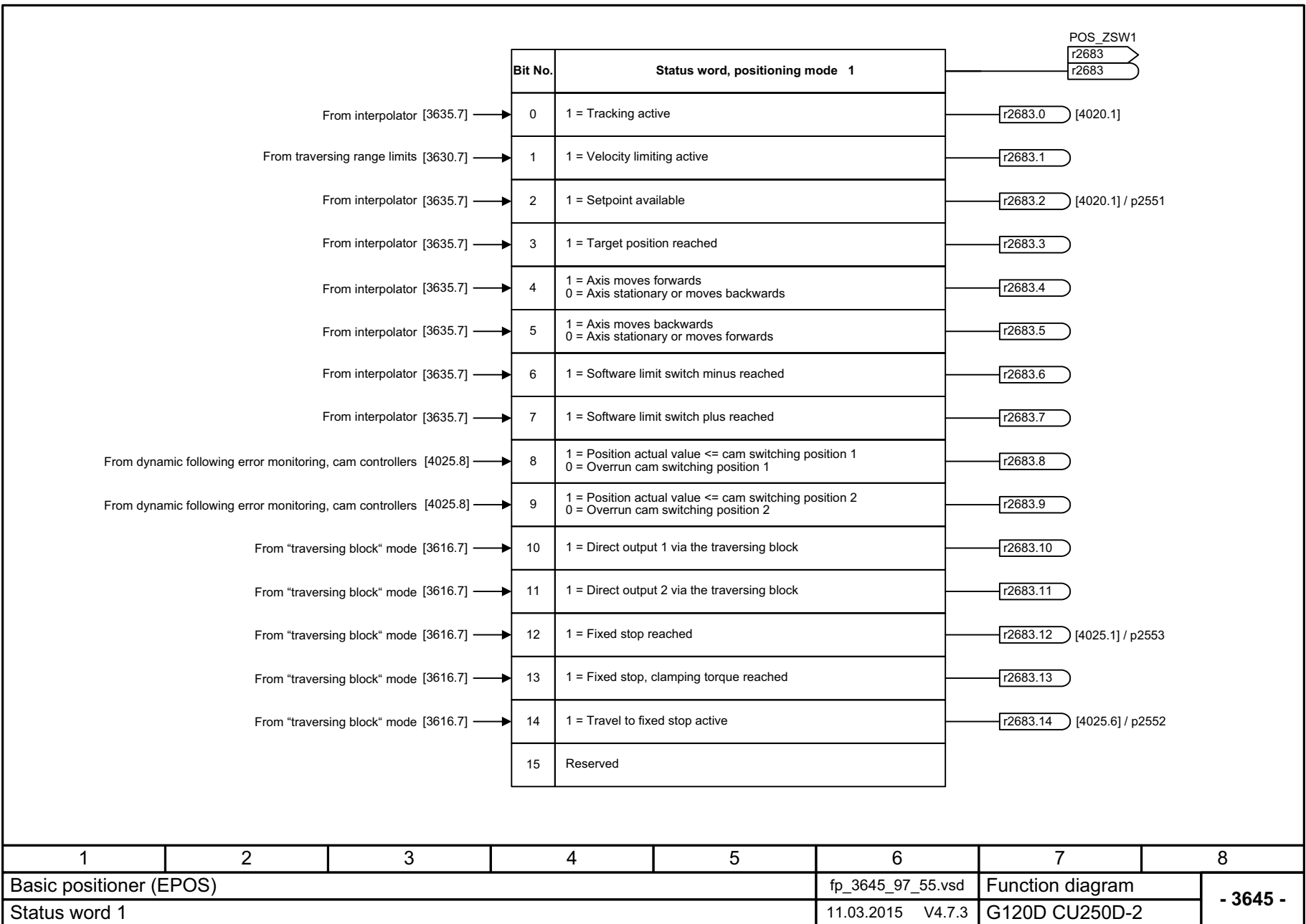
Fig. 3-97 3645 – Status word 1
