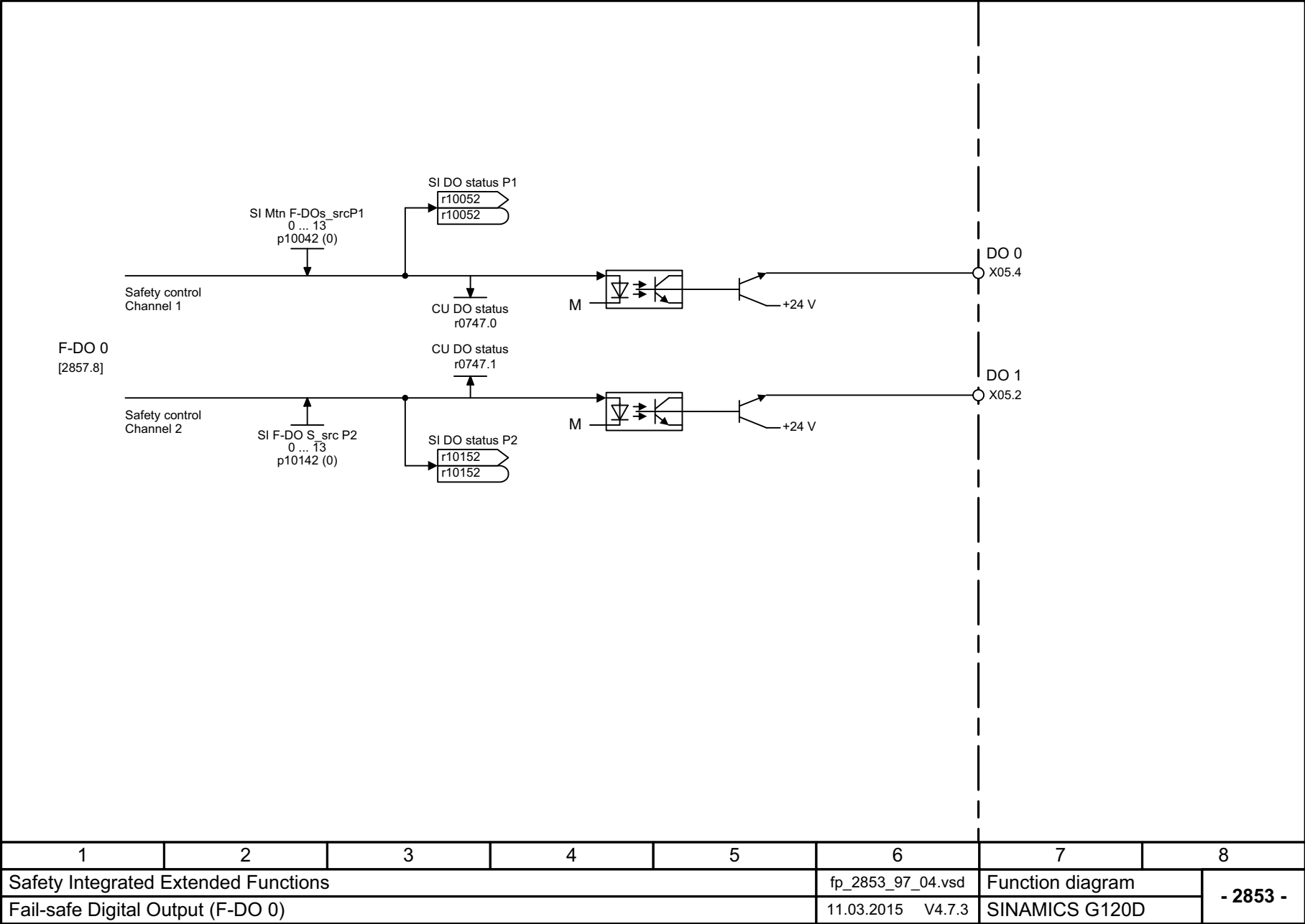
Fig. 3-68 2853 – Fail-safe digital output (F-DO 0)
