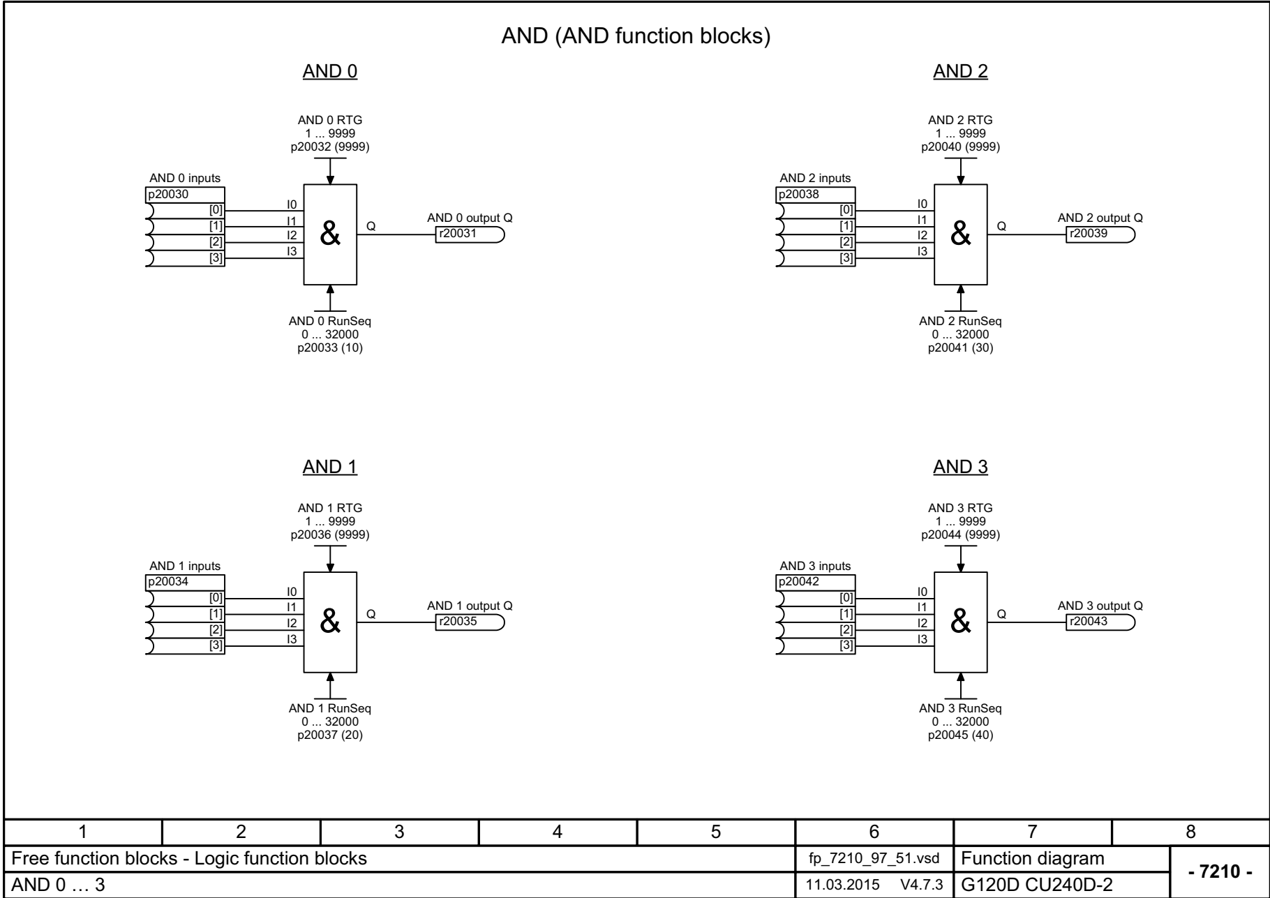
Fig. 3-136 7210 – AND 0 ... 3
