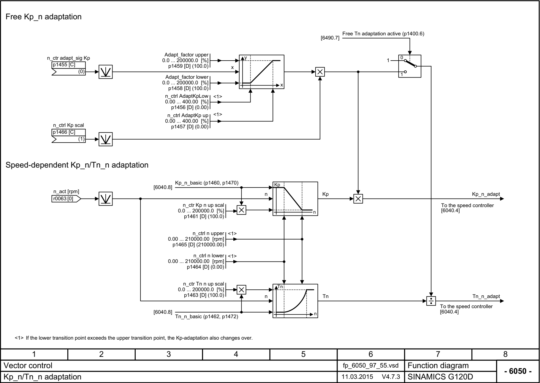
Fig. 3-115 6050 – Kp_n/Tn_n adaptation
