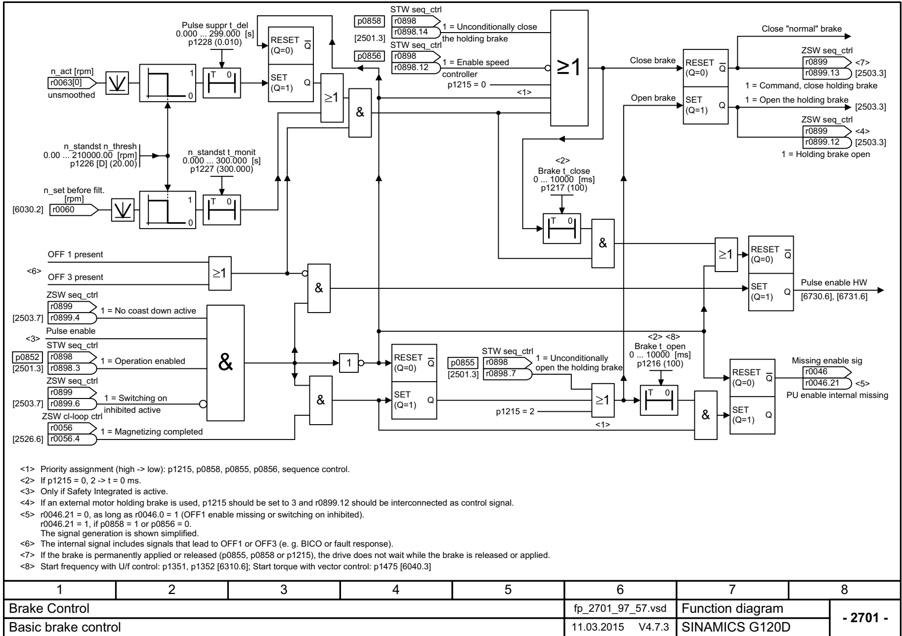
Fig. 3-56 2701 – Basic brake control
