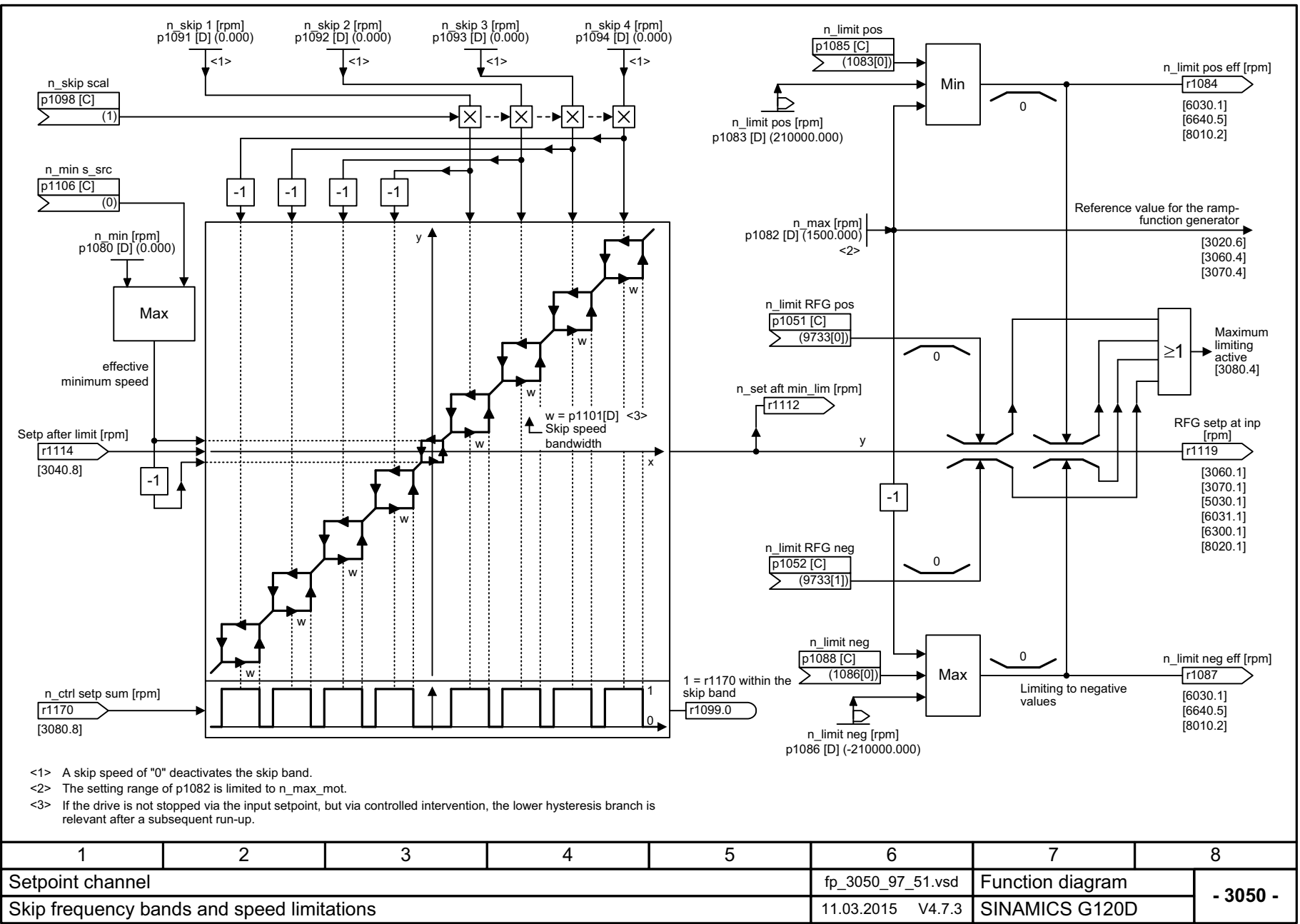
Fig. 3-81 3050 – Skip frequency bands and speed limitations
