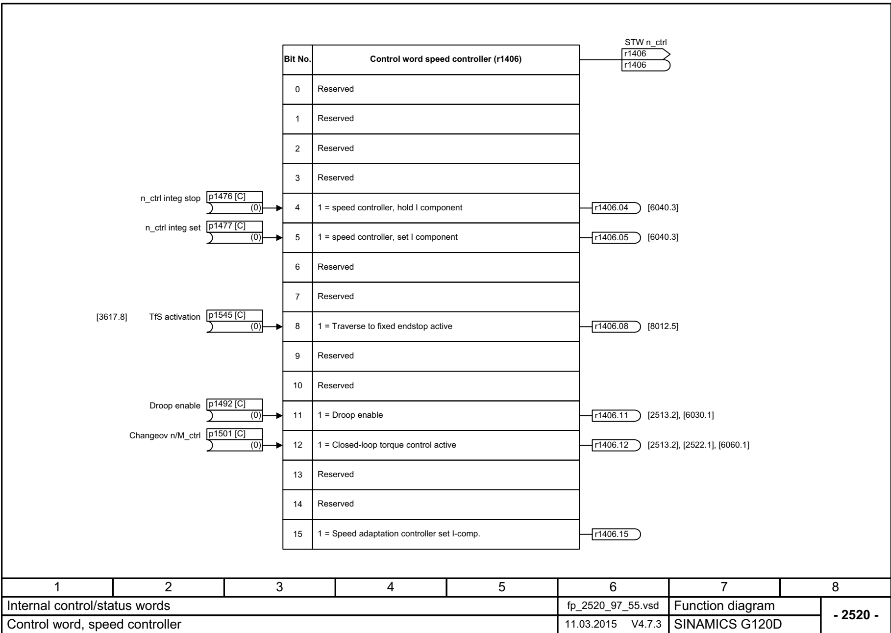
Fig. 3-45 2520 – Control word, speed controller
