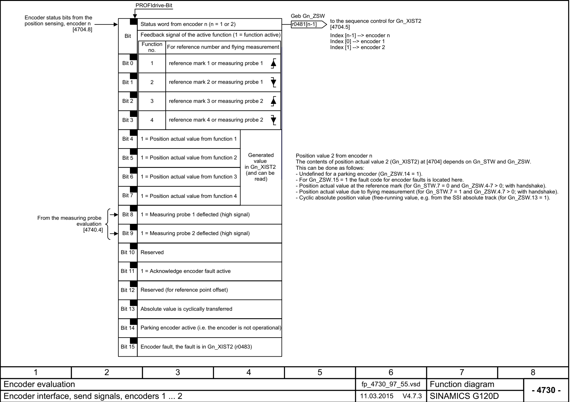
Fig. 3-107 4730 – Encoder interface, send signals, encoders 1 ... 2
