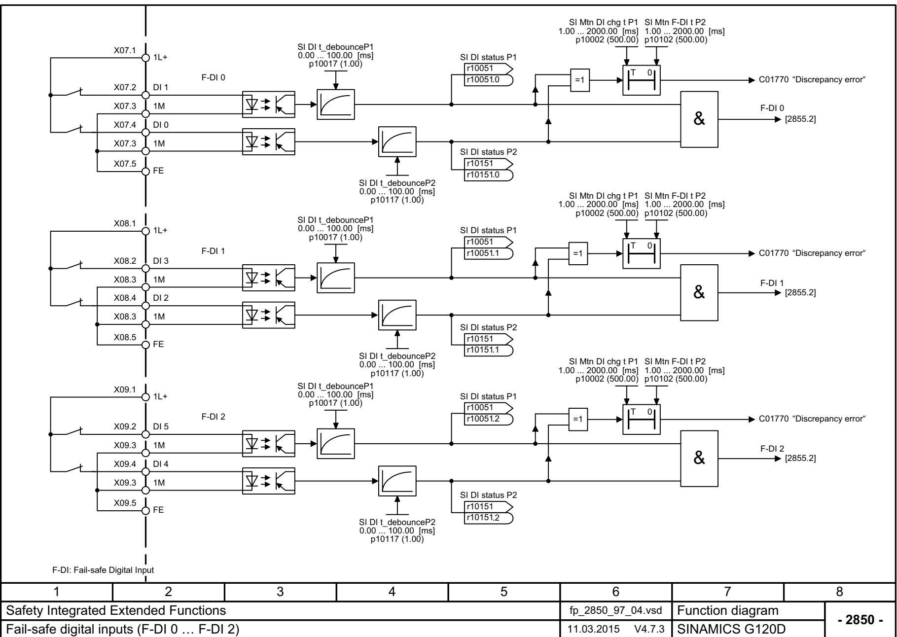
Fig. 3-67 2850 – Fail-safe digital inputs (F-DI 0 ... F-DI 2)
