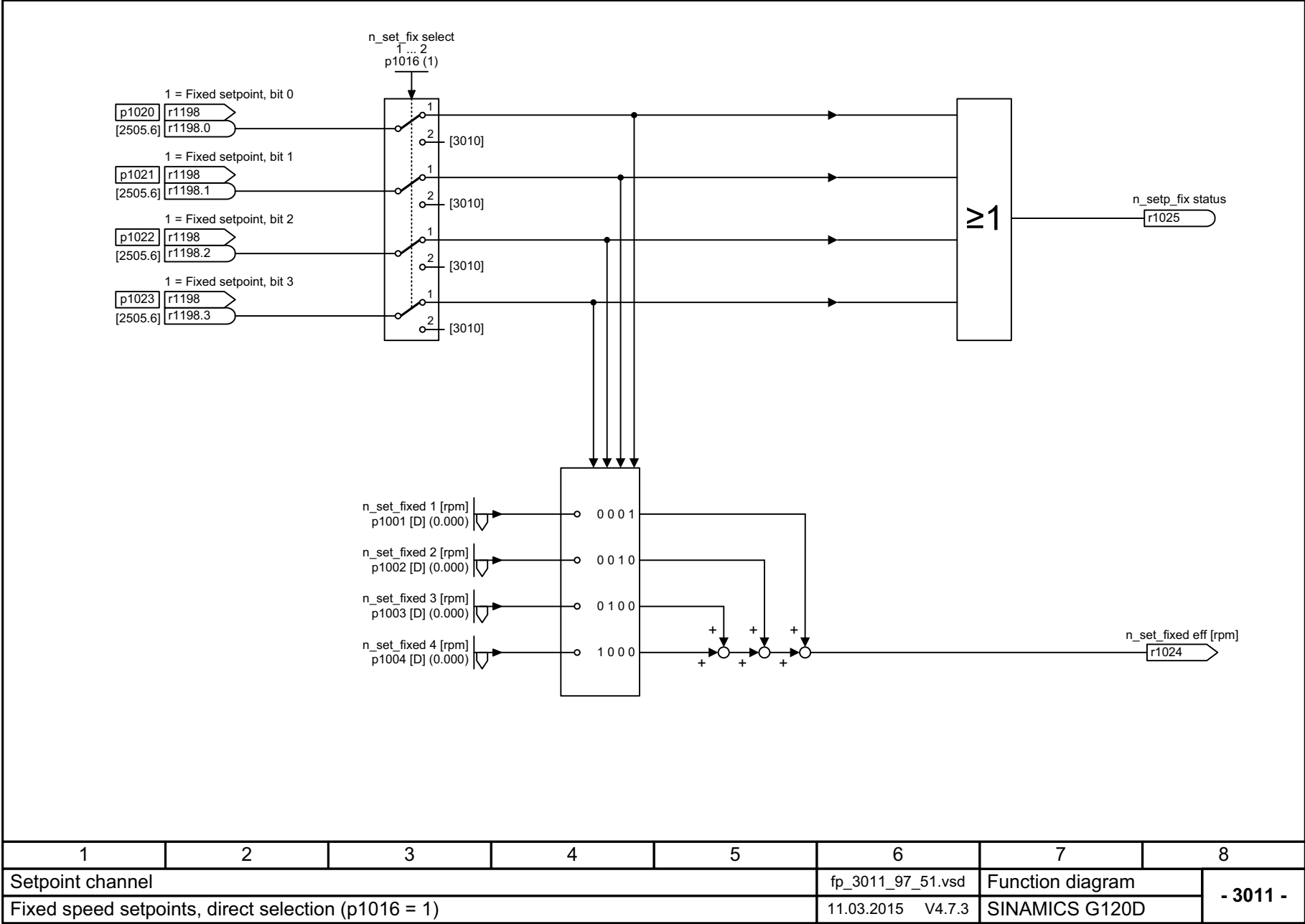
Fig. 3-77 3011 – Fixed speed setpoints, direct selection (p1016 = 1)
