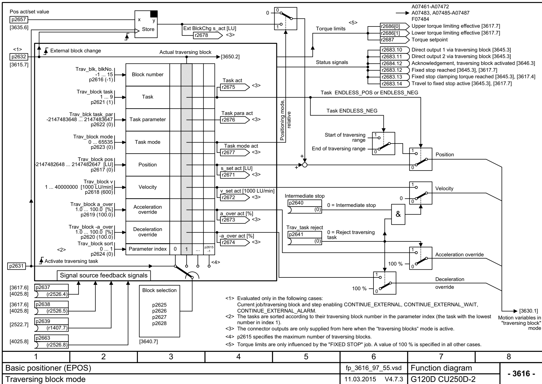
3 Function diagrams 3.12 Basic positioner (EPOS)
