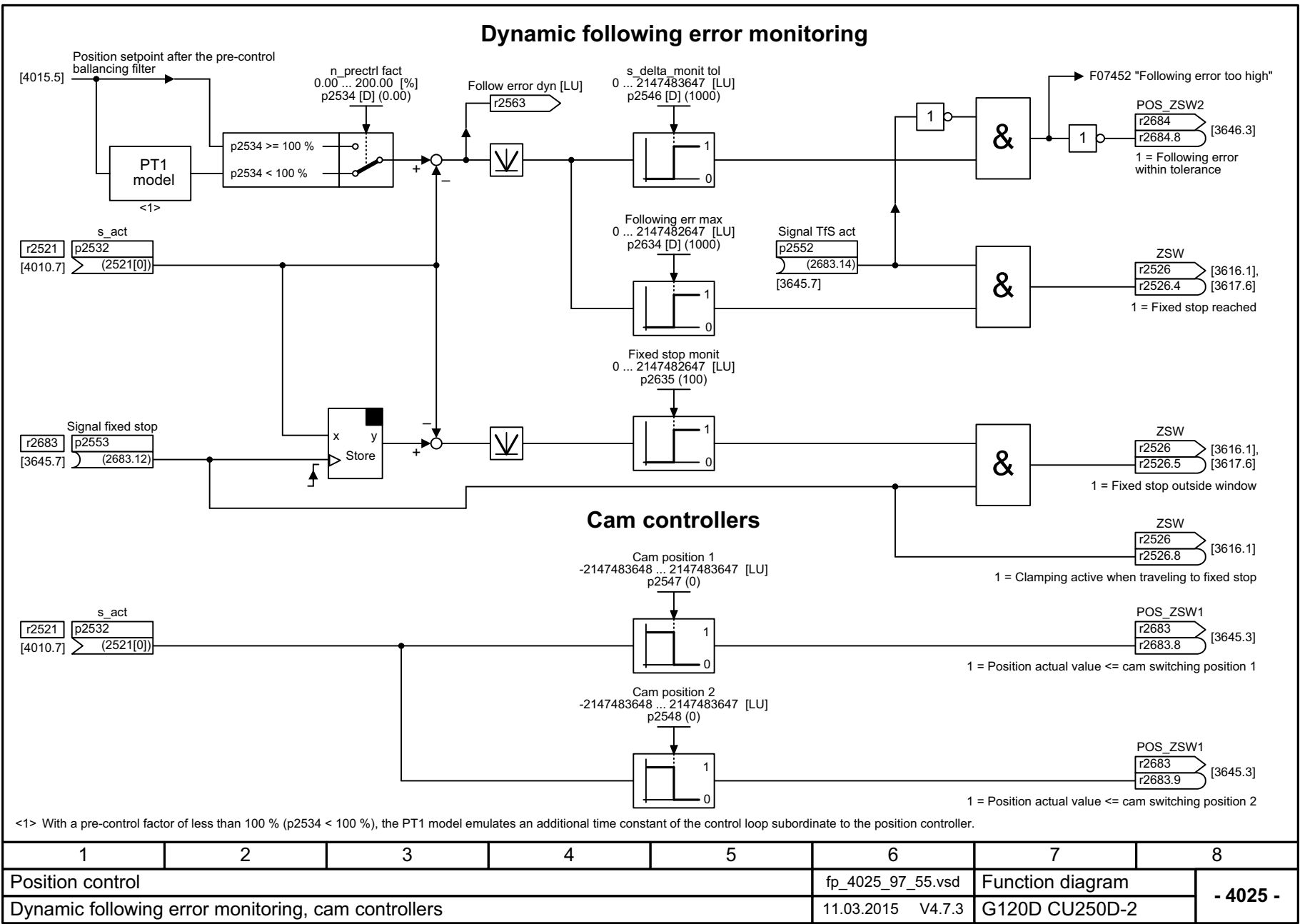
Fig. 3-103 4025 – Dynamic following error monitoring, cam controllers
