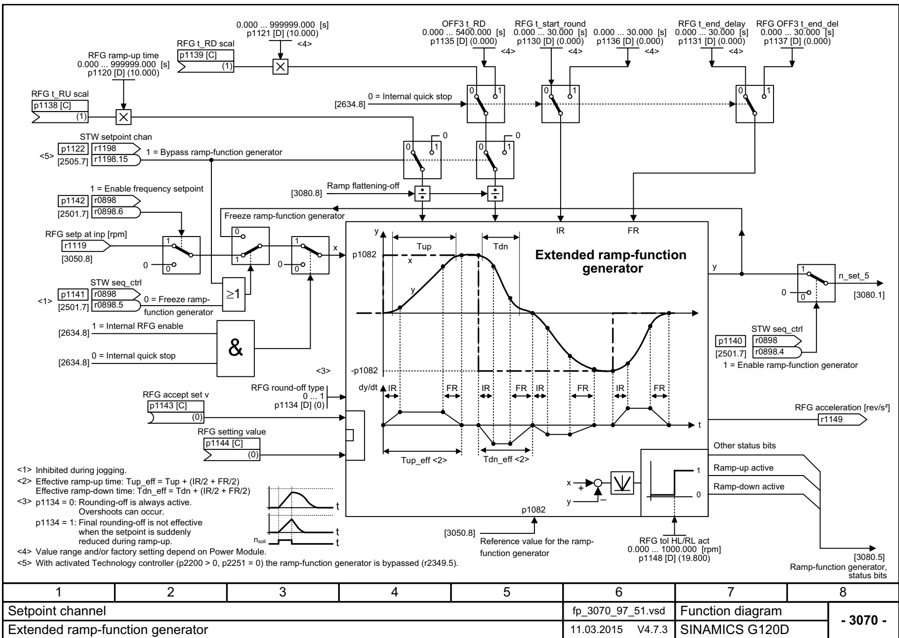
3070 – Extended ramp-function generator
