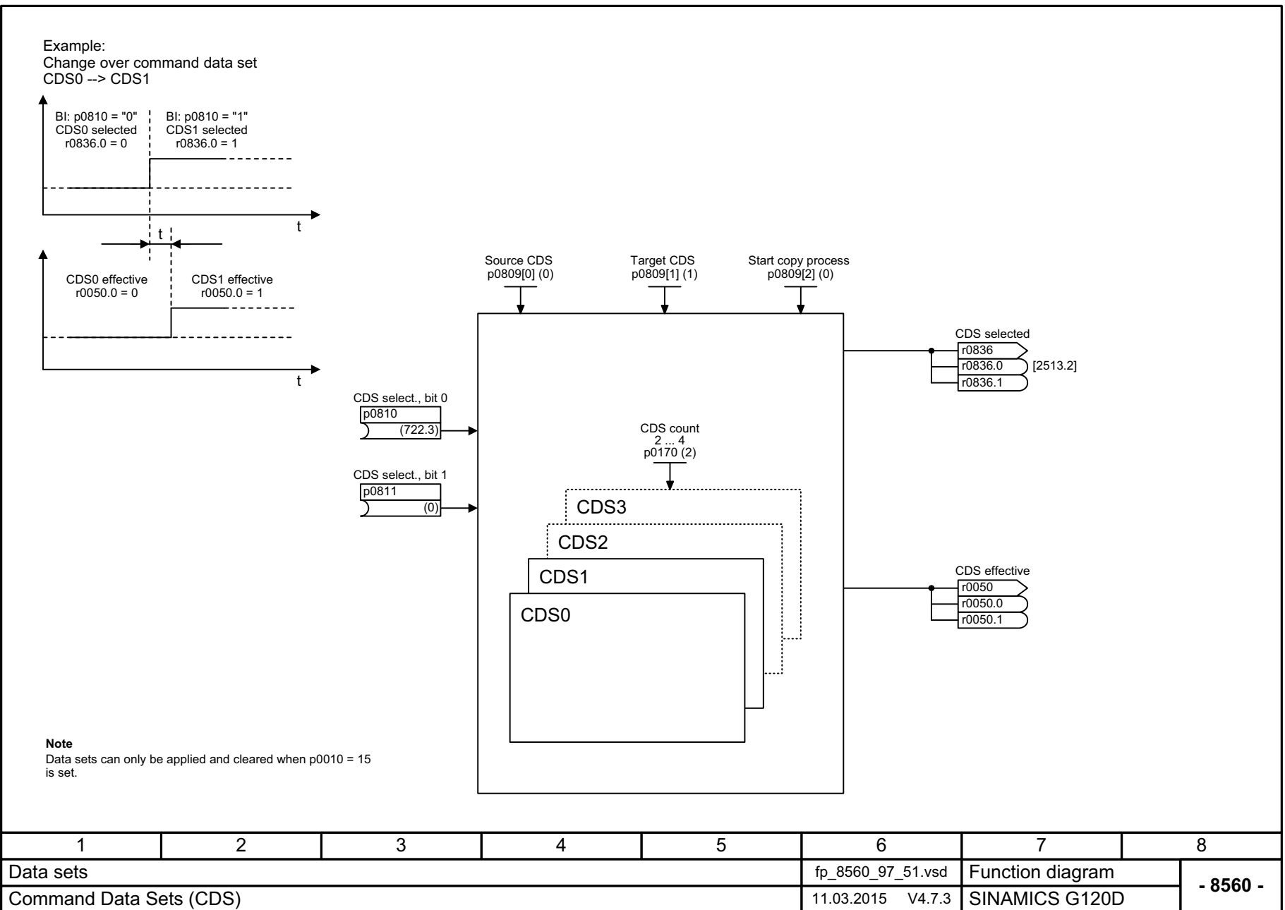
Fig. 3-174 8560 – Command Data Sets (CDS)
