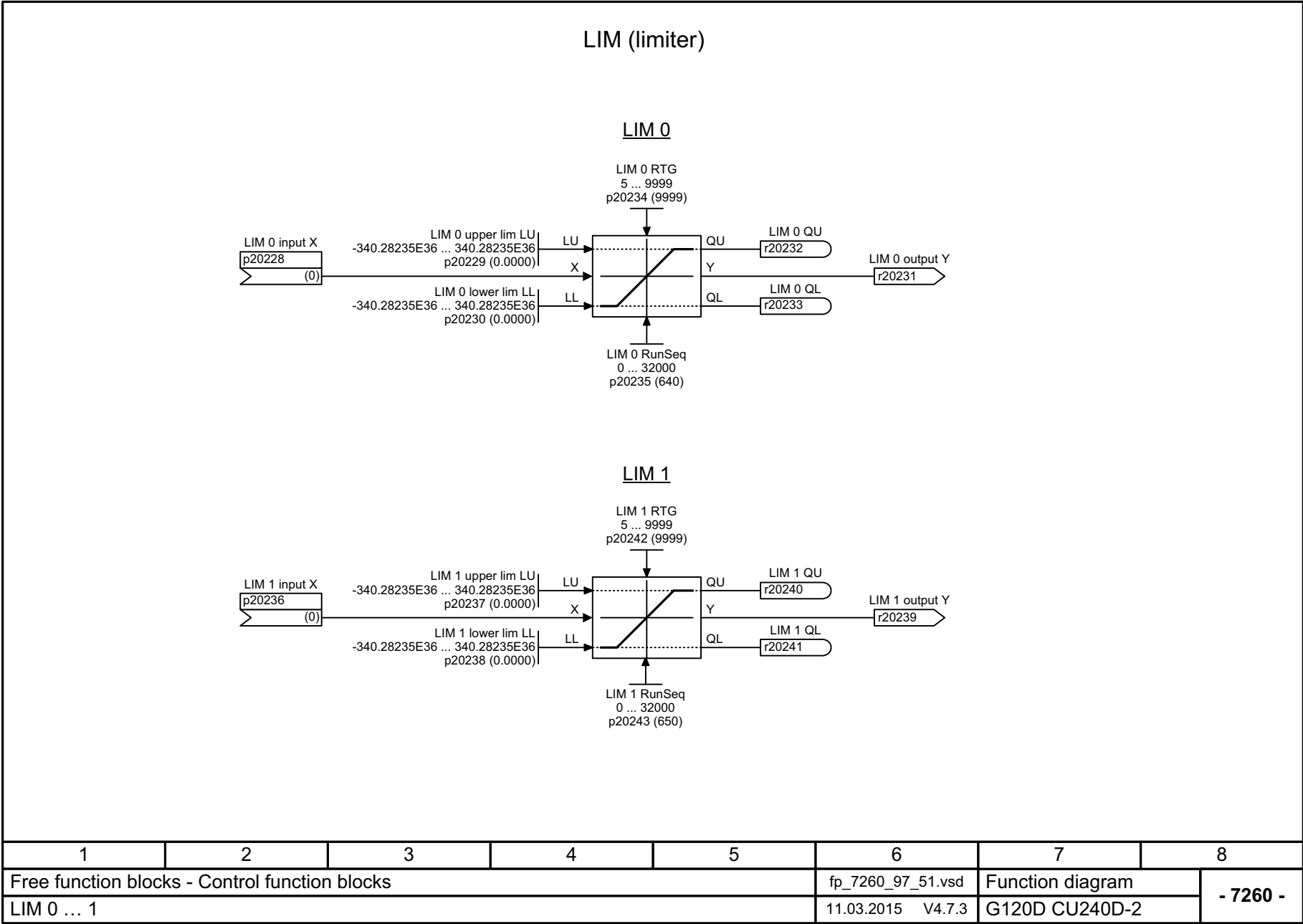
Fig. 3-151 7260 – LIM 0 ... 1
