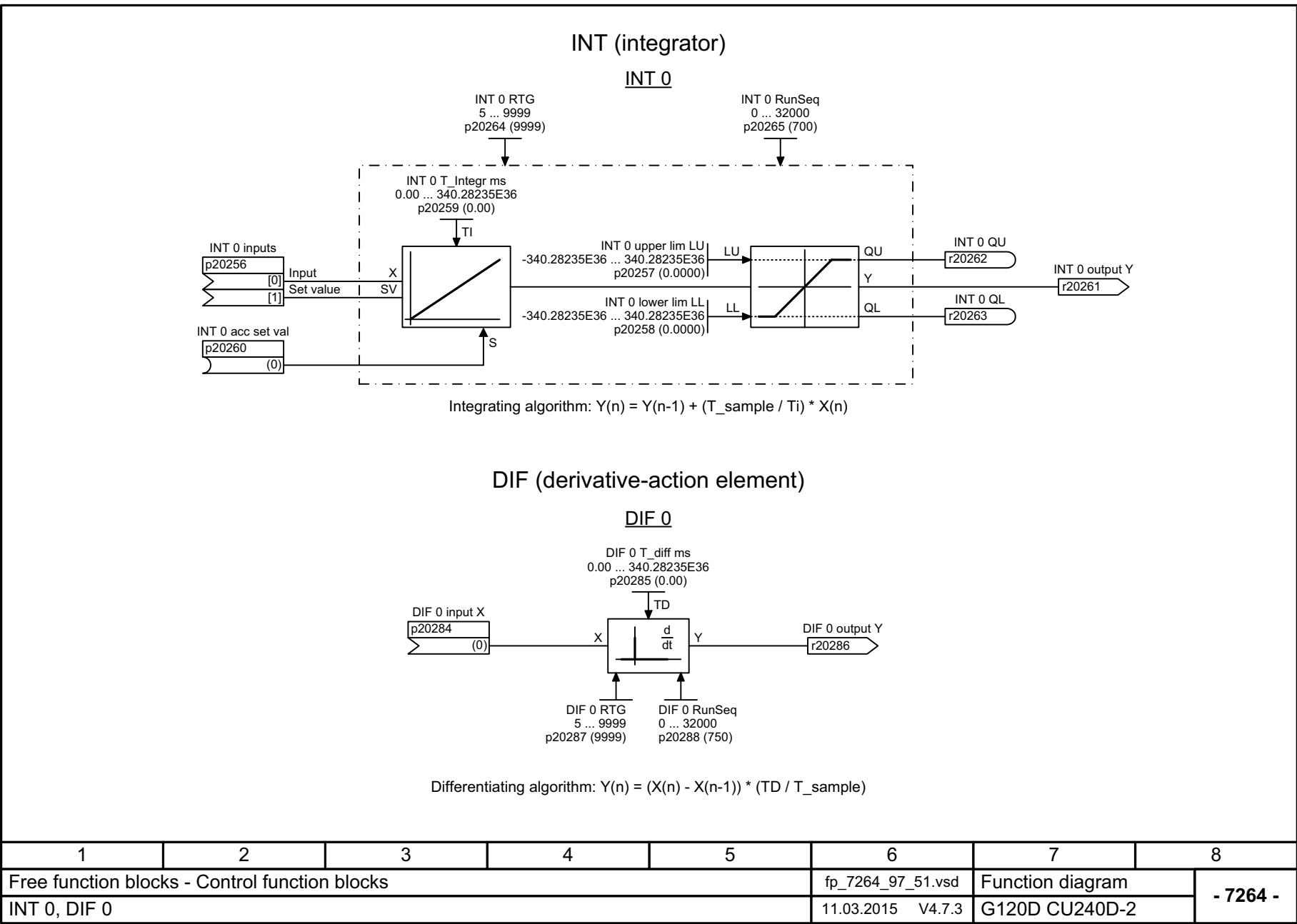
Fig. 3-153 7264 – INT 0, DIF 0
