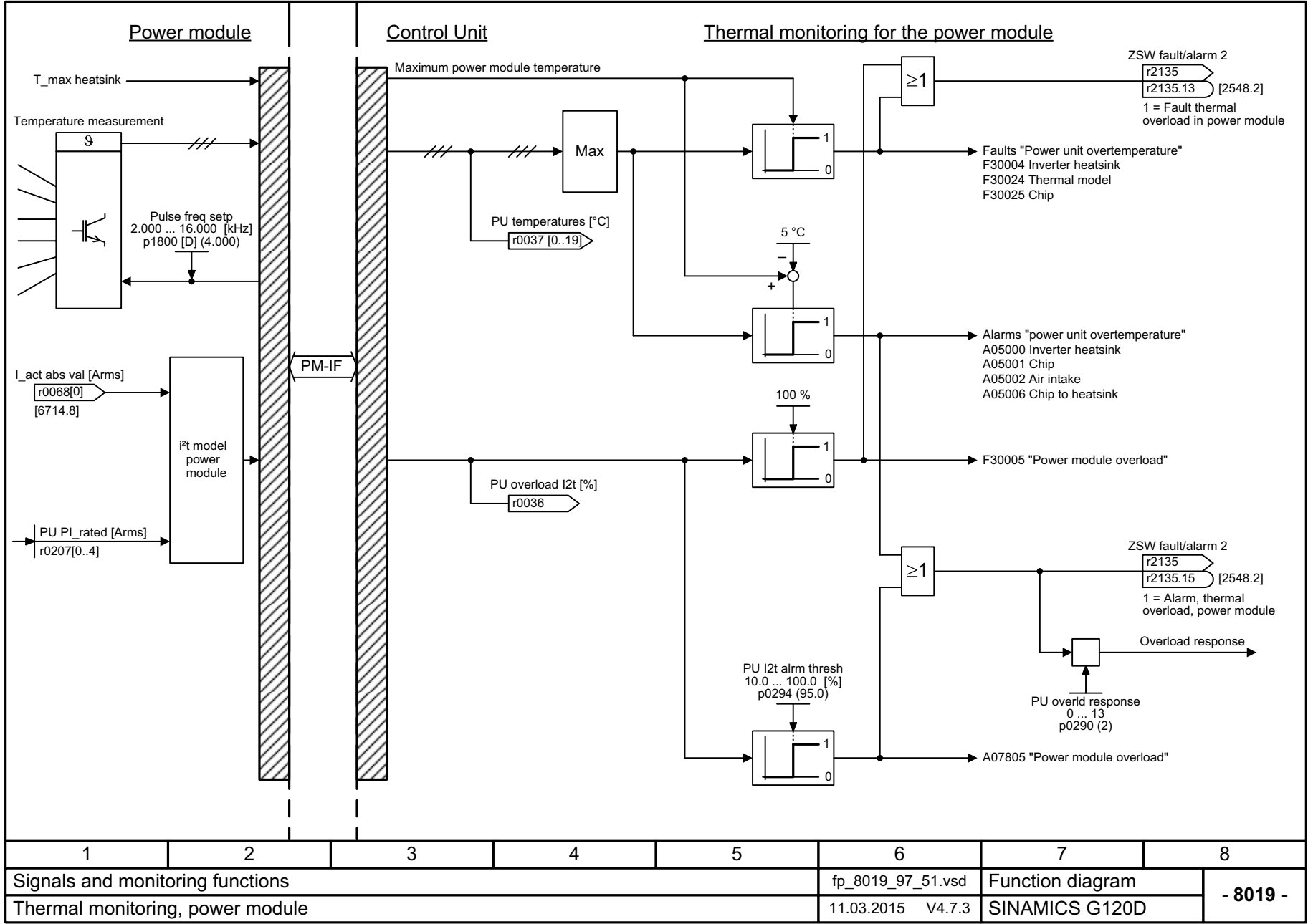
Fig. 3-166 8019 – Thermal monitoring, power unit
