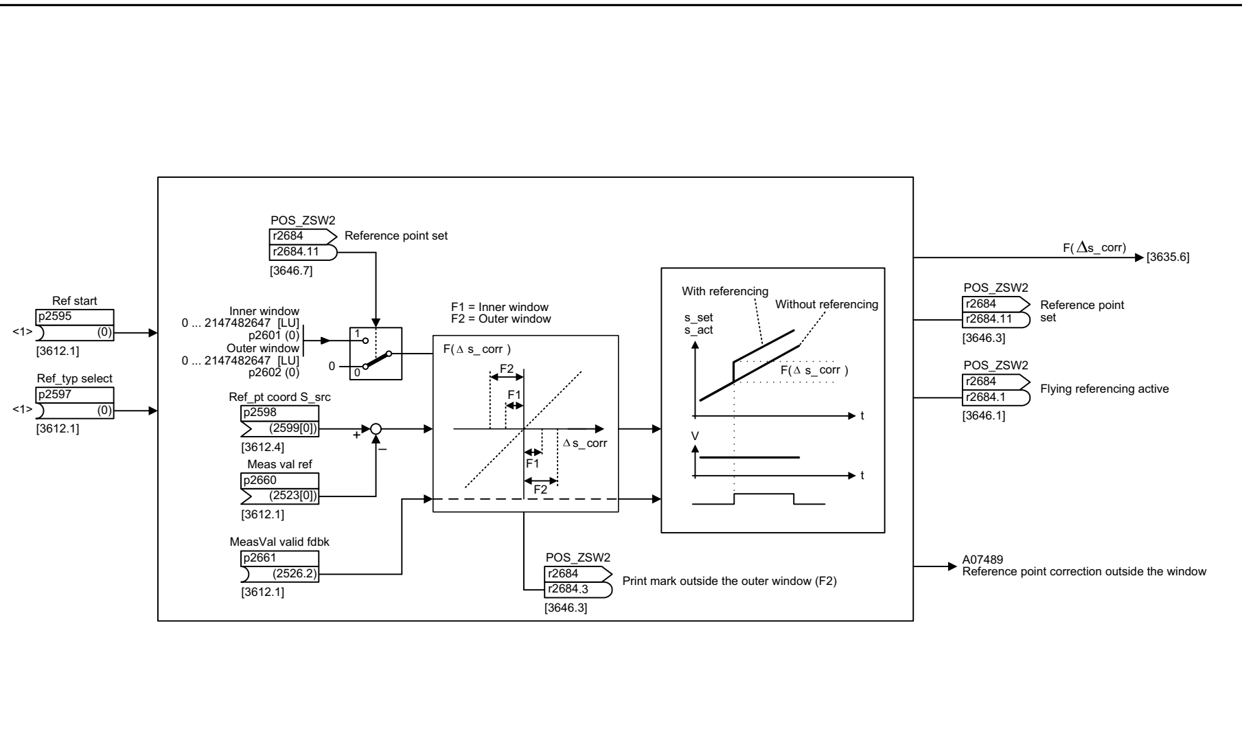
Fig. 3-87 3614 – Flying referencing mode (p2597 = 1 signal)
