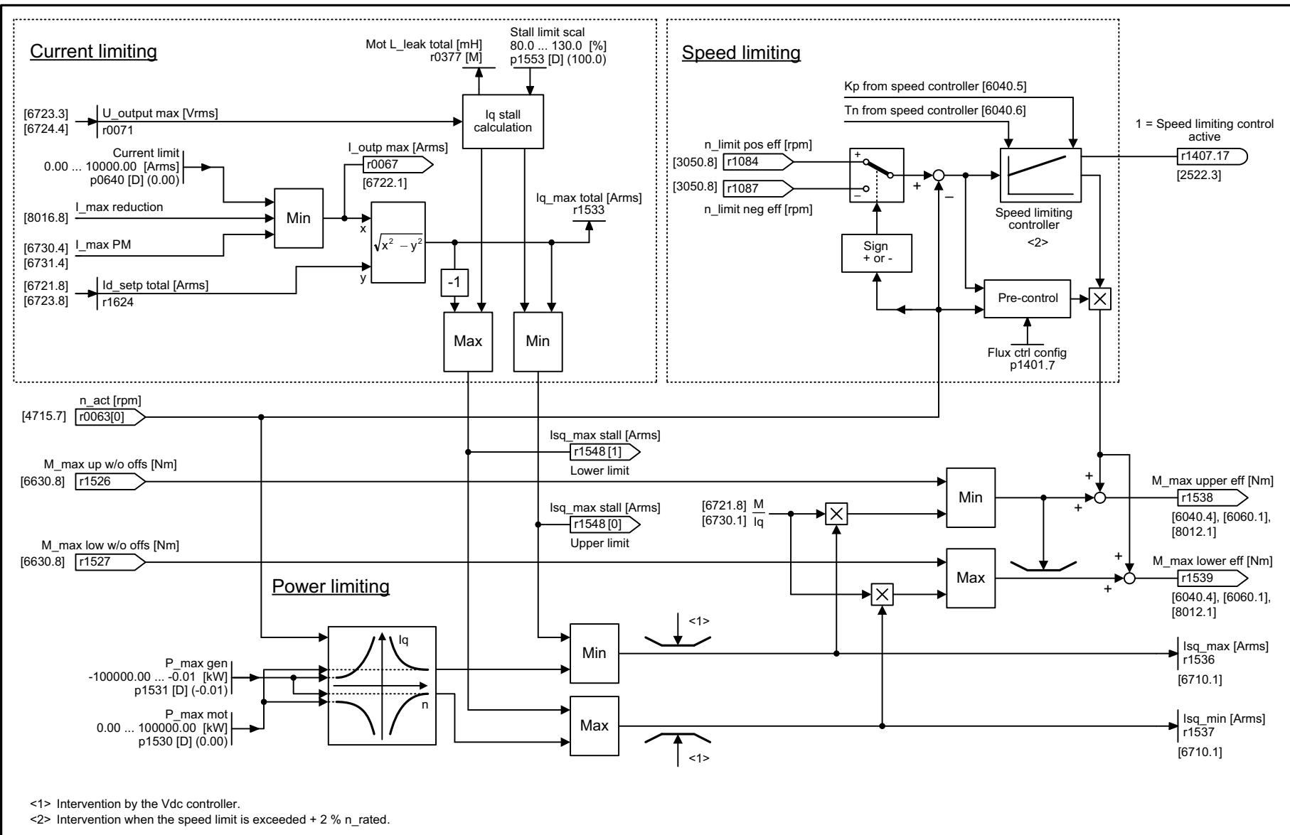
Fig. 3-123 6640 – Current/power/torque limits
