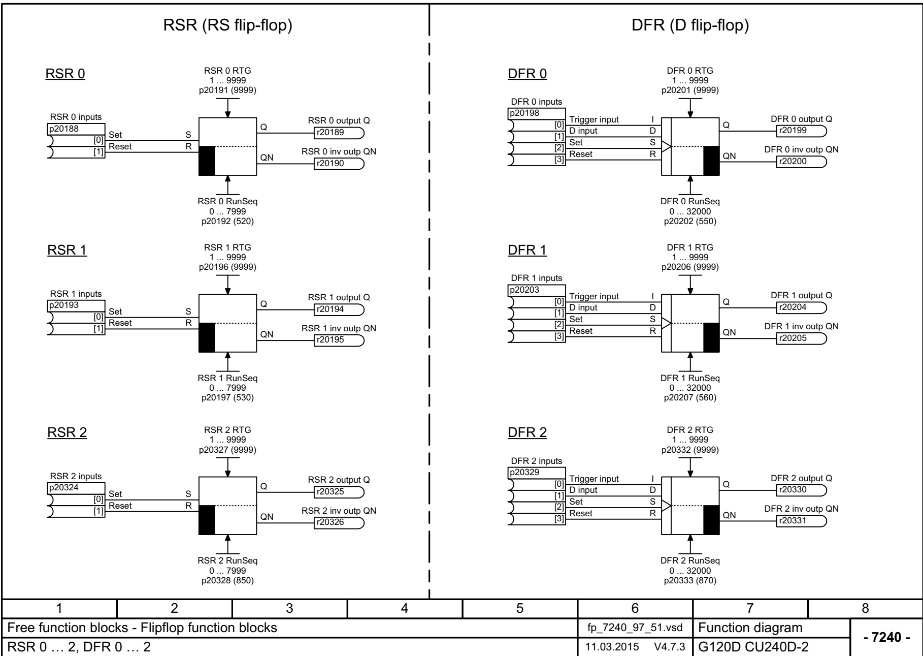
Fig. 3-149 7240 – RSR 0 ... 2, DFR 0 ... 2
