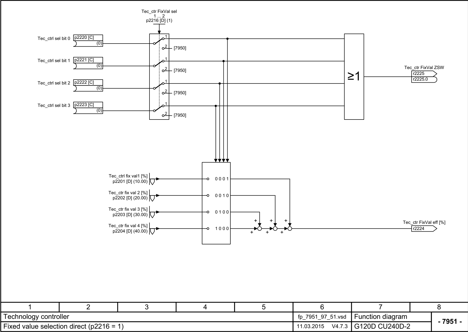
Fig. 3-156 7951 – Fixed value selection direct (p2216 = 1)
