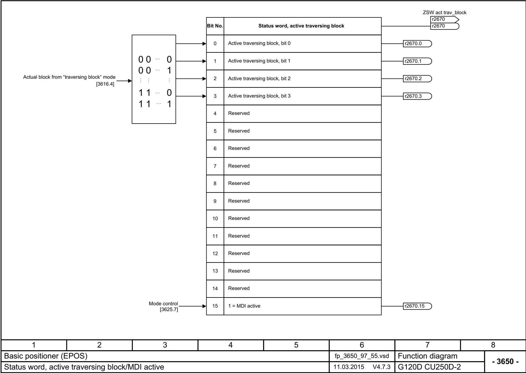
Fig. 3-99 3650 – Status word, active traversing block/MDI active
