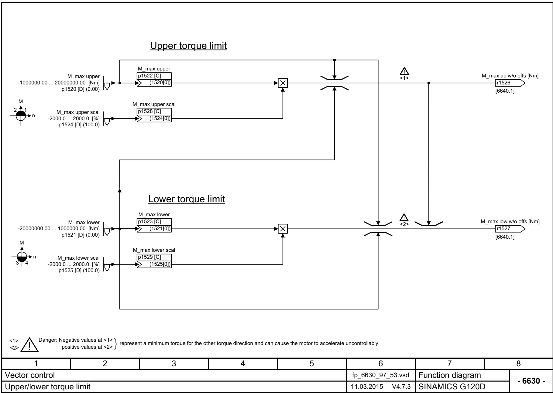
Fig. 3-122 6630 – Upper/lower torque limit
