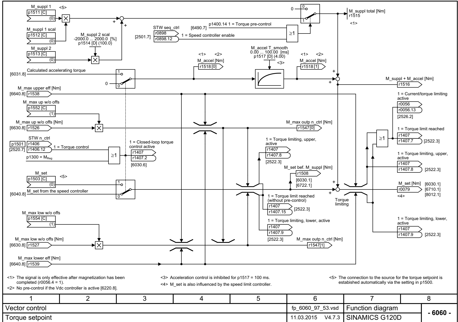
Fig. 3-116 6060 – Torque setpoint
