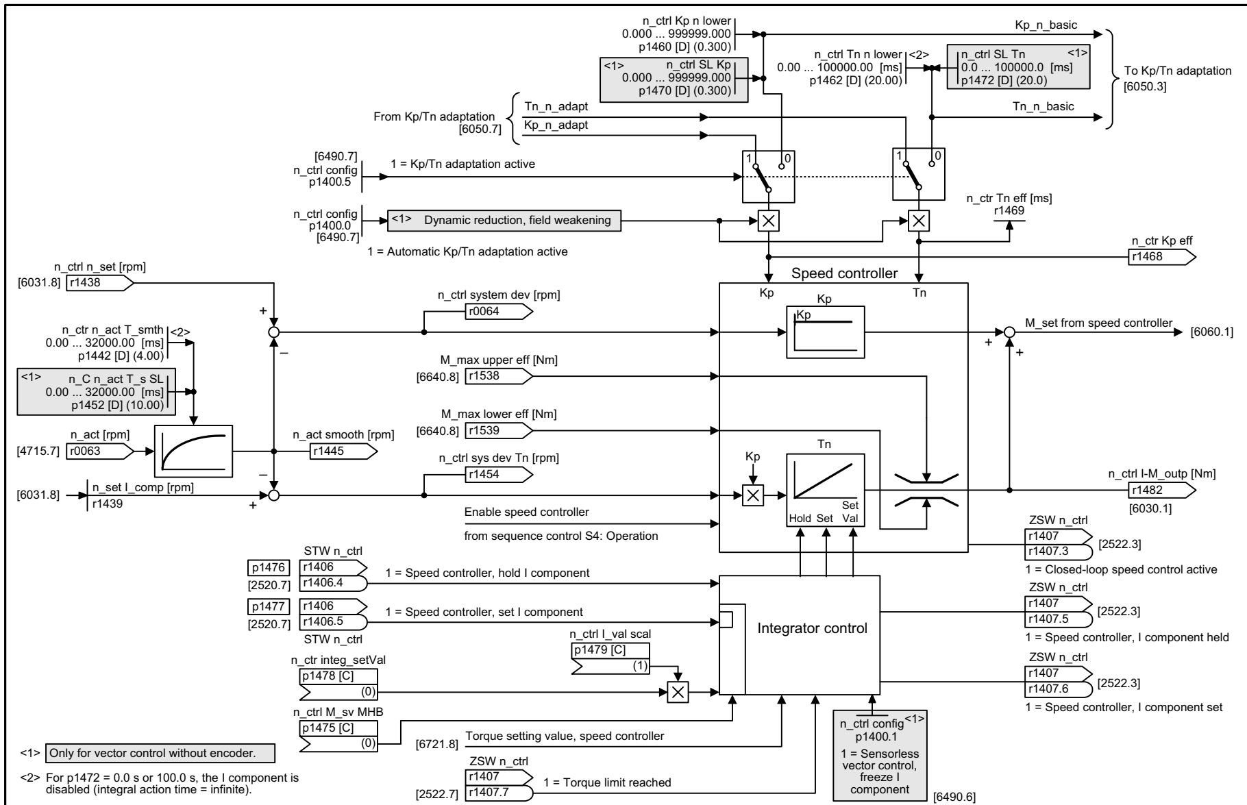
Fig. 3-114 6040 – Speed controller
