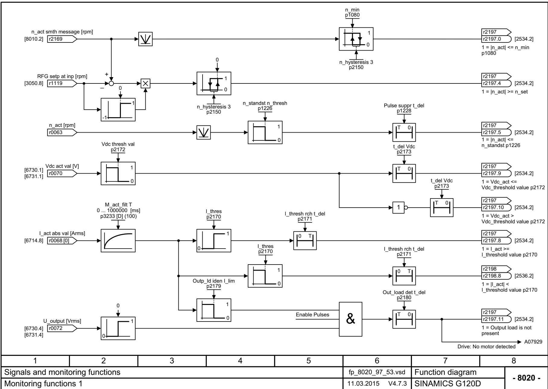
Fig. 3-167 8020 – Monitoring functions 1
