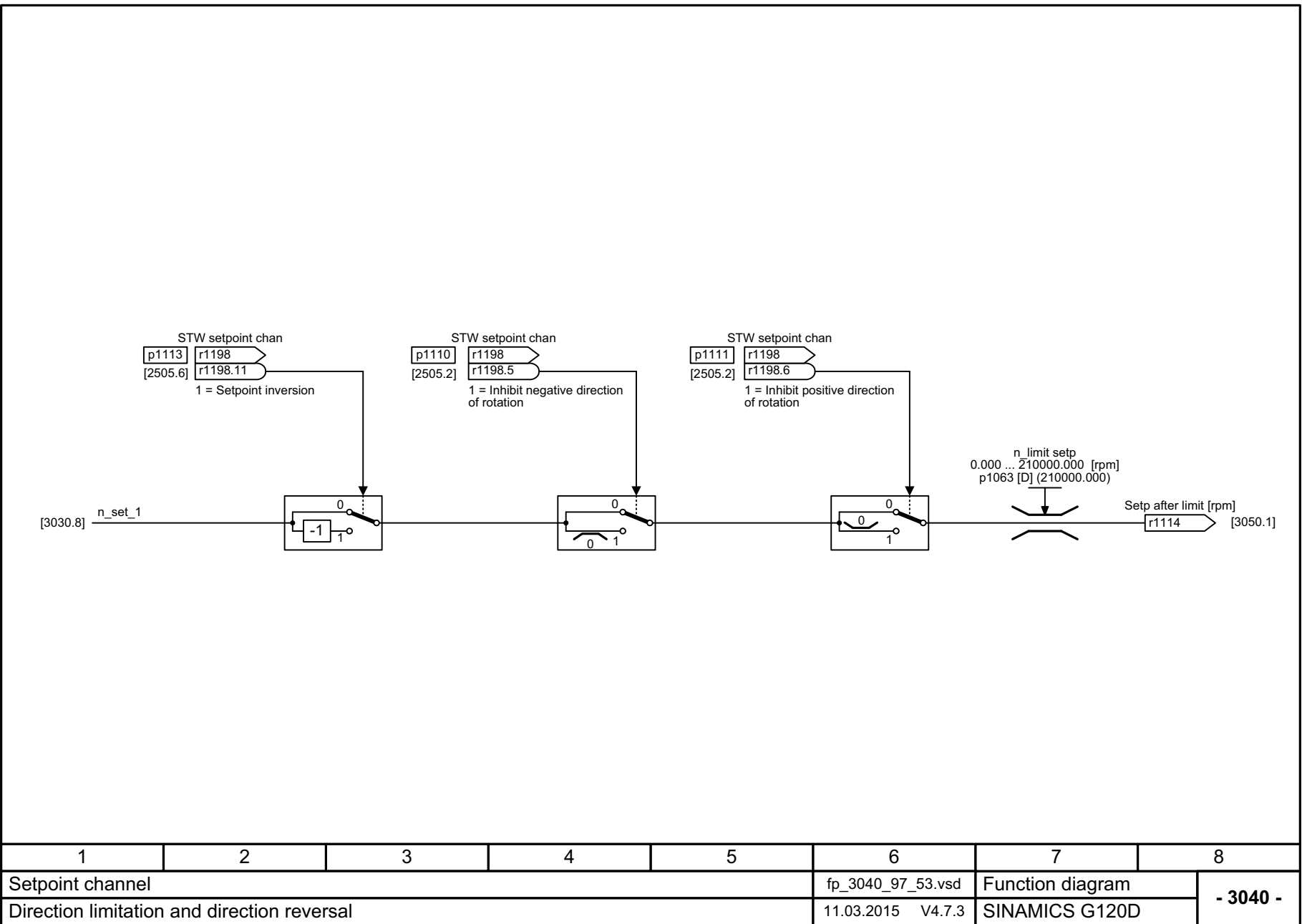
Fig. 3-80 3040 – Direction limitation and direction reversal
