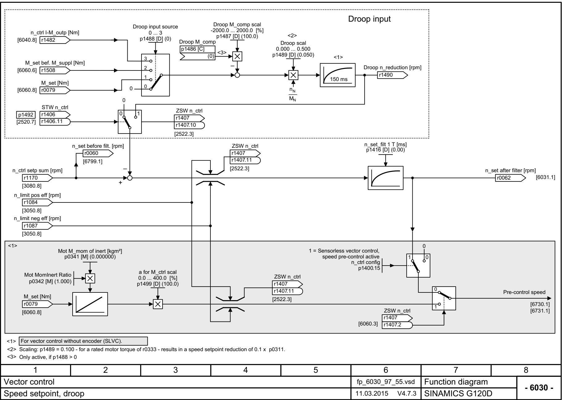
Fig. 3-111 6030 – Speed setpoint, droop
