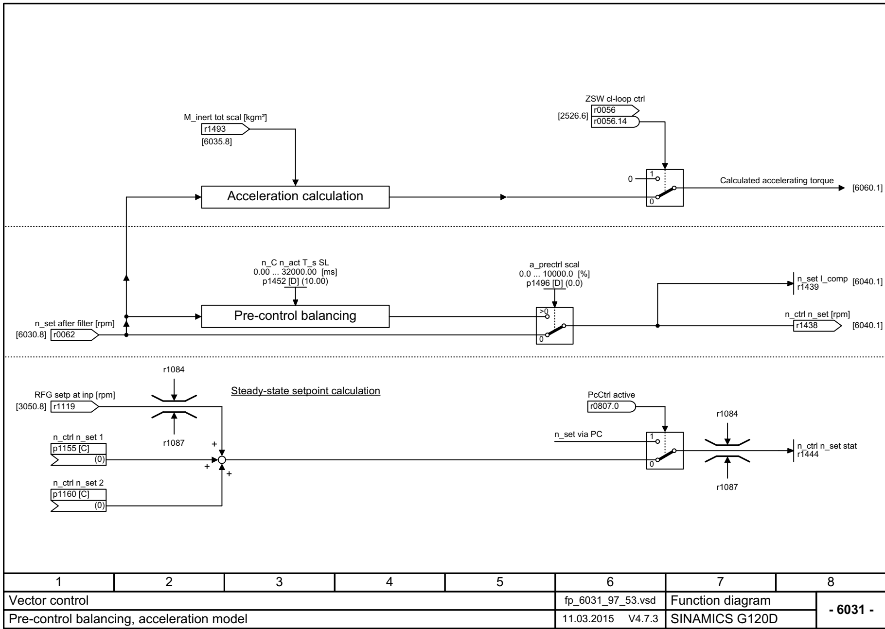
Fig. 3-112 6031 – Pre-control balancing, acceleration model
