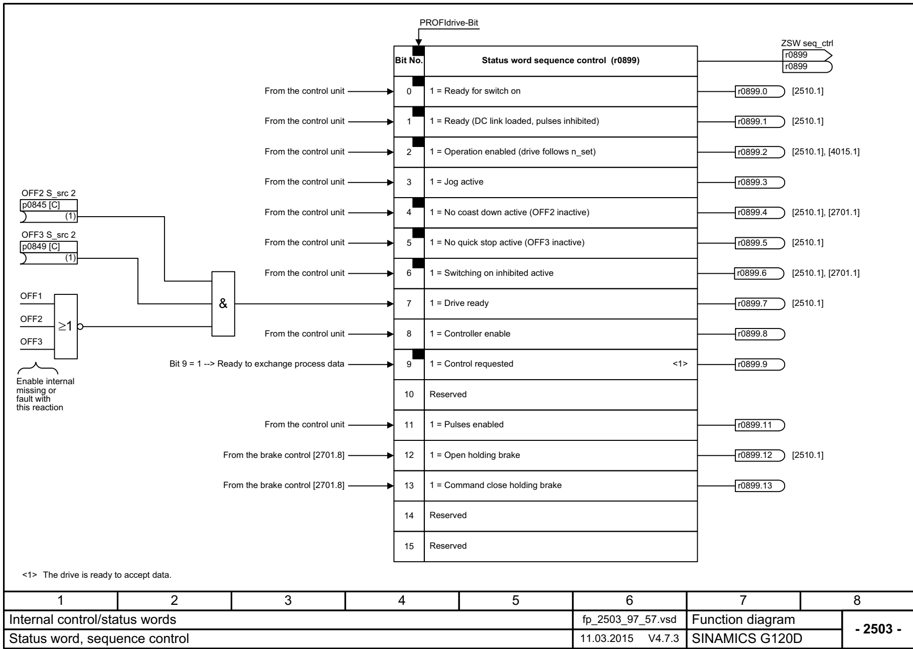
Fig. 3-39 2503 – Status word, sequence control
