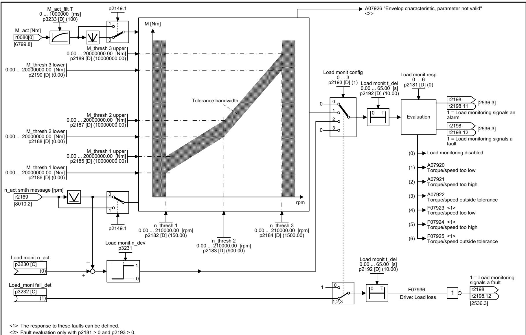
Fig. 3-163 8013 – Load monitoring
