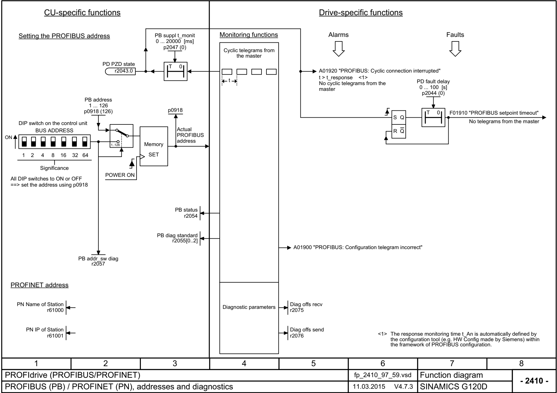
Fig. 3-13 2410 – PROFIBUS (PB) / PROFINET (PN), addresses and diagnostics
