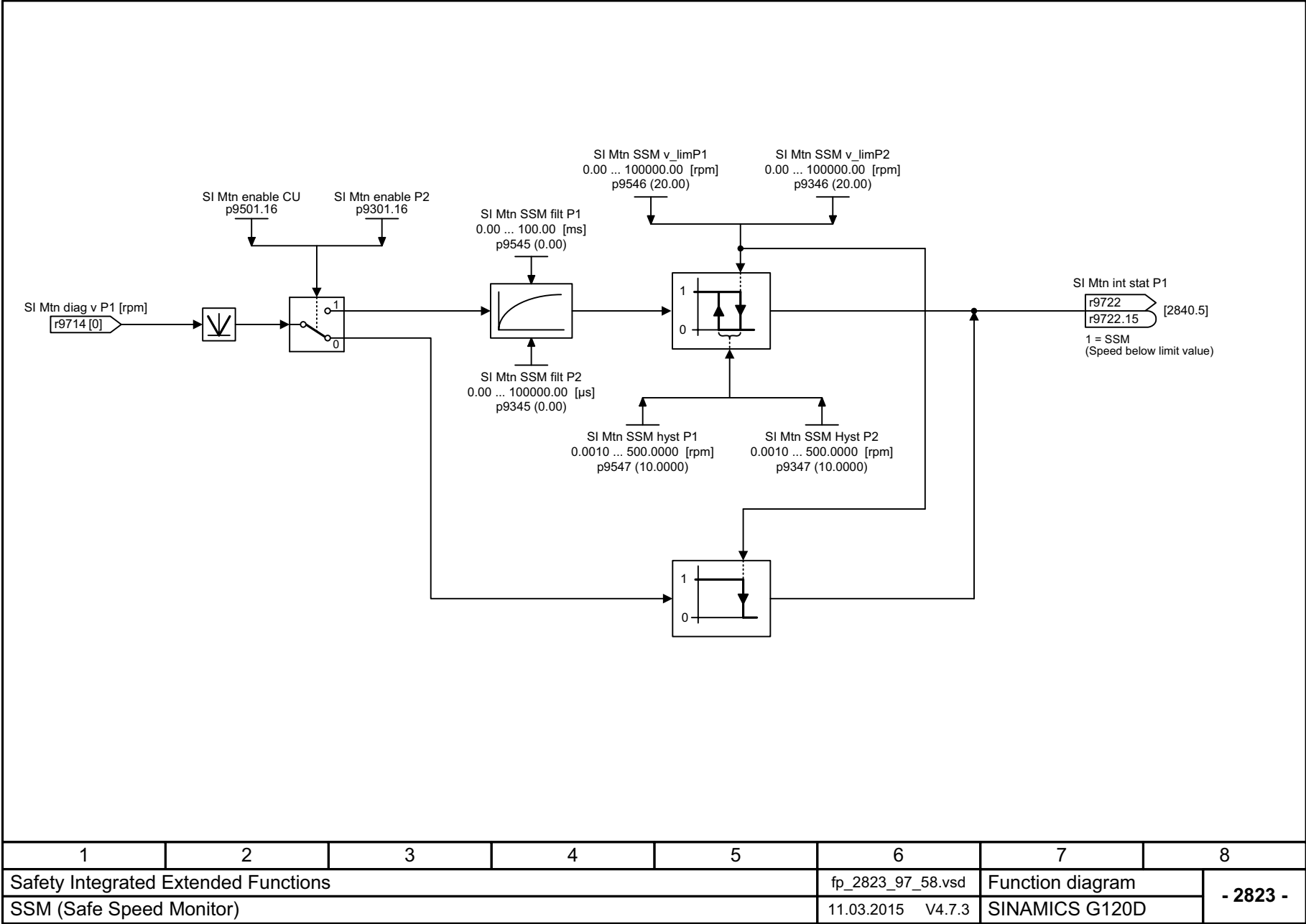
Fig. 3-64 2823 – SSM (Safe Speed Monitor)
