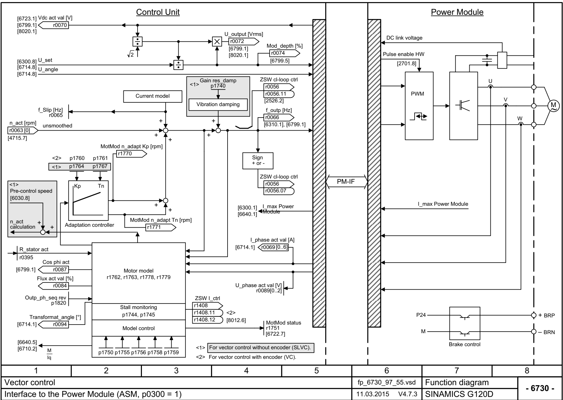
Fig. 3-131 6730 – Interface to the Power Module (ASM, p0300 = 1)
