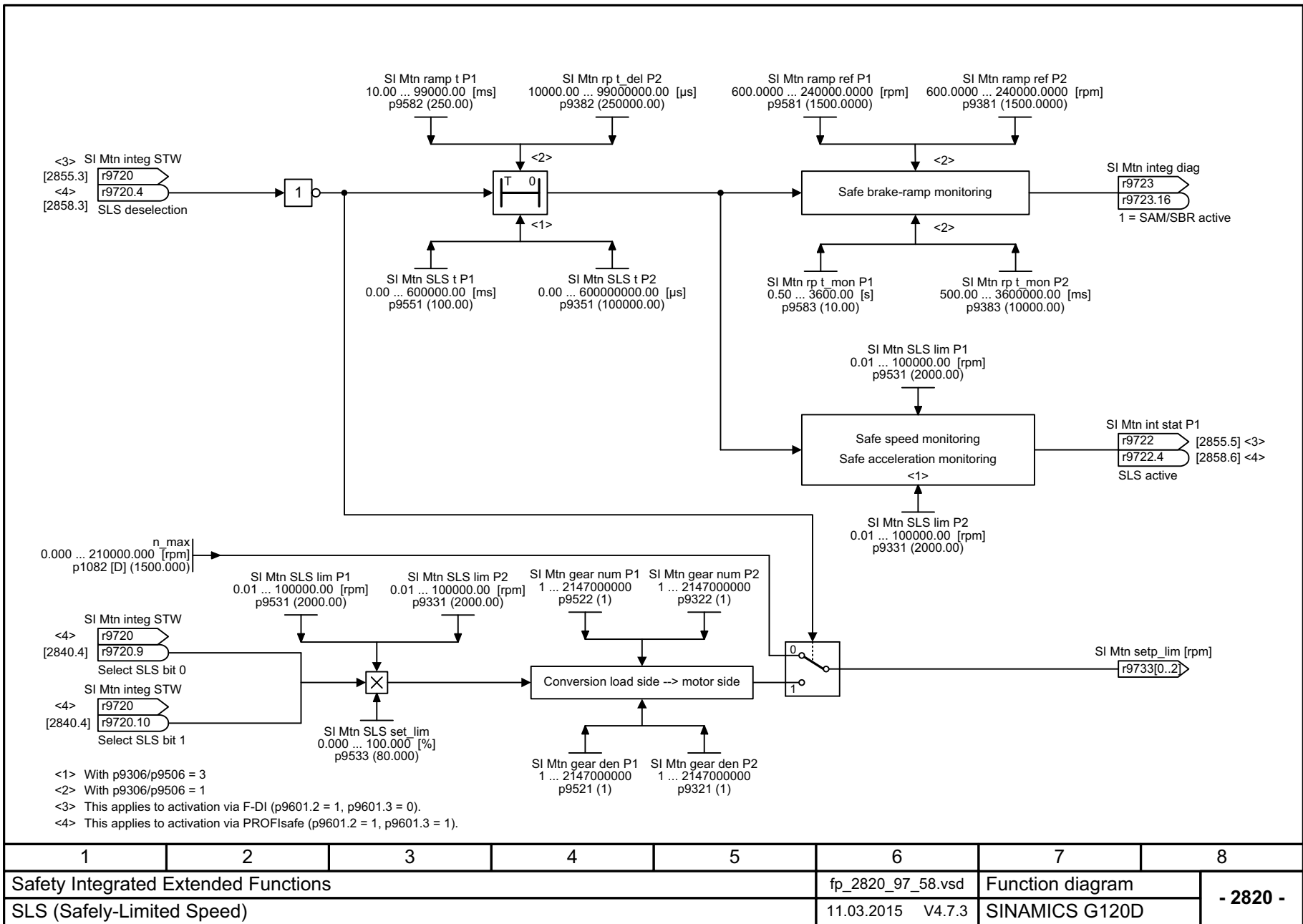
Fig. 3-63 2820 – SLS (Safely-Limited Speed)
