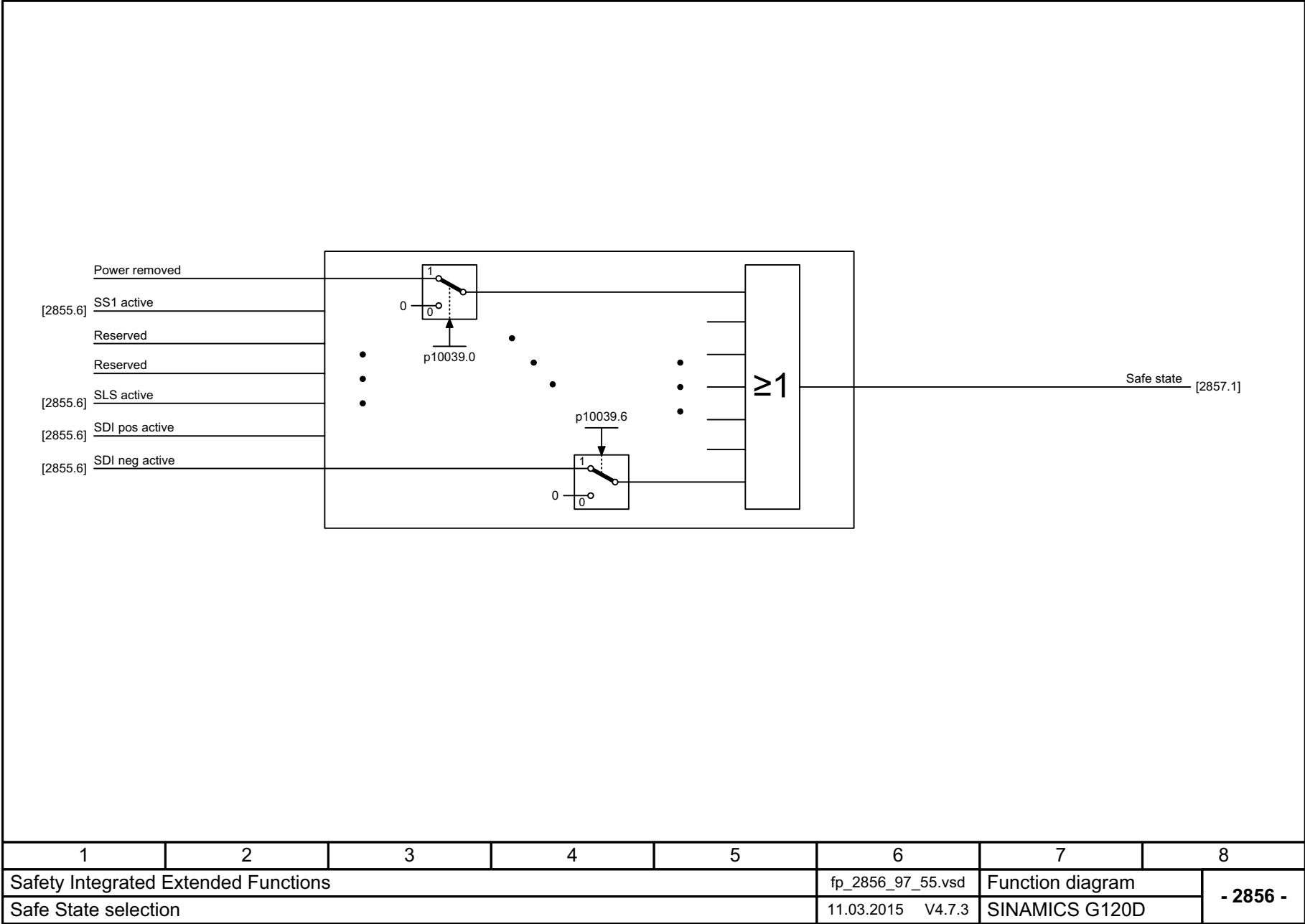
Fig. 3-70 2856 – Safe state selection
