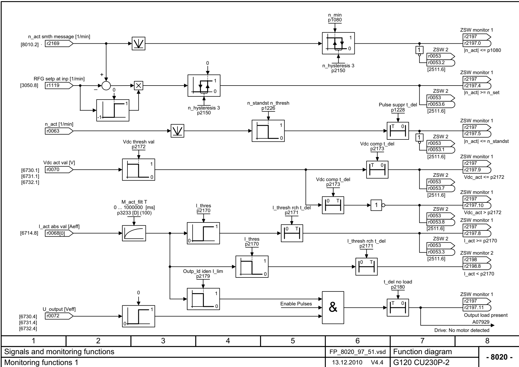
Fig. 2-130 8020 – Monitoring functions 1
