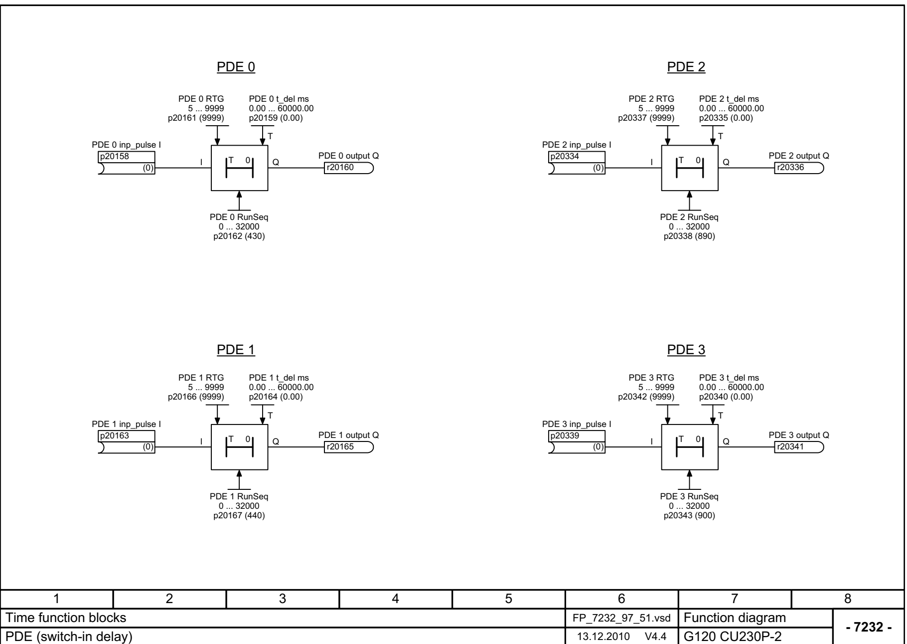
Fig. 2-103 7232 – PDE (switch-in delay)
