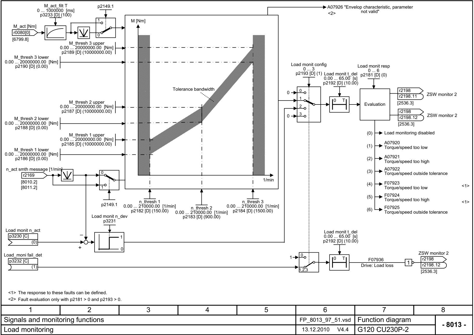
Fig. 2-126 8013 – Load monitoring
