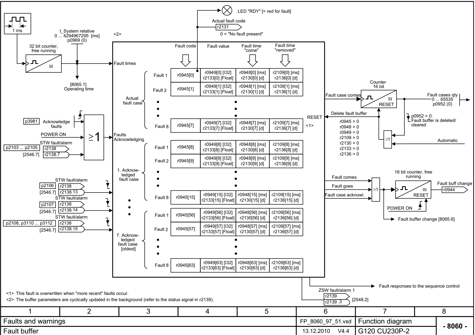
Fig. 2-132 8060 – Fault buffer
