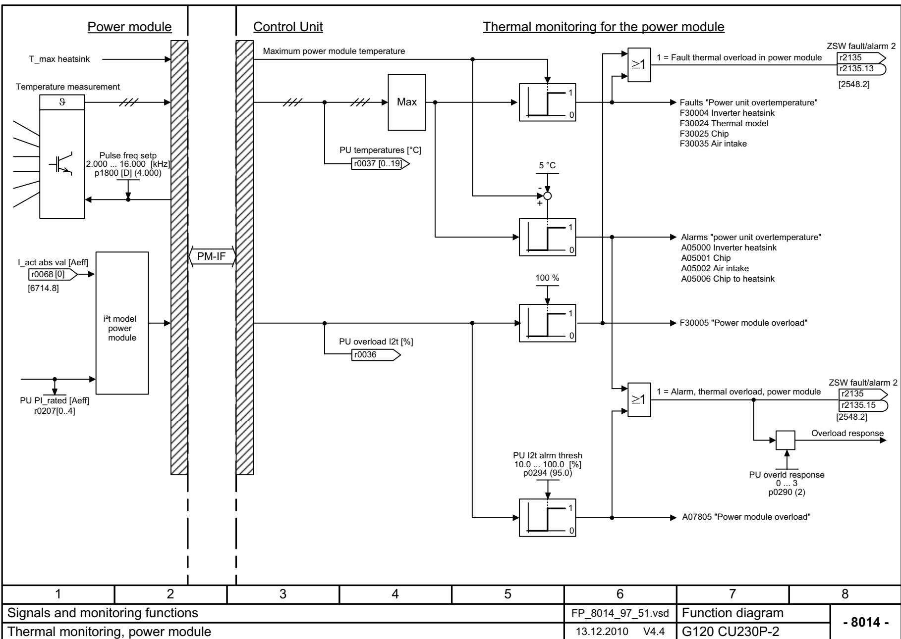
Fig. 2-127 8014 – Thermal monitoring, power module
