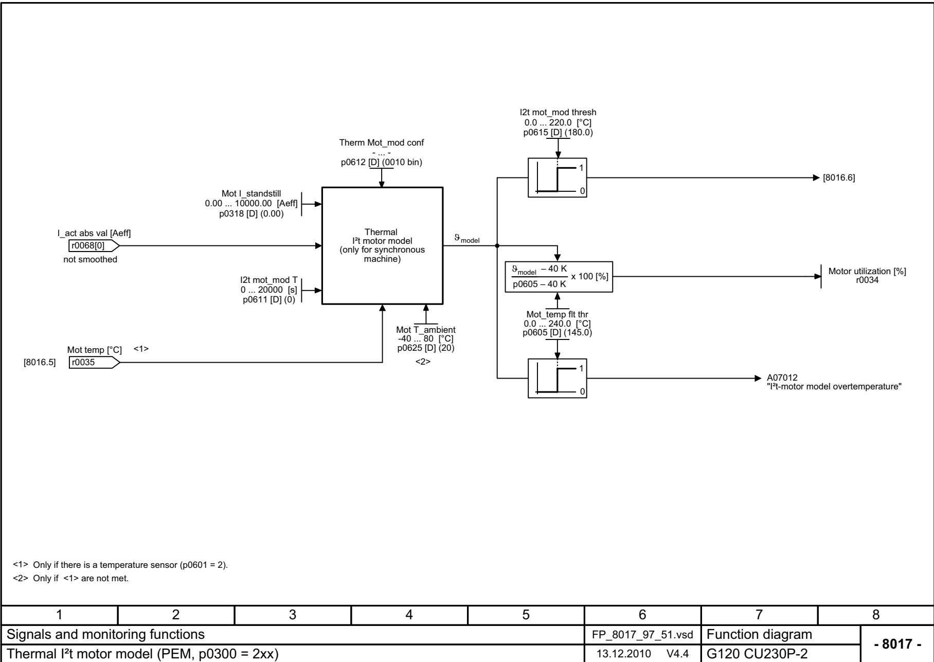
Fig. 2-129 8017 – Thermal I²t motor model (PEM, p0300 = 2xx)
