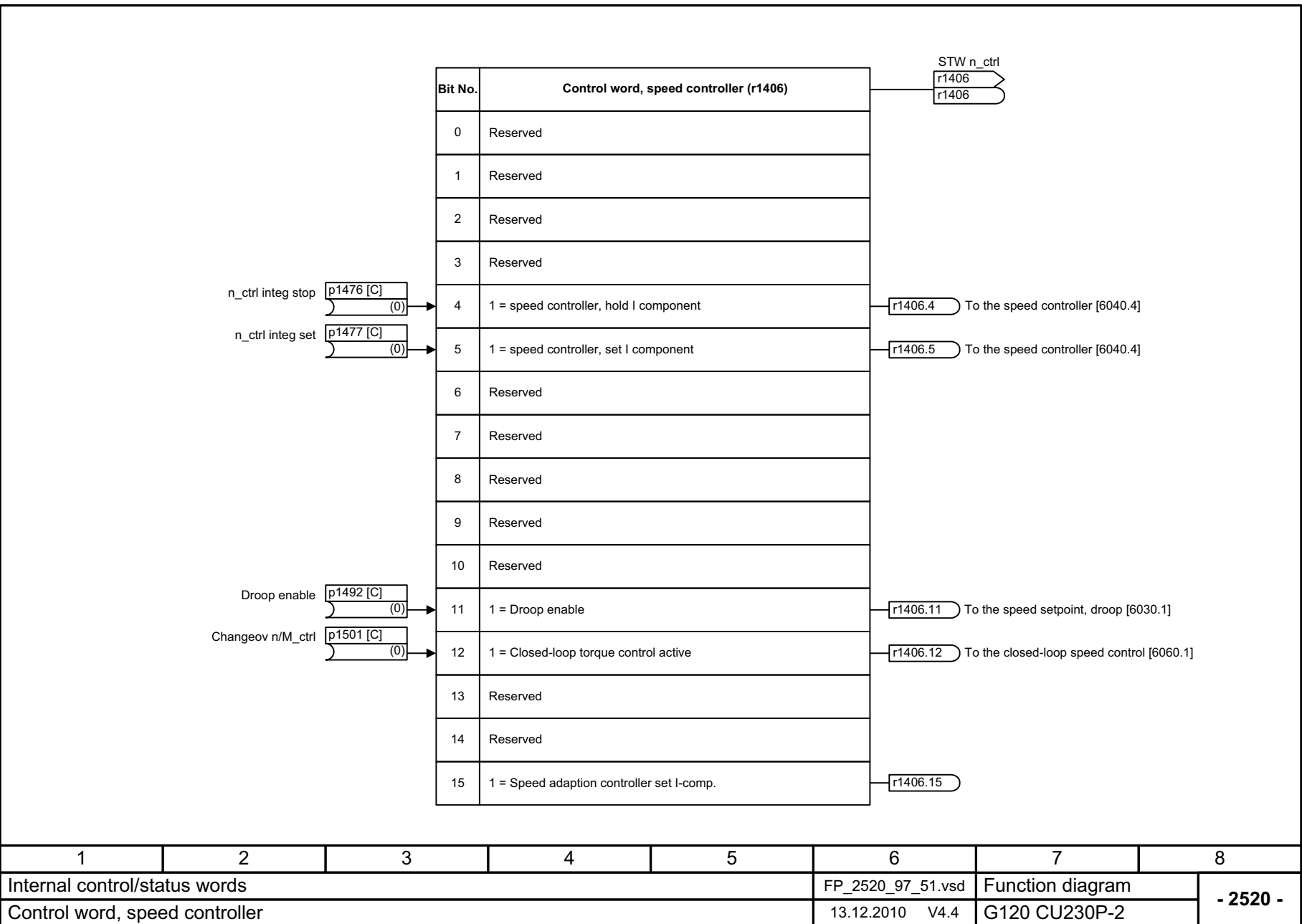
Fig. 2-51 2520 – Control word, speed controller
