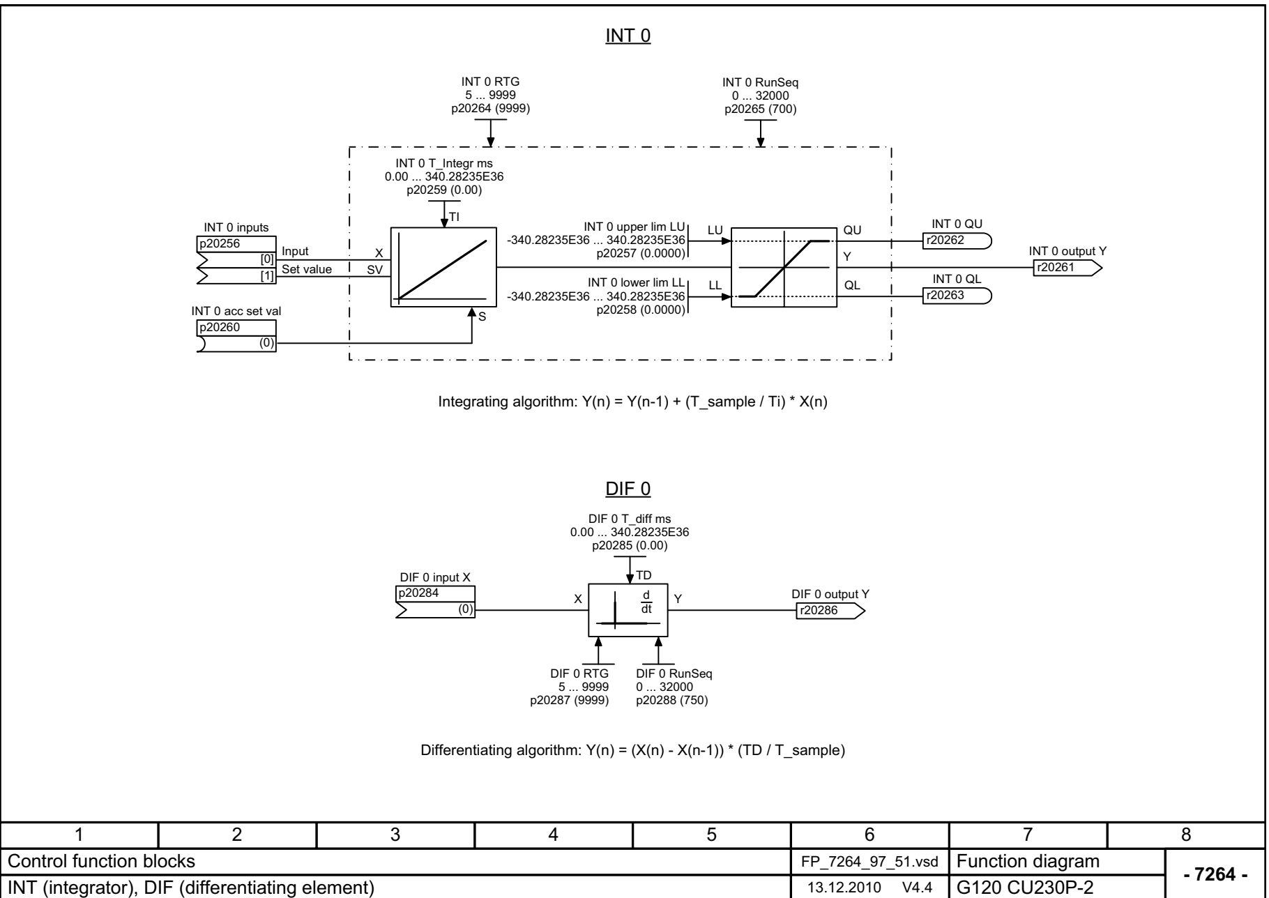
Fig. 2-110 7264 – INT (integrator), DIF (differentiating element)
