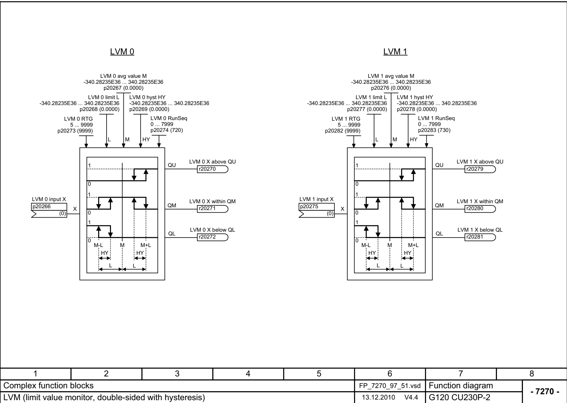
Fig. 2-111 7270 – LVM (limit value monitor, double-sided with hysteresis)
