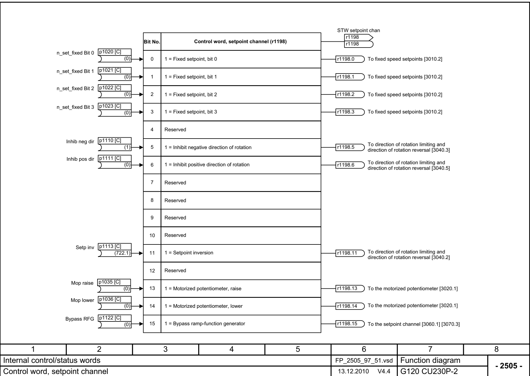
Fig. 2-46 2505 – Control word, setpoint channel
