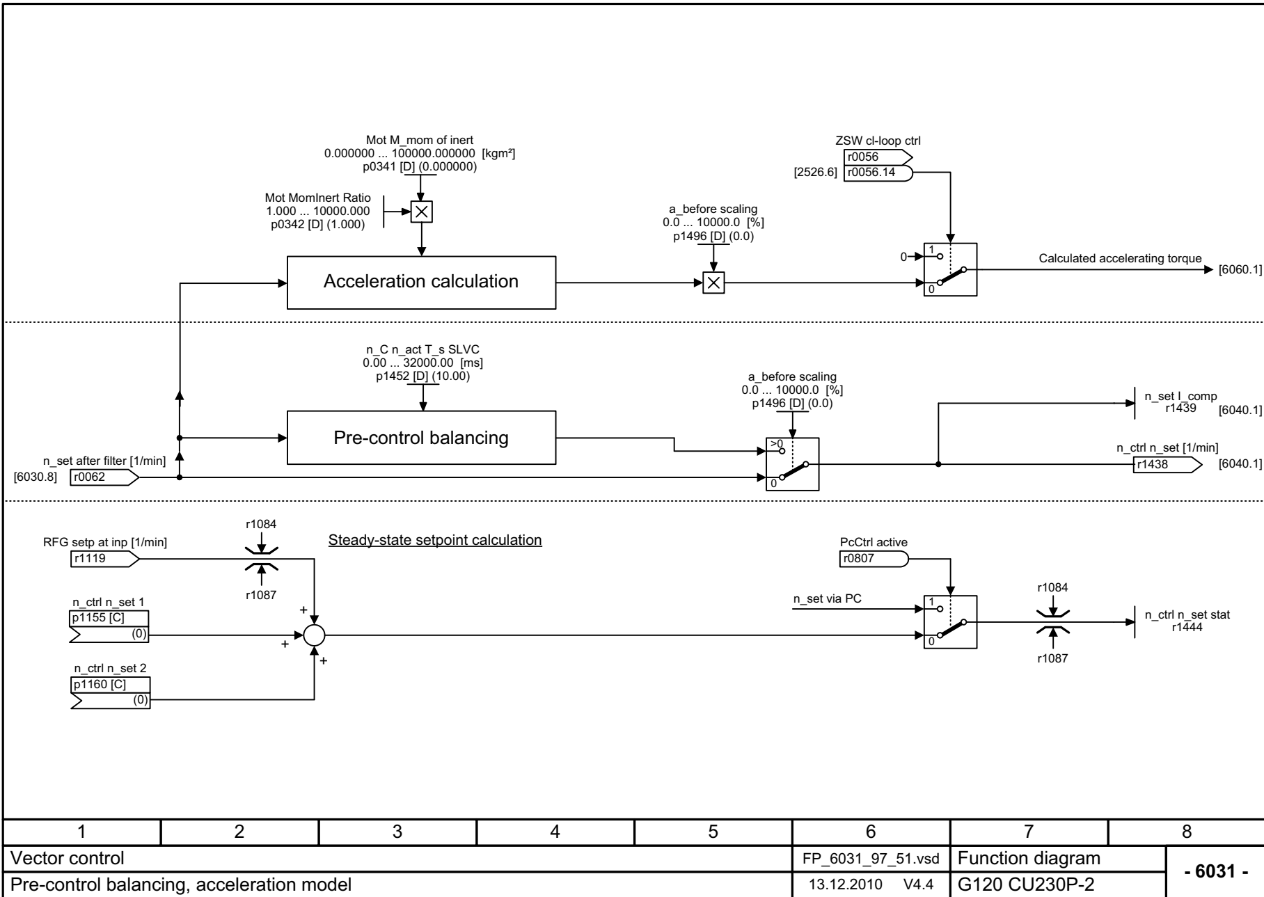
Fig. 2-74 6031 – Pre-control balancing, acceleration model
