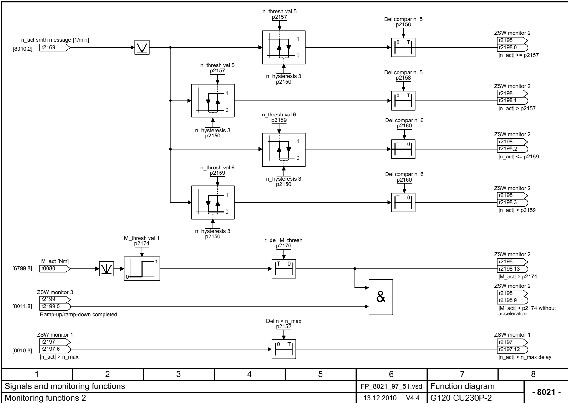
Fig. 2-131 8021 – Monitoring functions 2
