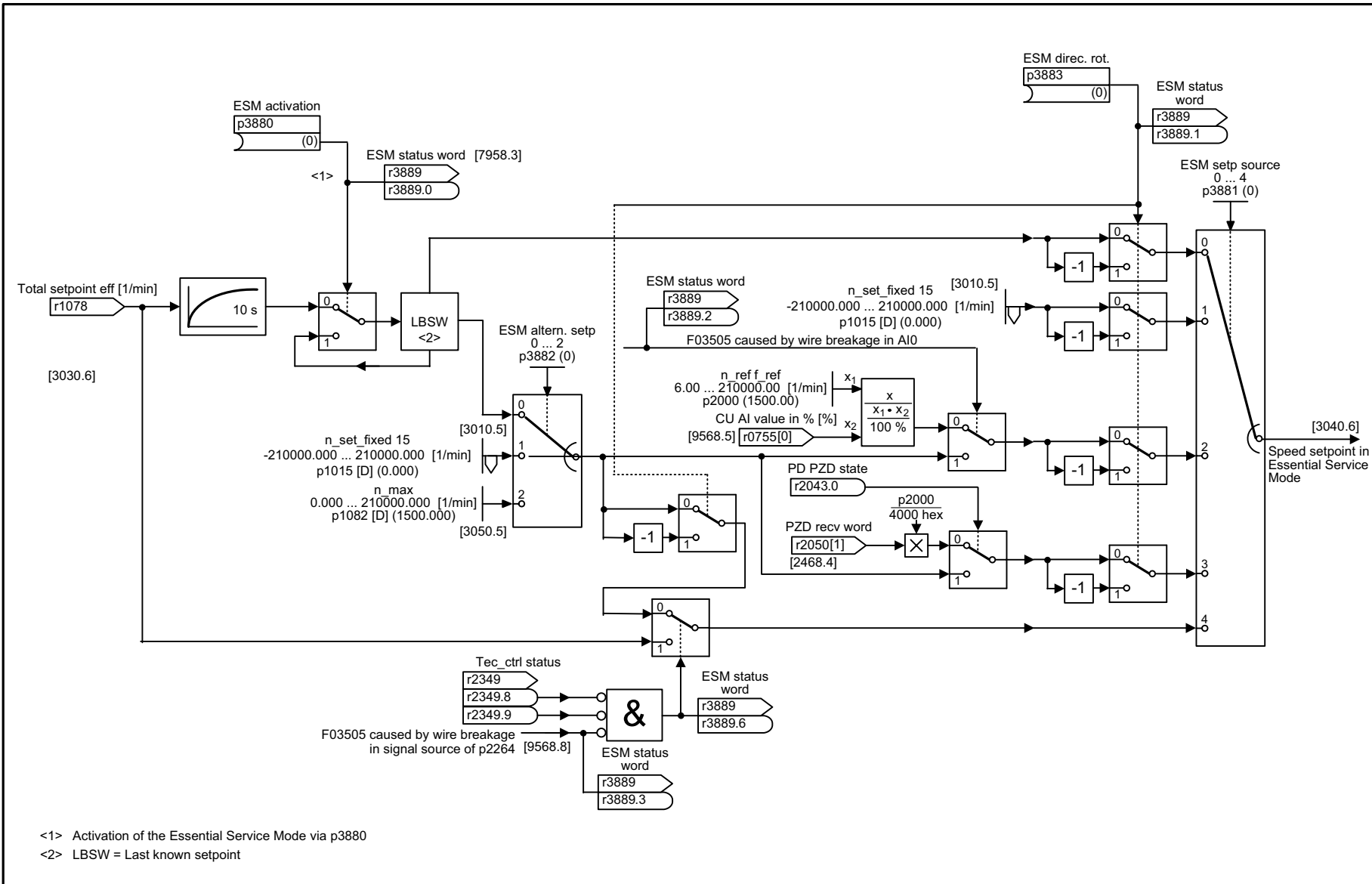
Fig. 2-115 7973 – Essential Service Mode
