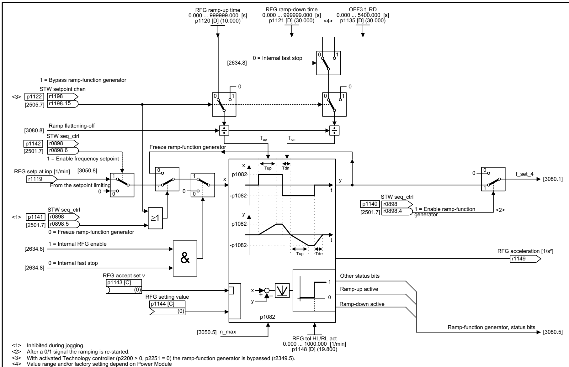
Fig. 2-67 3060 – Basic ramp-function generator
