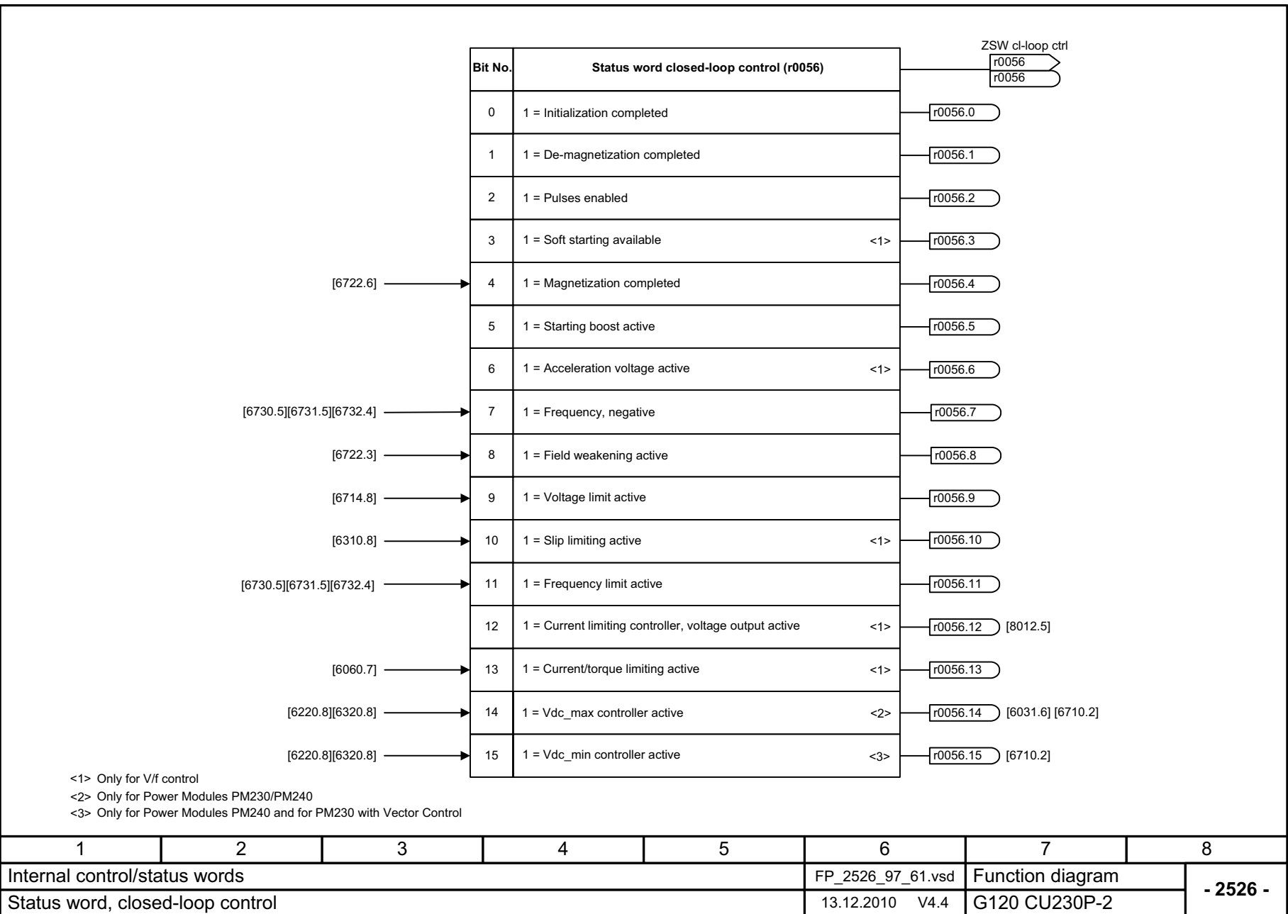
Fig. 2-53 2526 – Status word, closed-loop control
