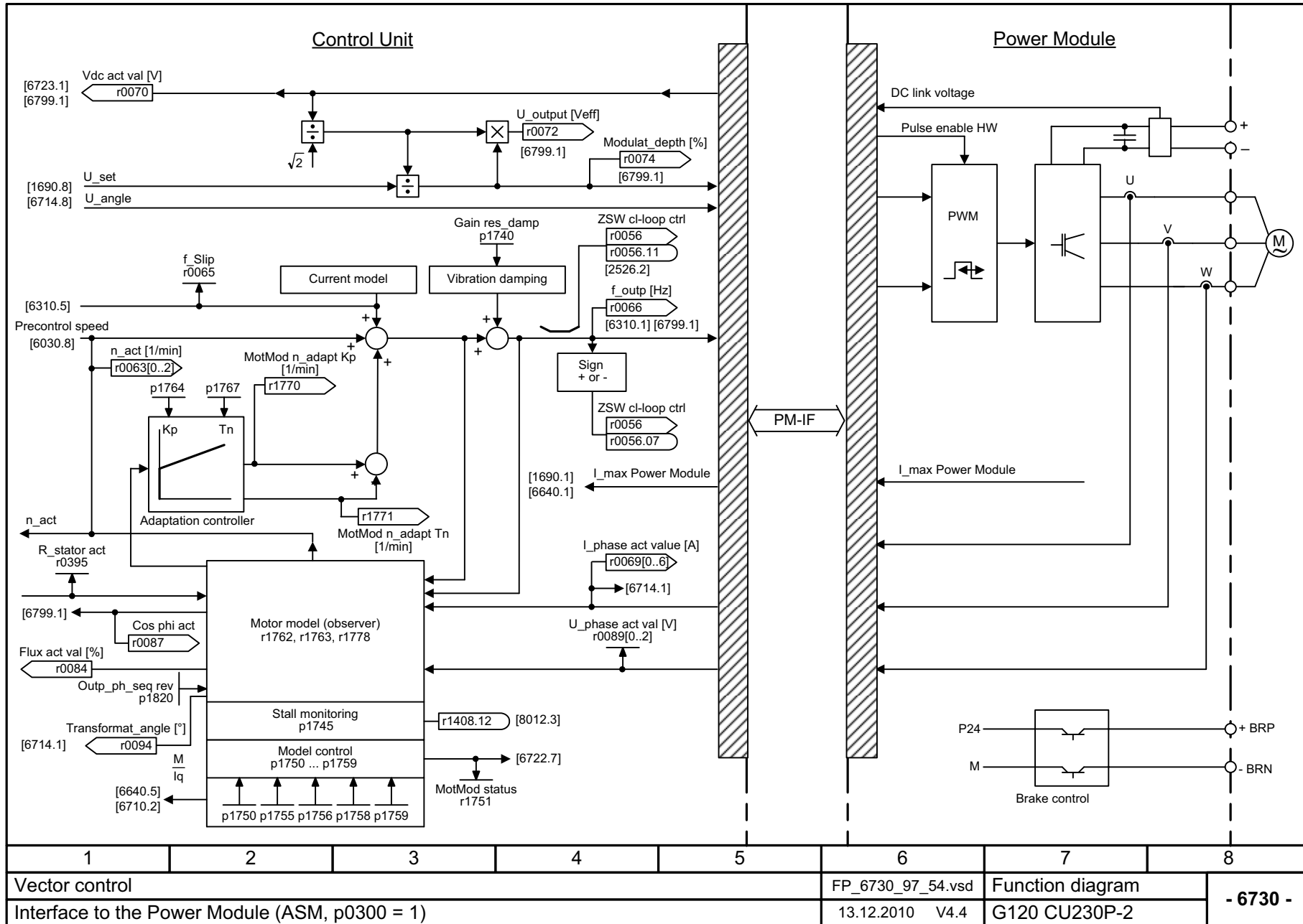
Fig. 2-89 6730 – Interface to the Power Module (ASM, p0300 = 1)
