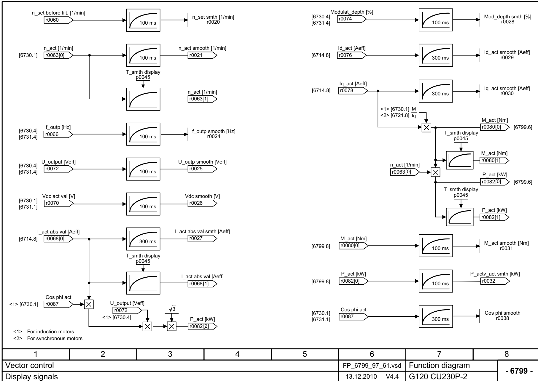
Fig. 2-91 6799 – Display signals
