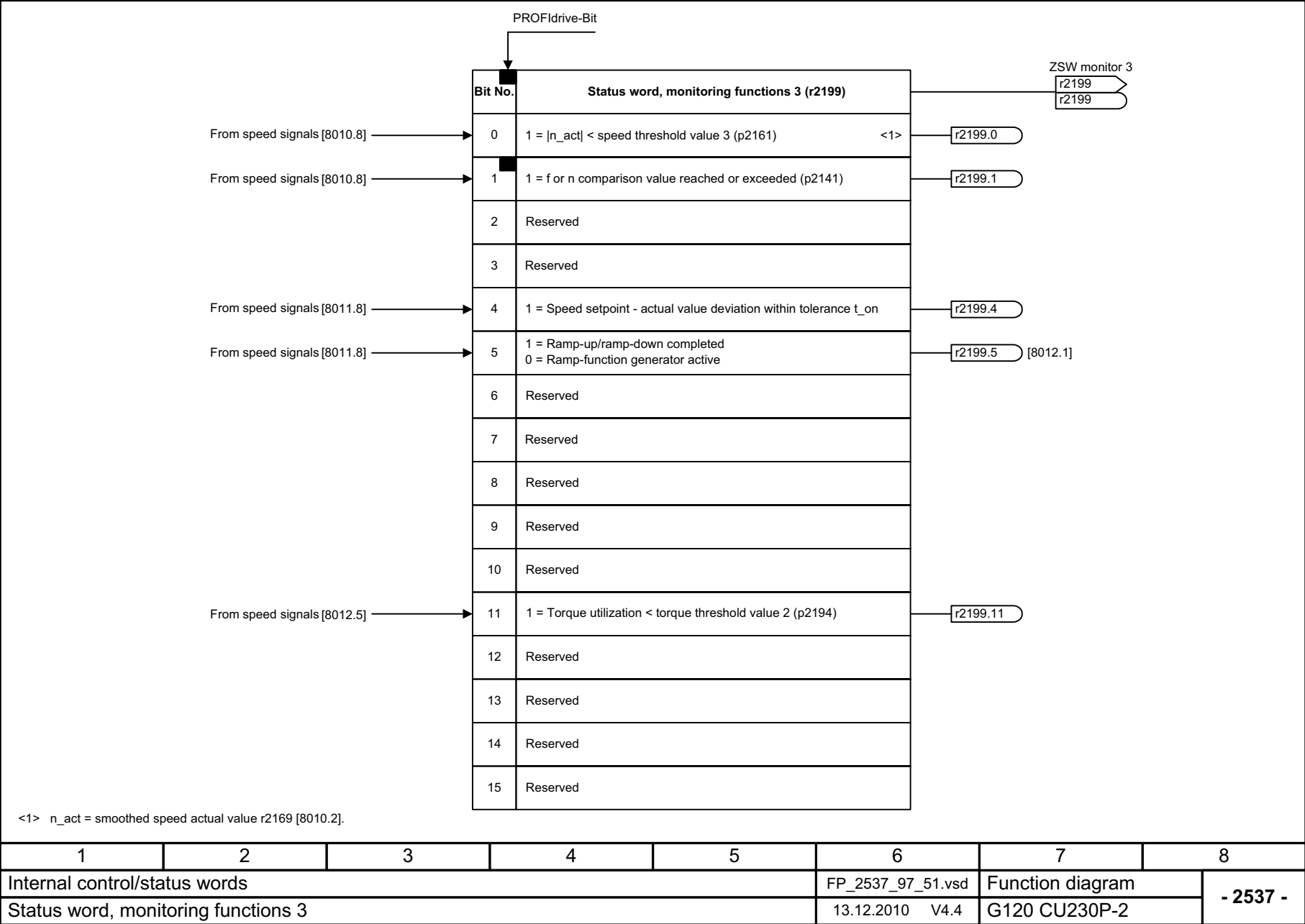
Fig. 2-57 2537 – Status word, monitoring functions 3
