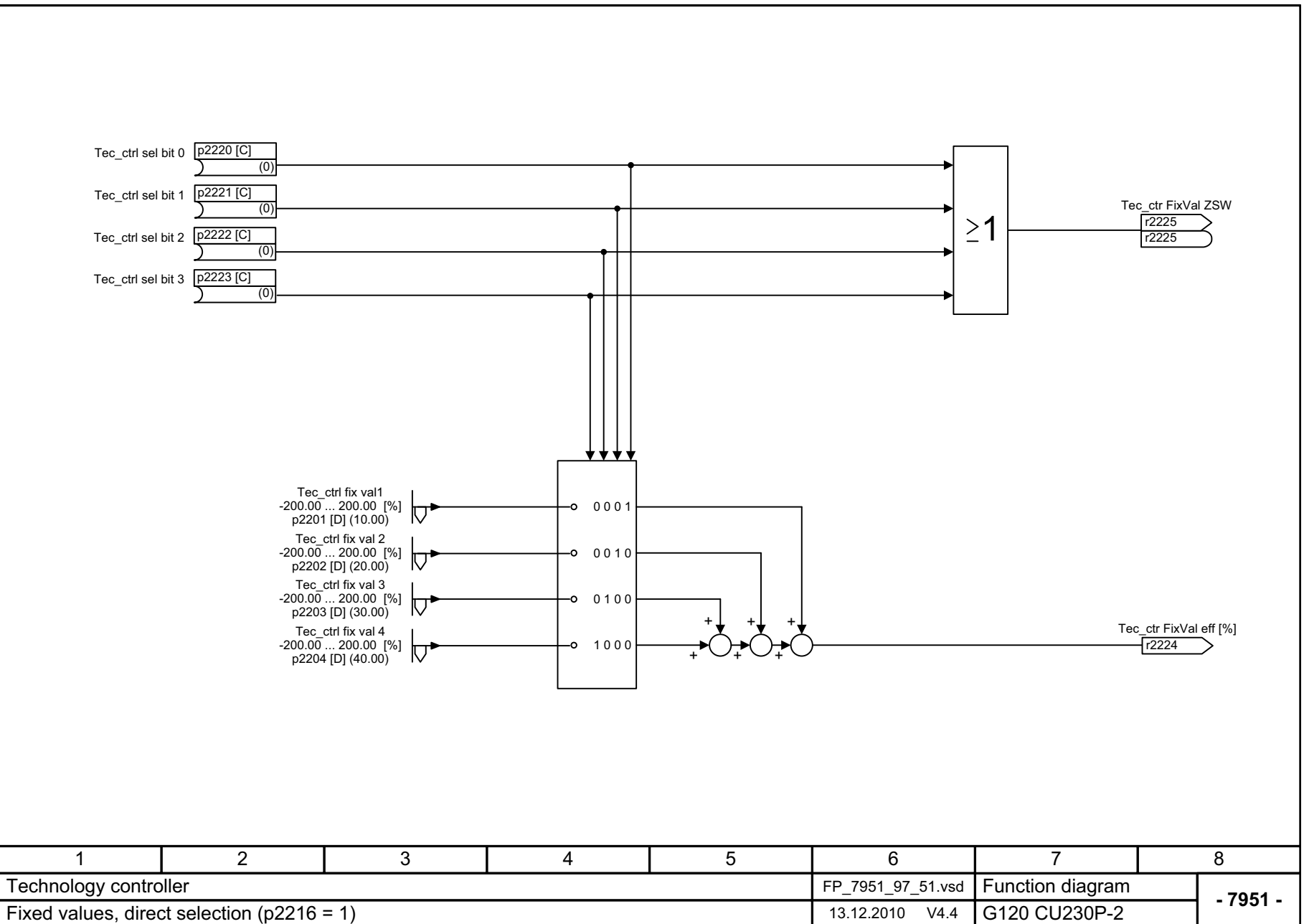
Fig. 2-120 7951 – Fixed values, direct selection (p2216 = 1)
