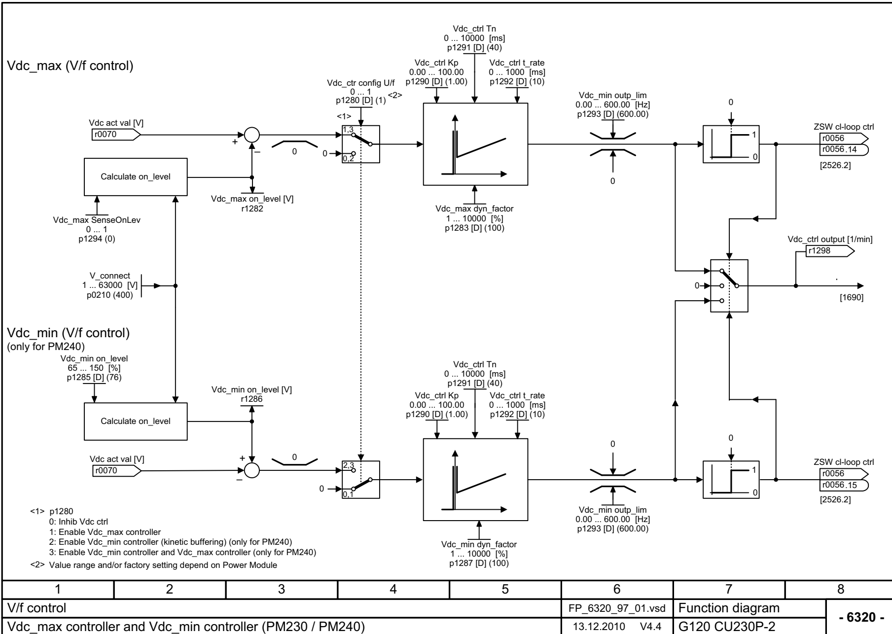
Fig. 2-72 6320 – Vdc_max controller and Vdc_min controller (V/f control, PM230 / PM240)
