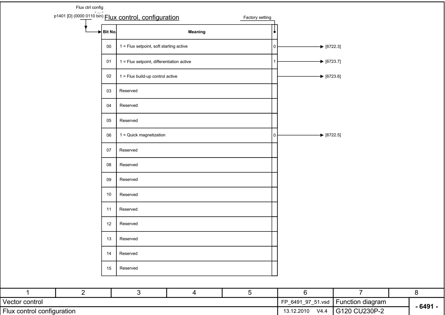
Fig. 2-80 6491 – Flux control configuration
