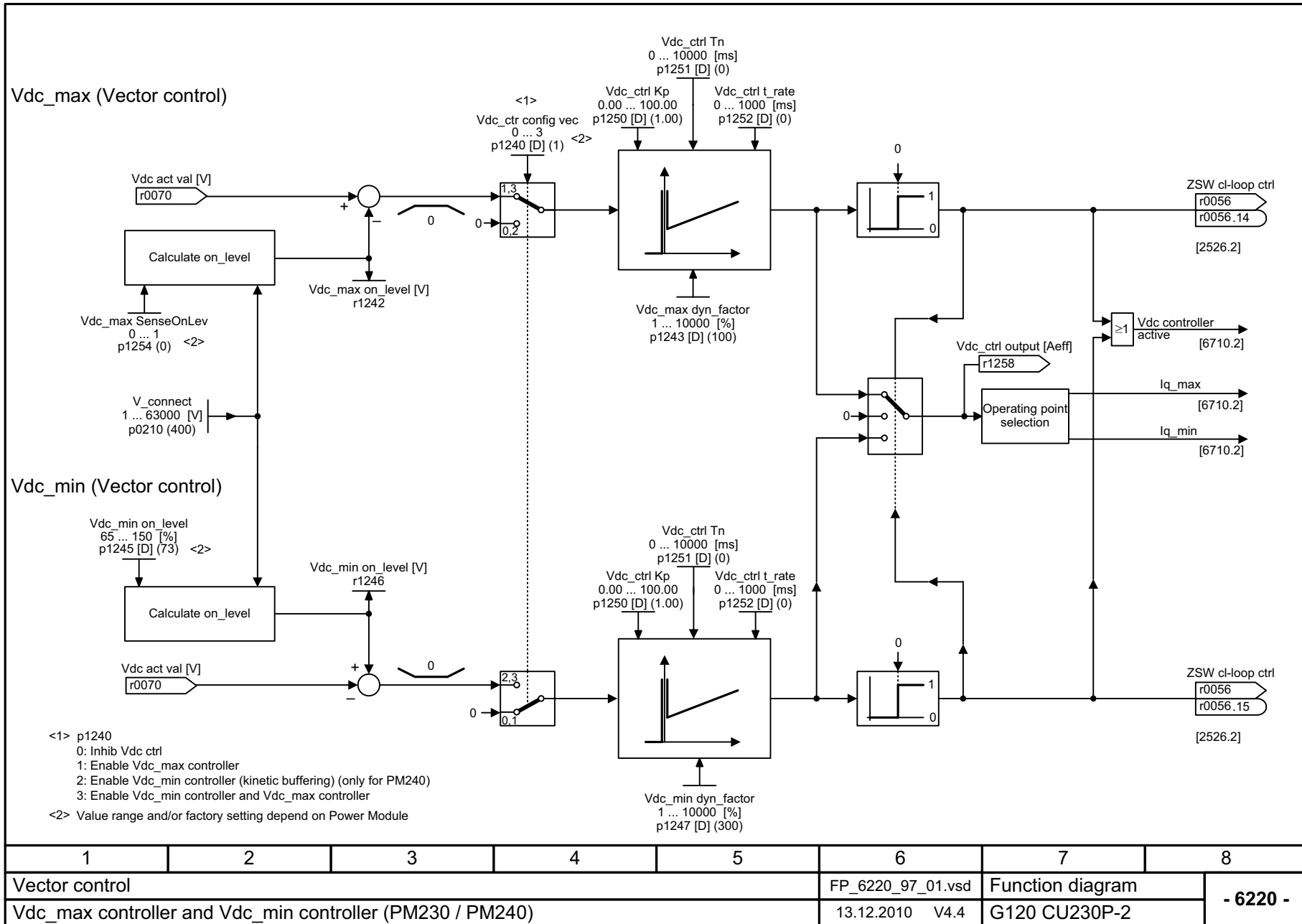
Fig. 2-78 6220 – Vdc_max controller and Vdc_min controller (PM230 / PM240)
