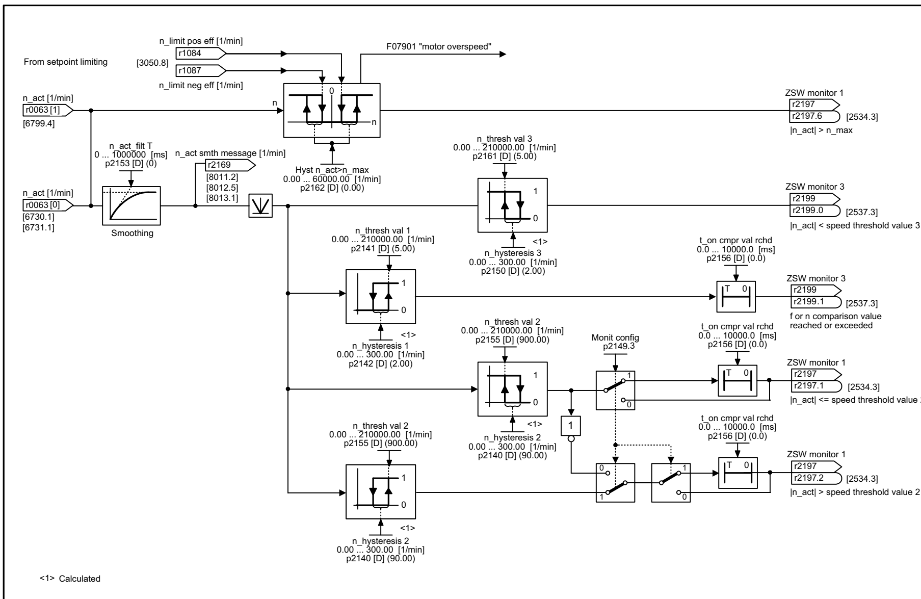
Fig. 2-123 8010 – Speed signals 1
