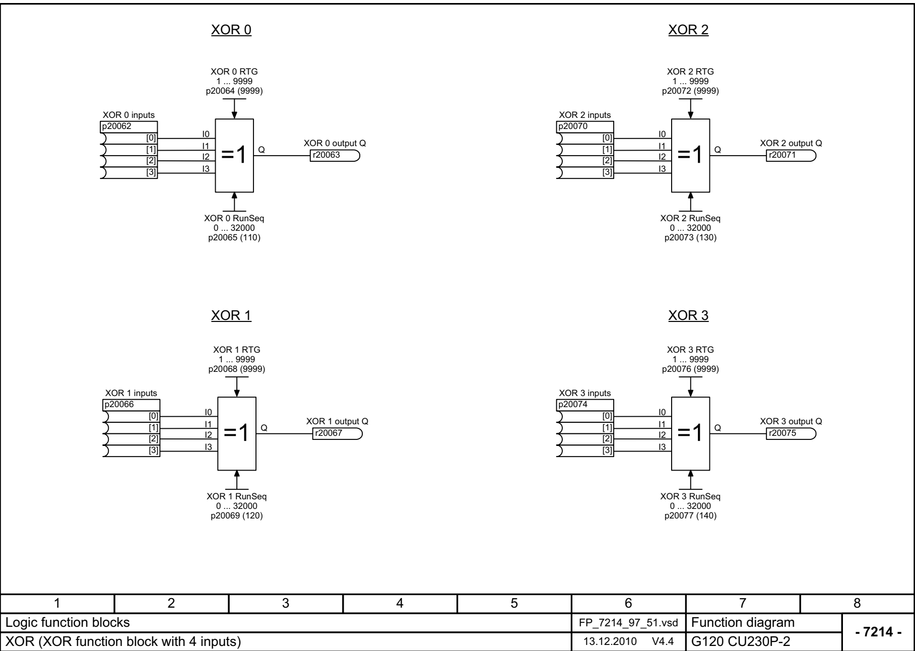
Fig. 2-95 7214 – XOR (XOR function block with 4 inputs)
