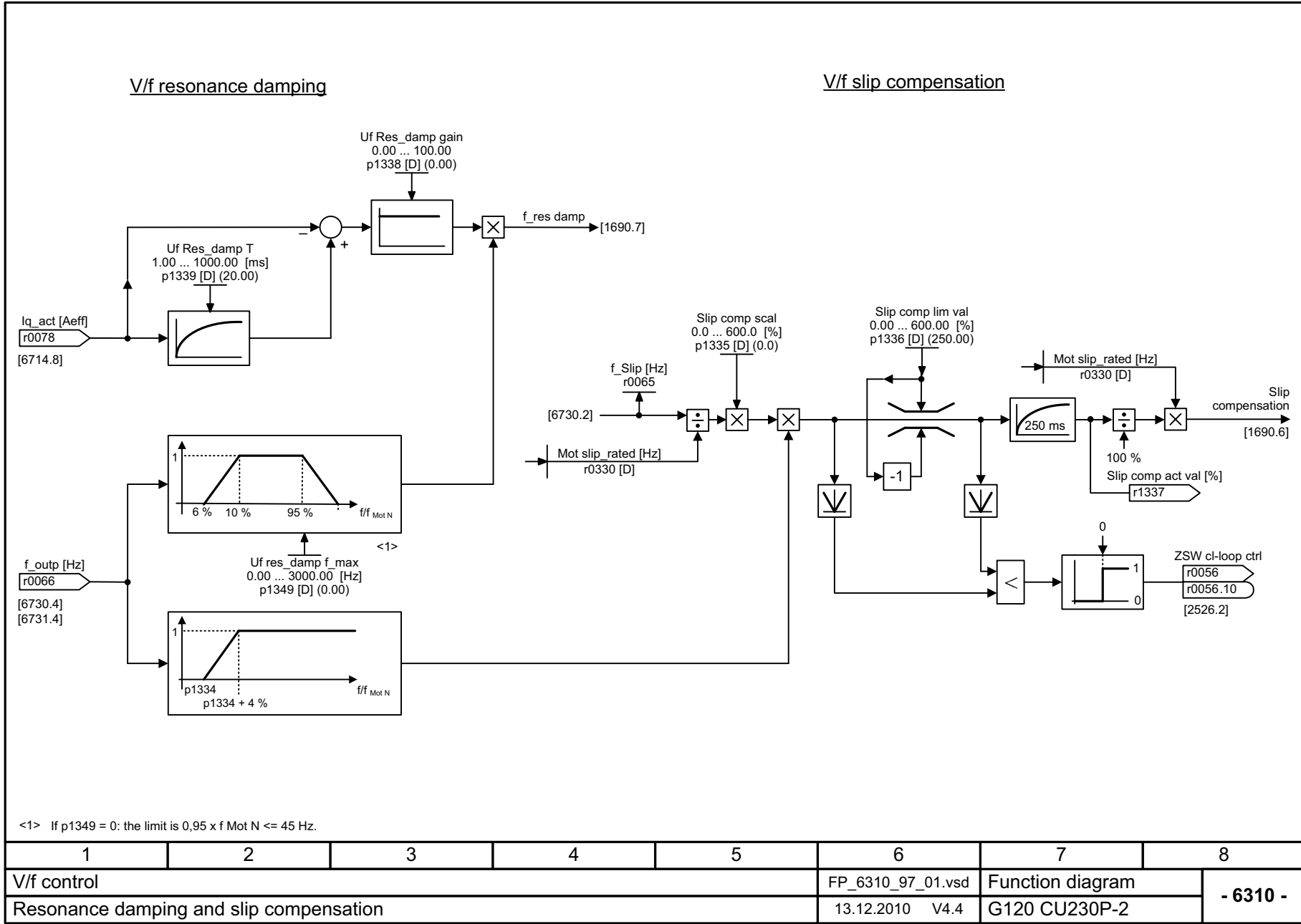
Fig. 2-71 6310 – Resonance damping and slip compensation
