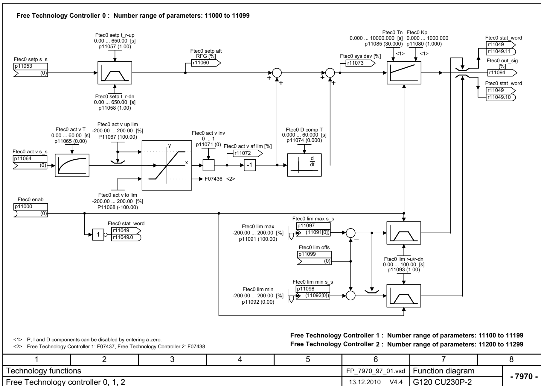
Fig. 2-113 7970 – Free Technology controller 0, 1, 2
