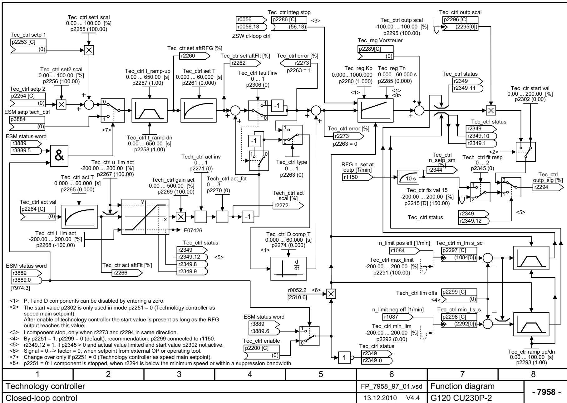
Fig. 2-122 7958 – Closed-loop control
