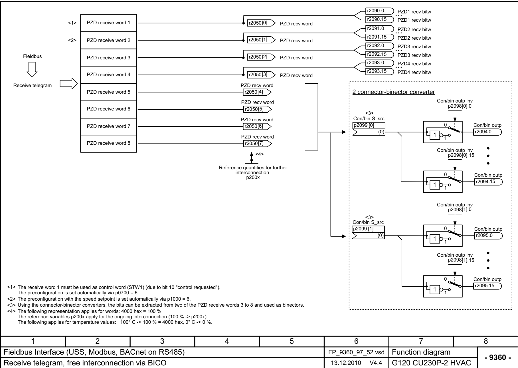
Fig. 2-22 9360 – Receive telegram, free interconnection via BICO
