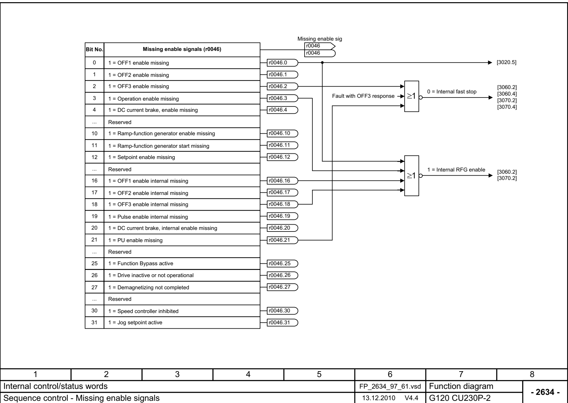
Fig. 2-60 2634 – Sequence control - Missing enable signals
