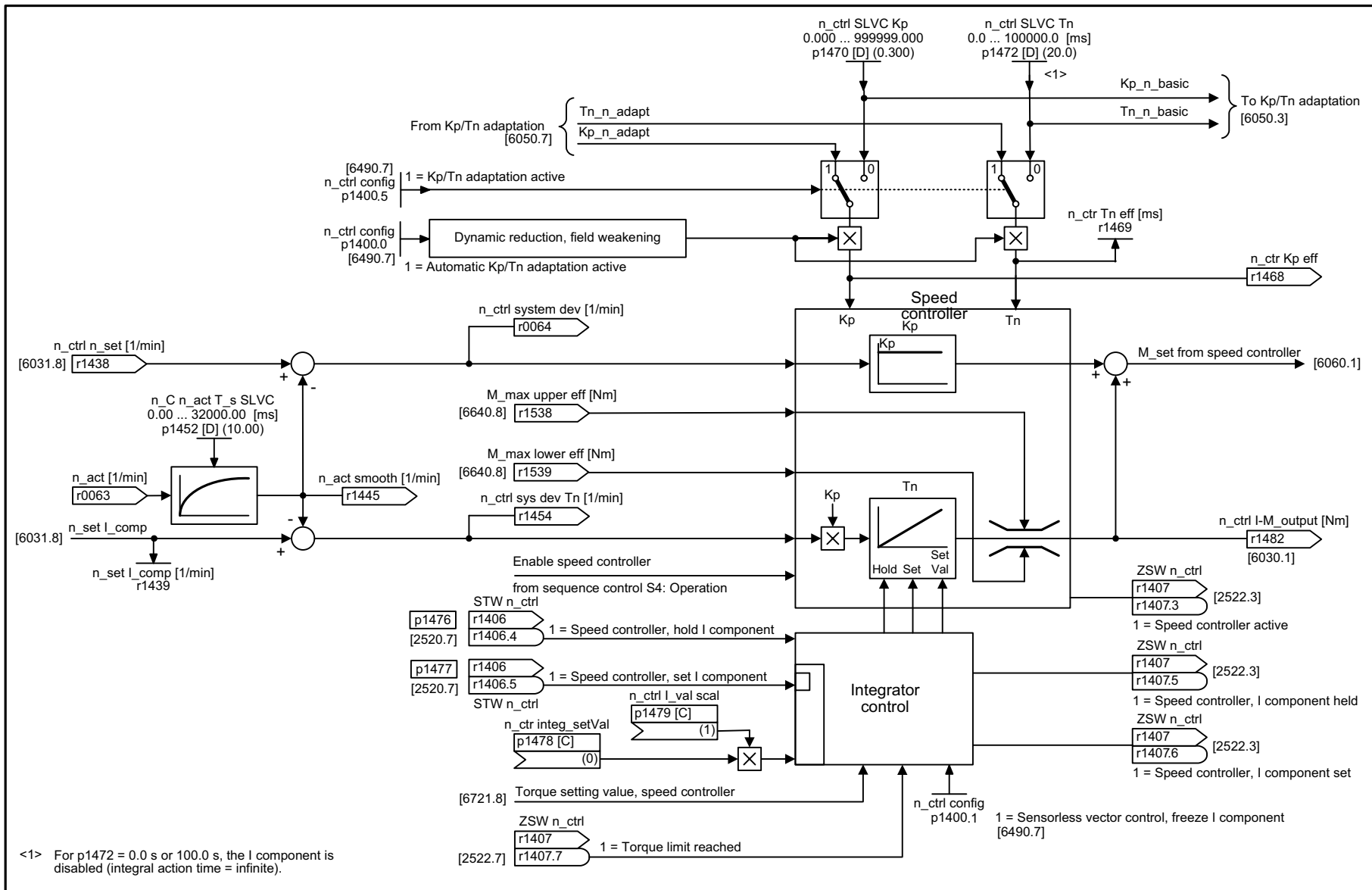
Fig. 2-75 6040 – Speed controller
