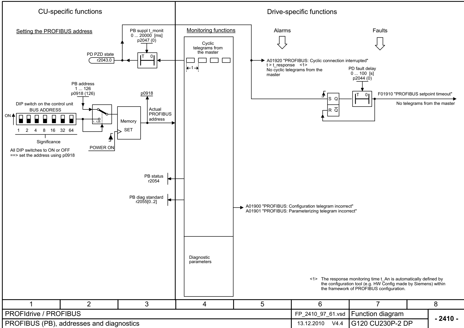
Fig. 2-25 2410 – PROFIBUS, addresses and diagnostics
