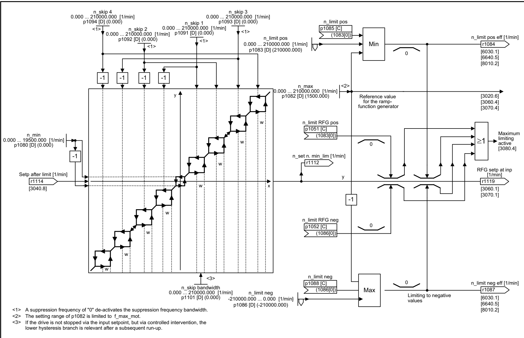
Fig. 2-66 3050 – Skip frequency bands and frequency limitations
