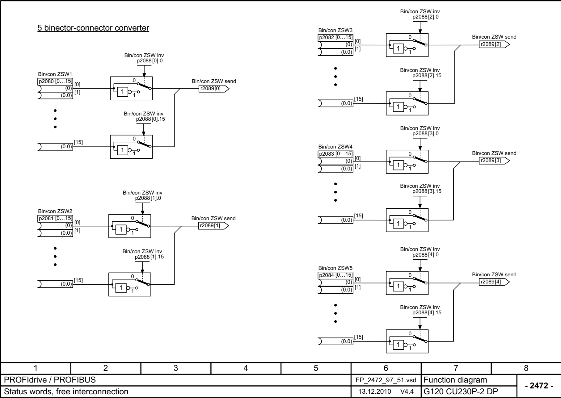
Fig. 2-37 2472 – Status words, free interconnection
