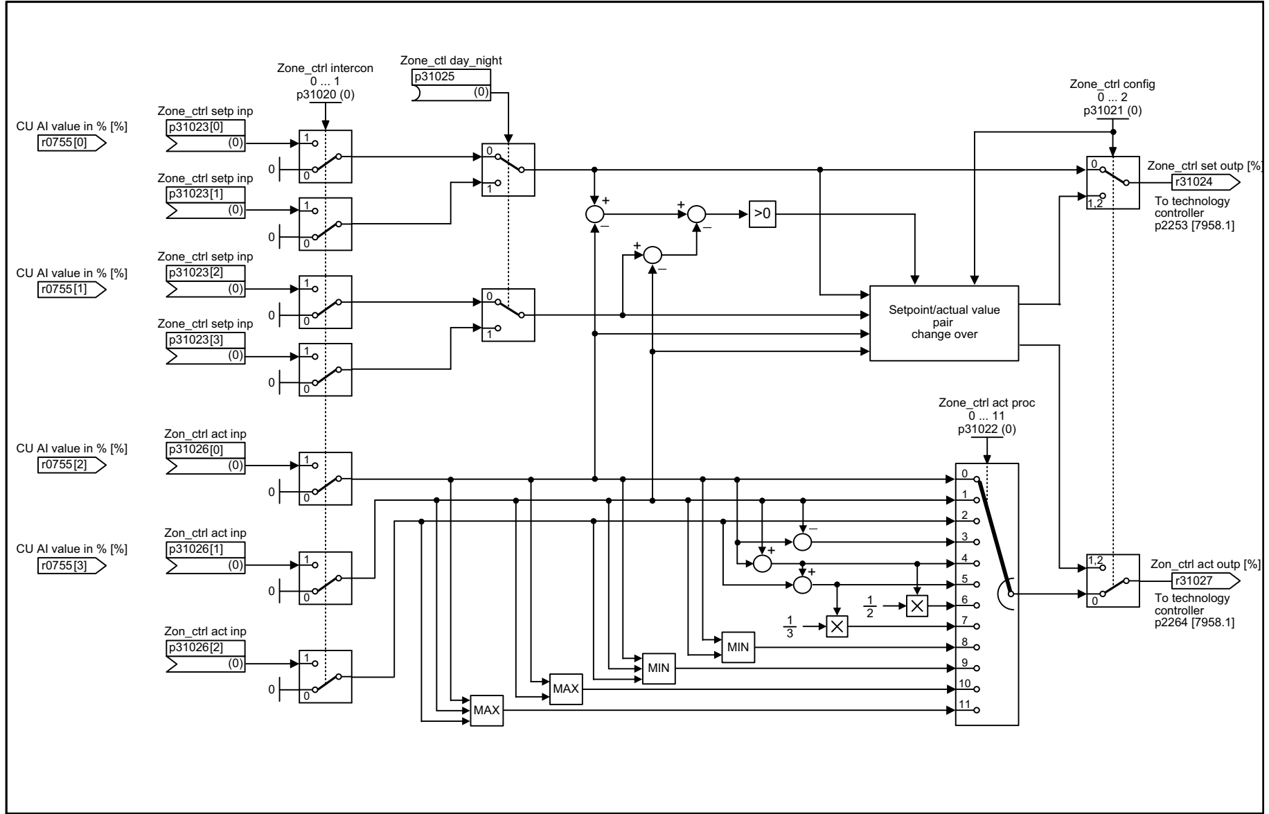
Fig. 2-114 7972 – Multi Zone Control
