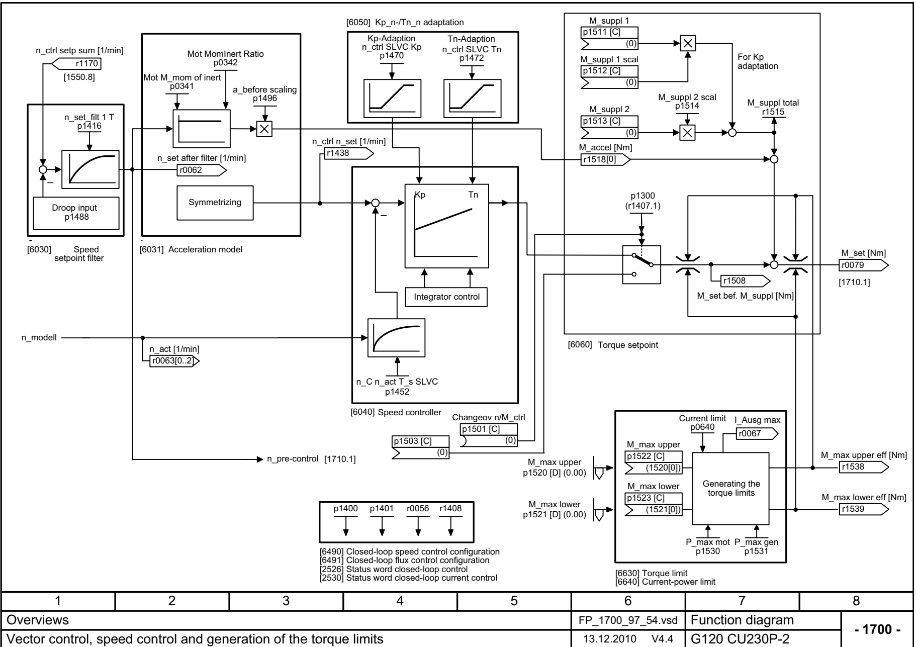
Fig. 2-9 1700 – Vector control, speed control and generation of the torque limits
