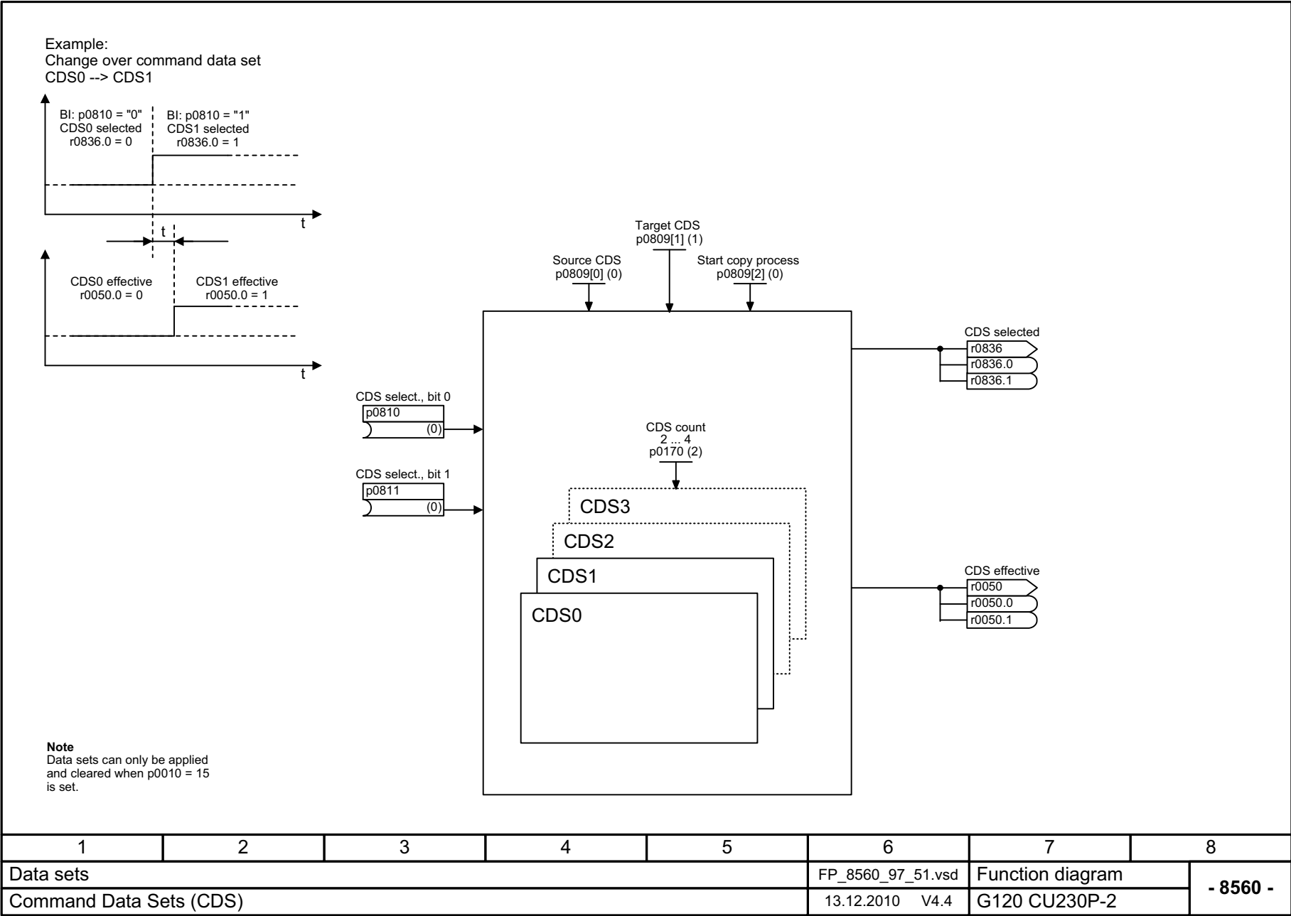
Fig. 2-136 8560 – Command Data Sets (CDS)
