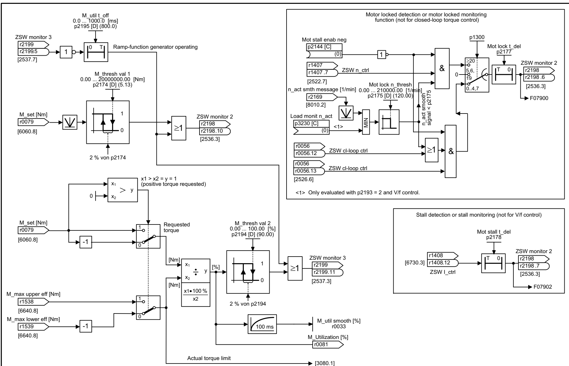
Fig. 2-125 8012 – Torque signals, motor locked/stalled
