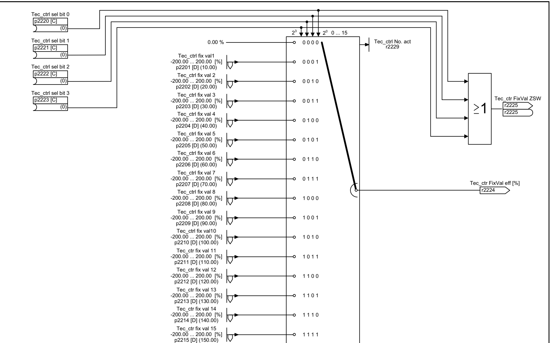
Fig. 2-119 7950 – Fixed values, binary selection (p2216 = 2)
