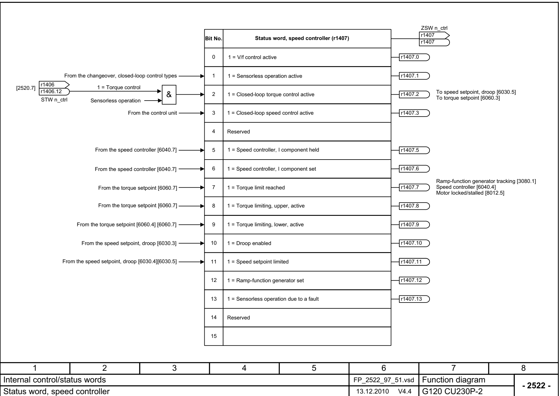
Fig. 2-52 2522 – Status word, speed controller
