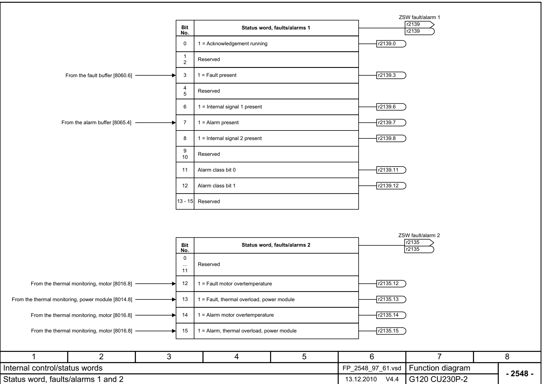
Fig. 2-59 2548 – Status word, faults/alarms 1 and 2
