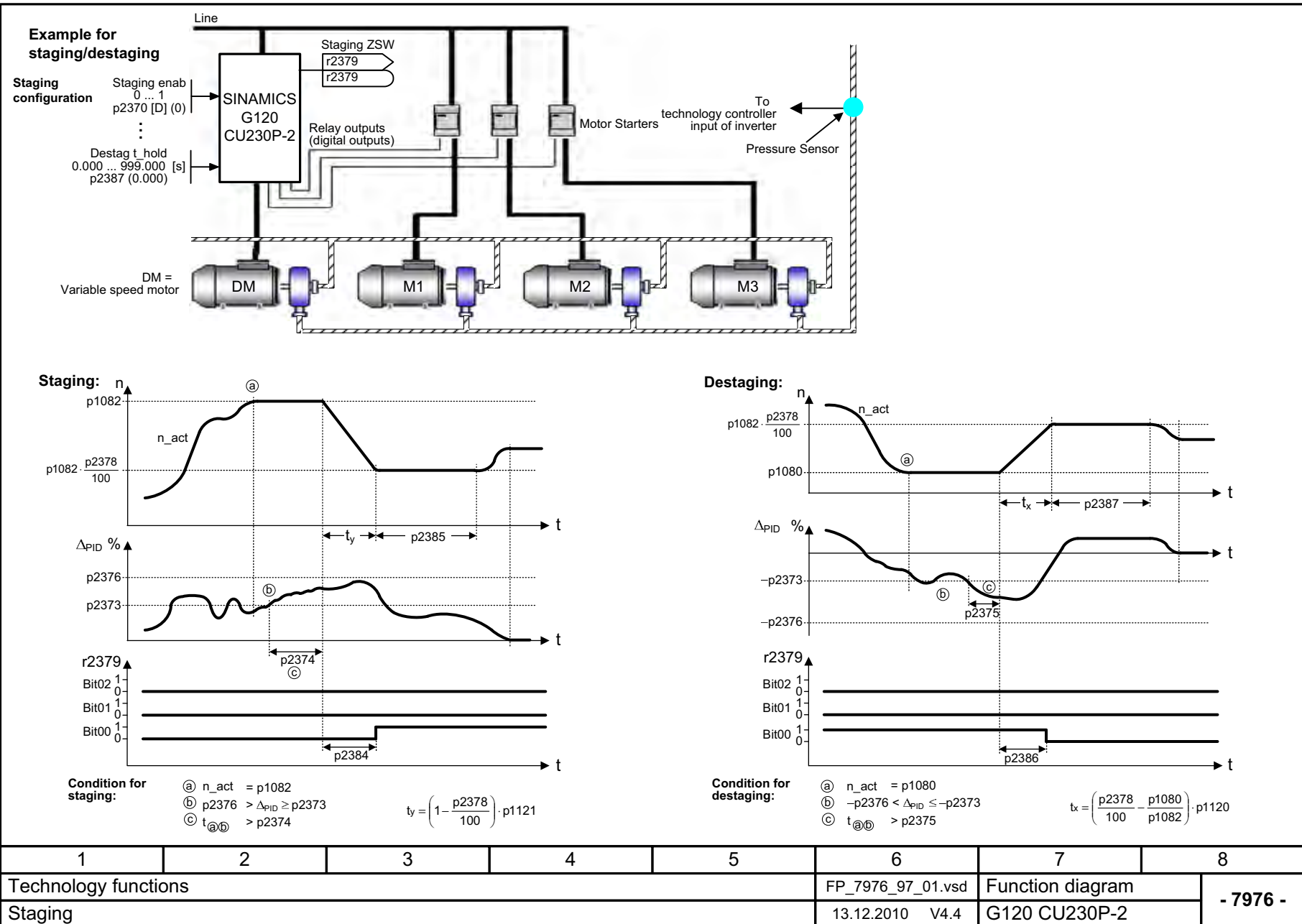
Fig. 2-117 7976 – Staging
