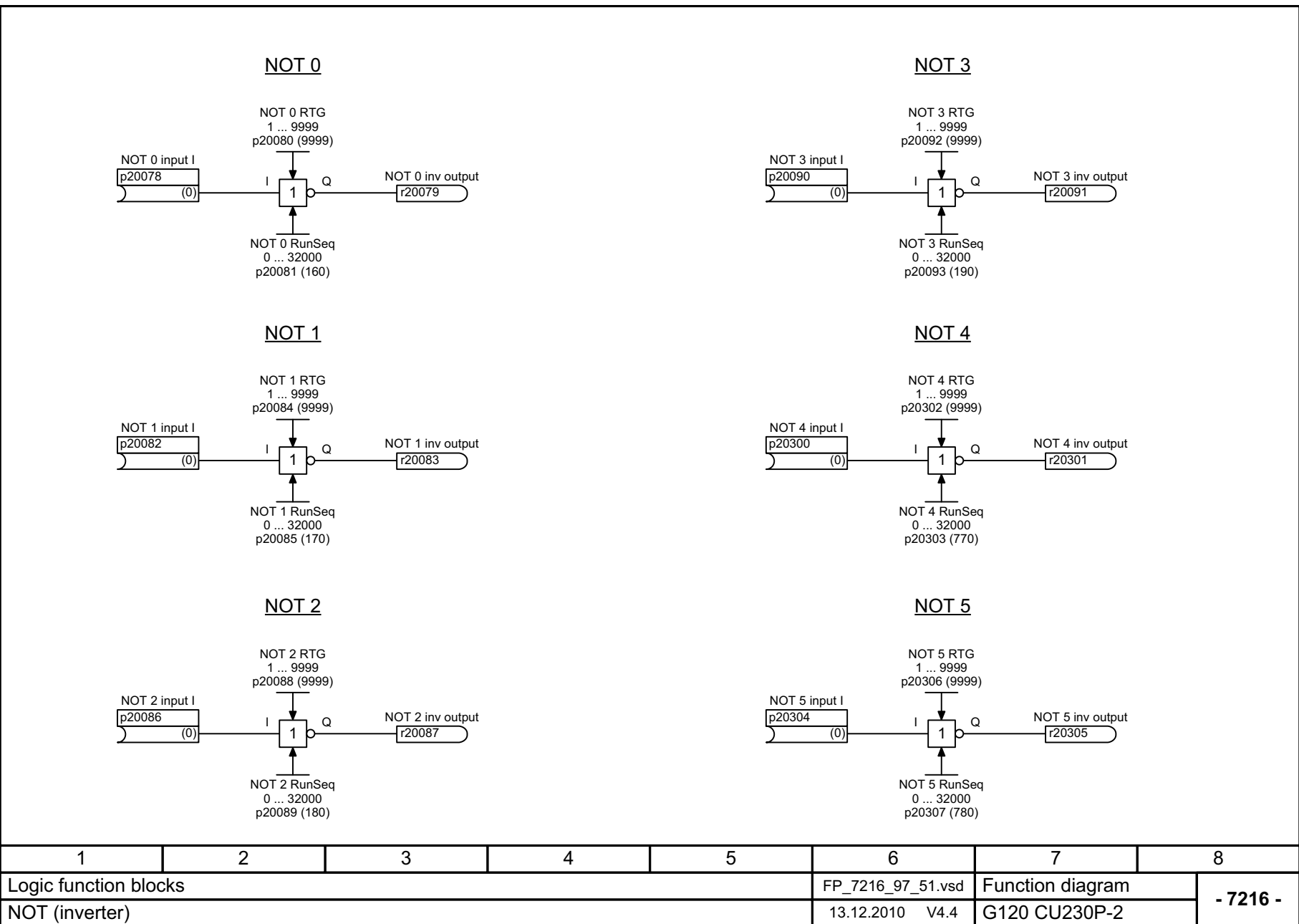
Fig. 2-96 7216 – NOT (inverter)
