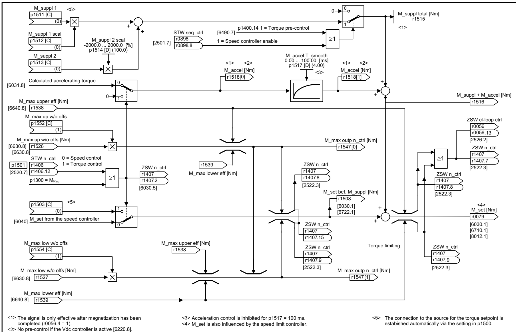
Fig. 2-77 6060 – Torque setpoint
