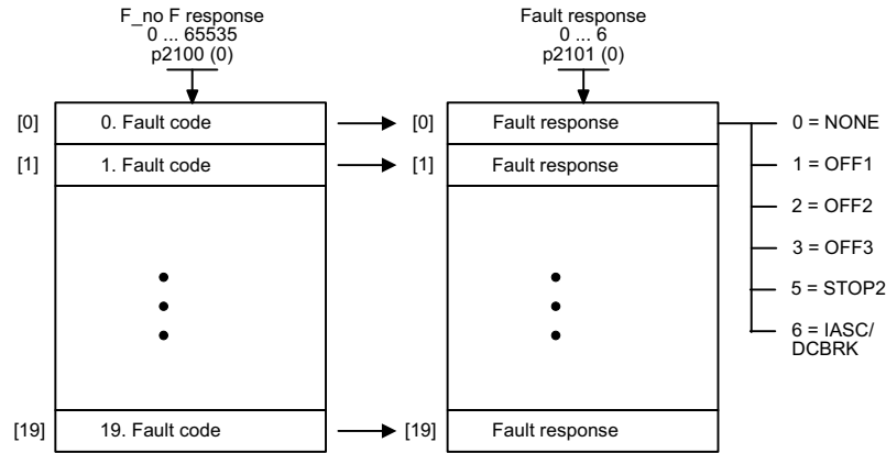
Fig. 2-135 8075 – Fault/warning configuration
