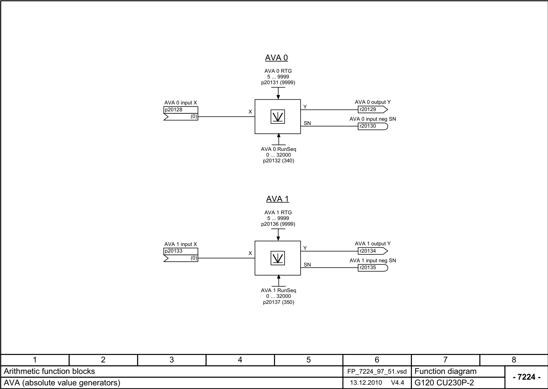
Fig. 2-99 7224 – AVA (absolute value generators)
