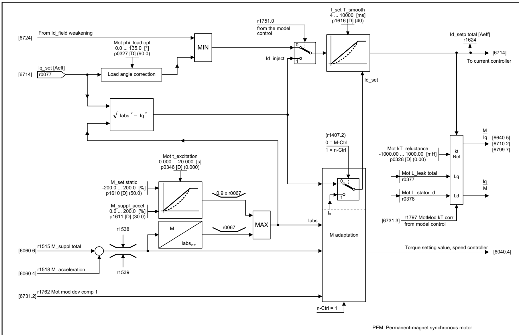
Fig. 2-85 6721 – Id setpoint (PEM, p0300 = 2xx)
