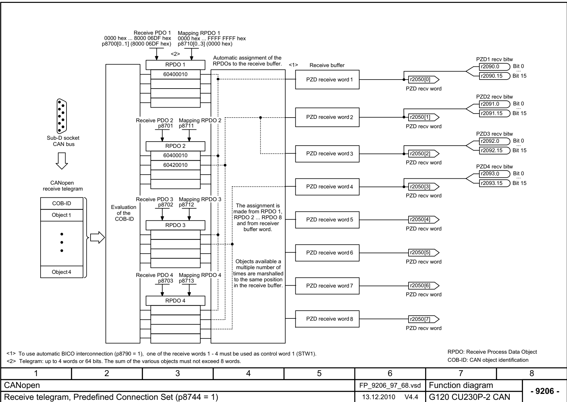
Fig. 2-39 9206 – Receive telegram, Predefined Connection Set (p8744 = 1)
