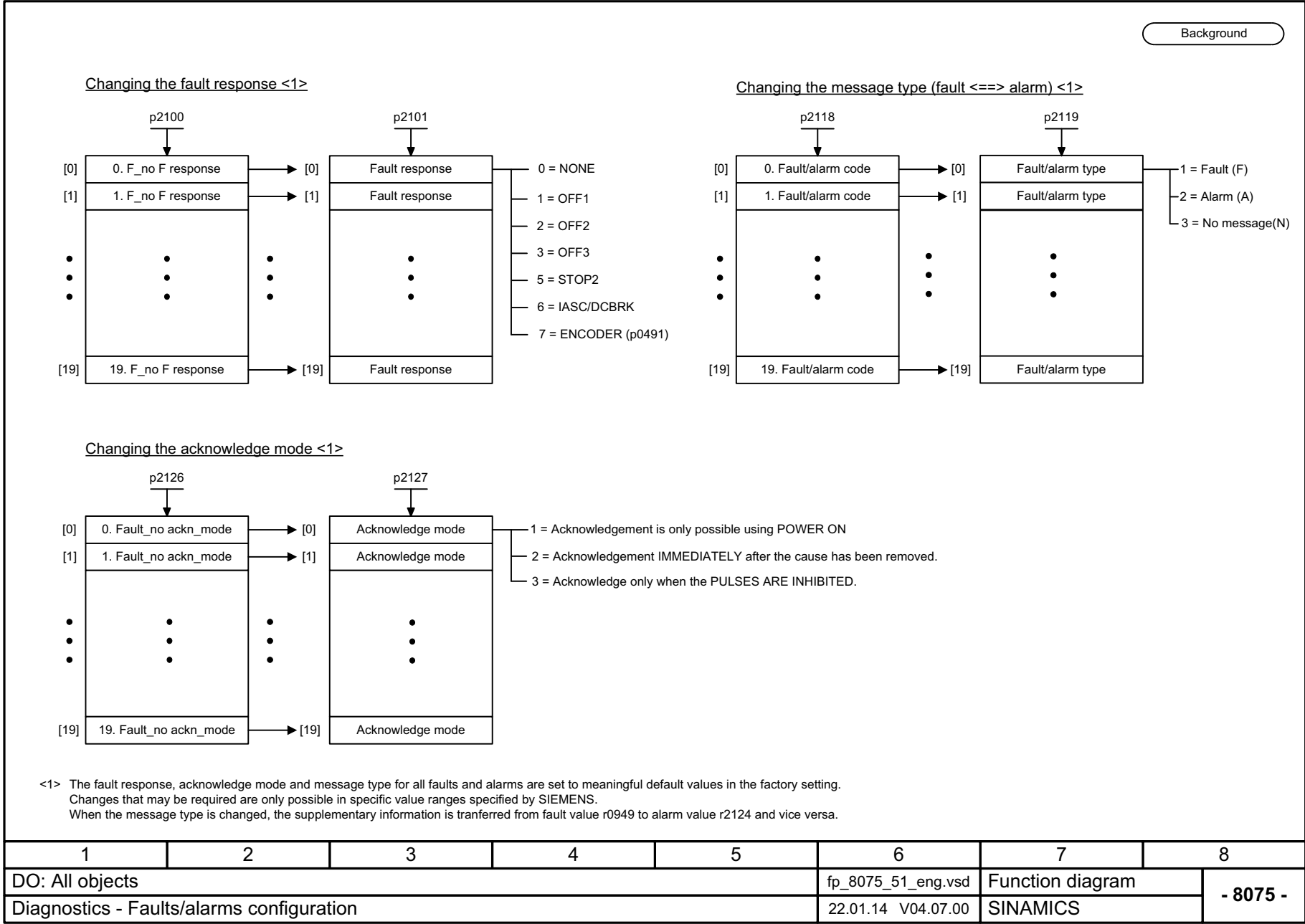
Fig. 3-165 8075 – Faults/alarms configuration
