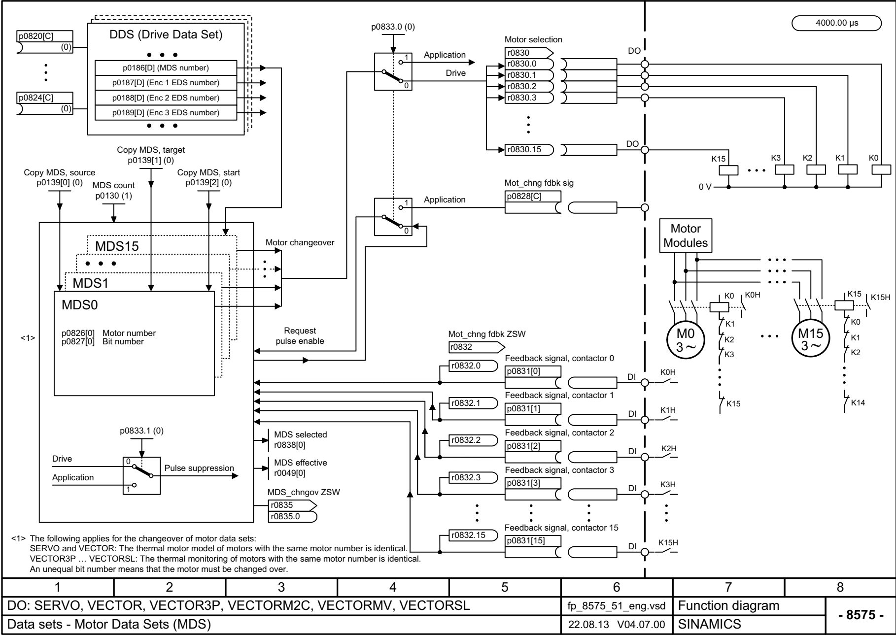
Fig. 3-170 8575 – Motor Data Sets (MDS)
