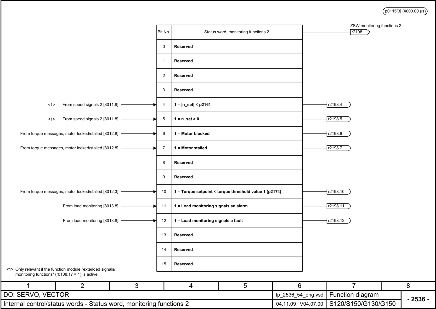
Fig. 3-65 2536 – Status word, monitoring functions 2
