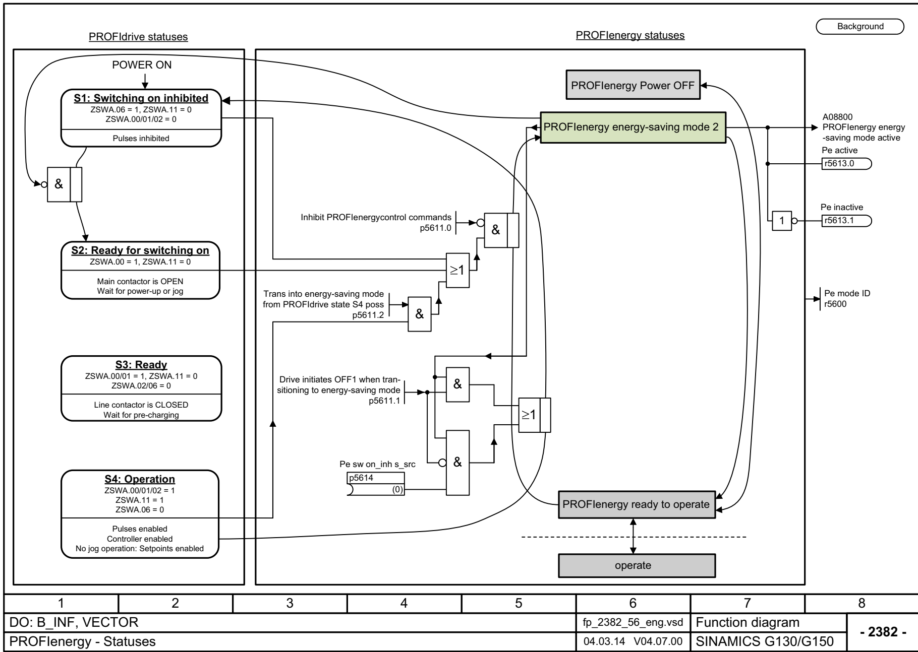
Fig. 3-13 2382 – States
