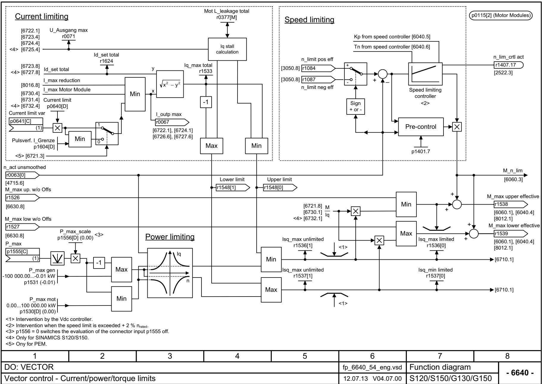
Fig. 3-131 6640 – Current/power/torque limits
