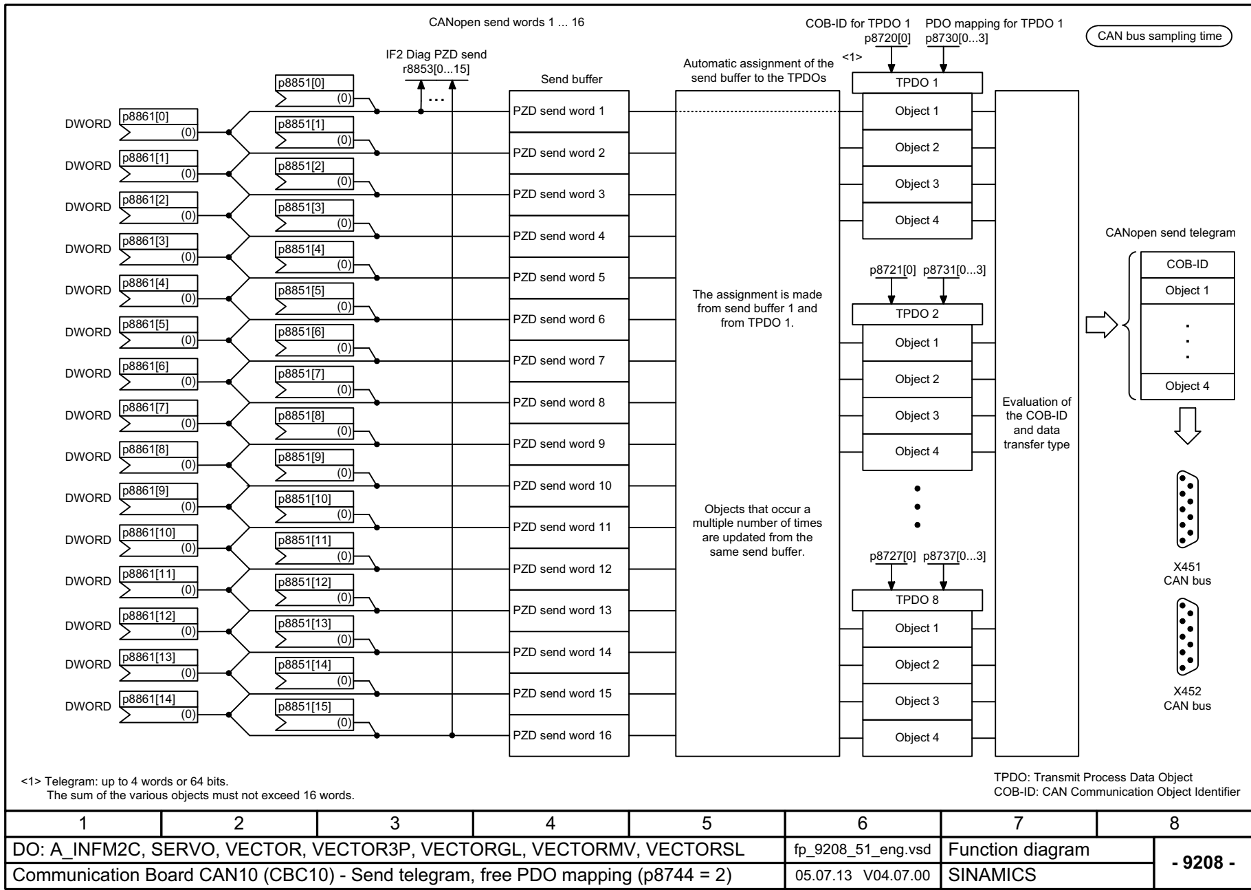
Fig. 3-186 9208 – Send telegram, free PDO mapping (p8744 = 2) SINAMICS G130/G150 List Manual (LH2), 04/2014, A5E03263479A
