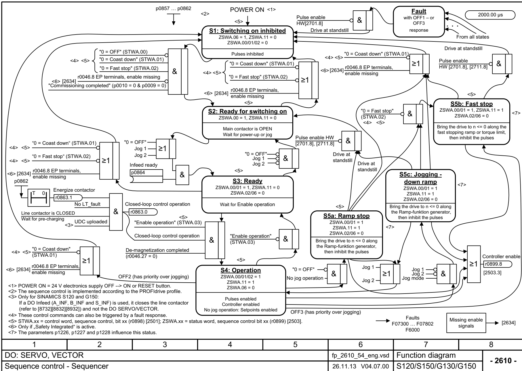
Fig. 3-69 2610 – Sequencer
