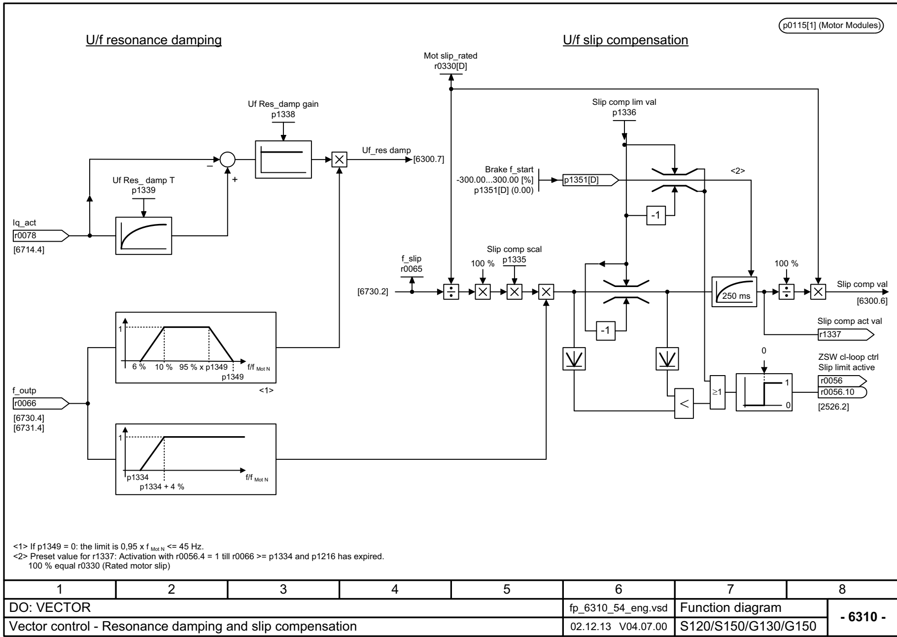
Fig. 3-126 6310 – Resonance damping and slip compensation SINAMICS G130/G150 List Manual (LH2), 04/2014, A5E03263479A
