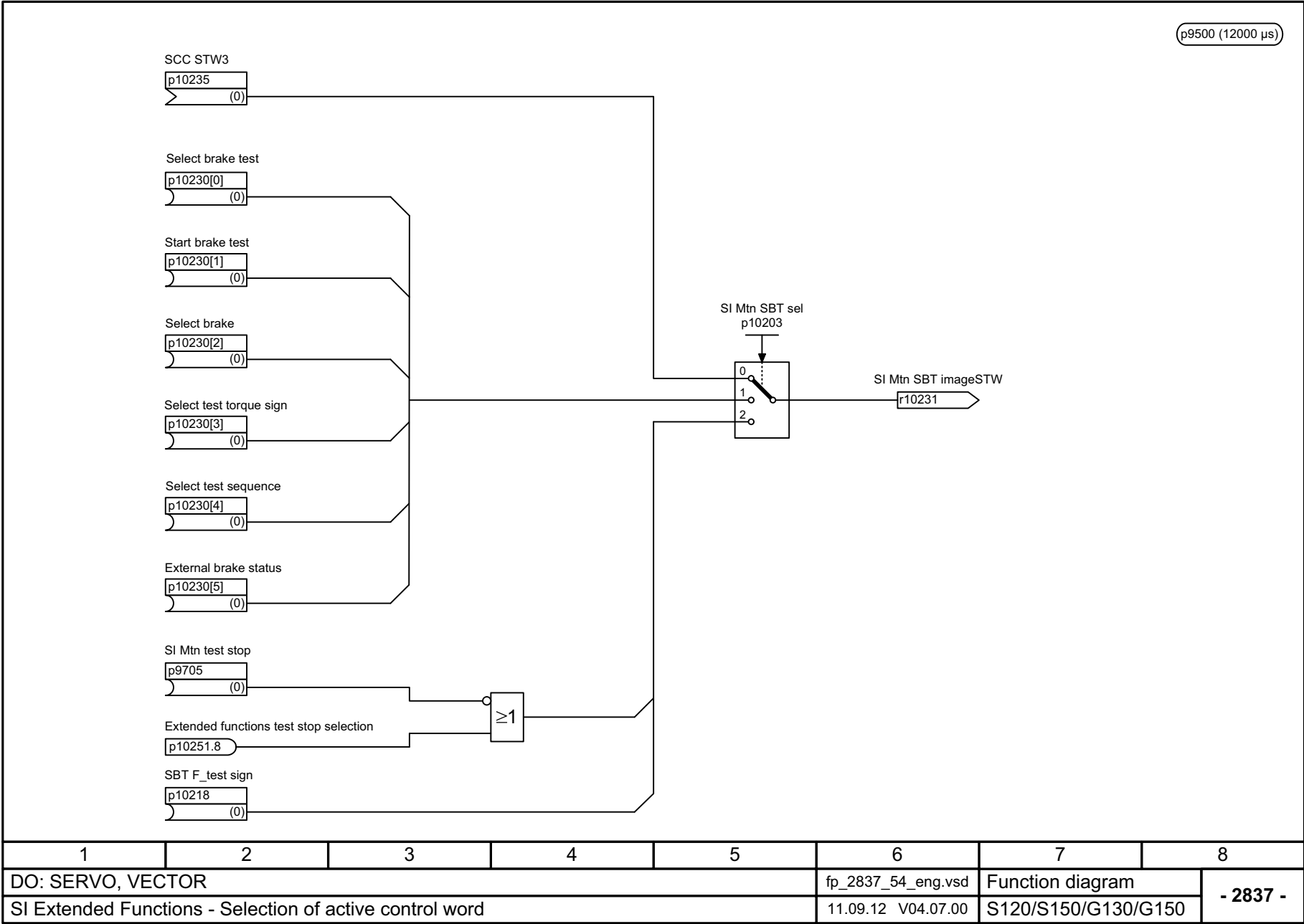
Fig. 3-90 2837 – Selection of active control word
