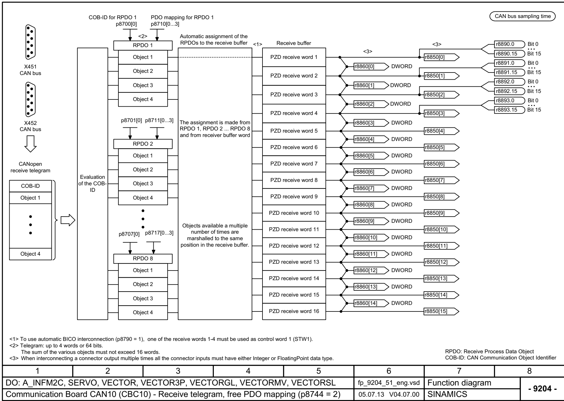
Fig. 3-184 9204 – Receive telegram, free PDO mapping (p8744 = 2) SINAMICS G130/G150 List Manual (LH2), 04/2014, A5E03263479A 1239
