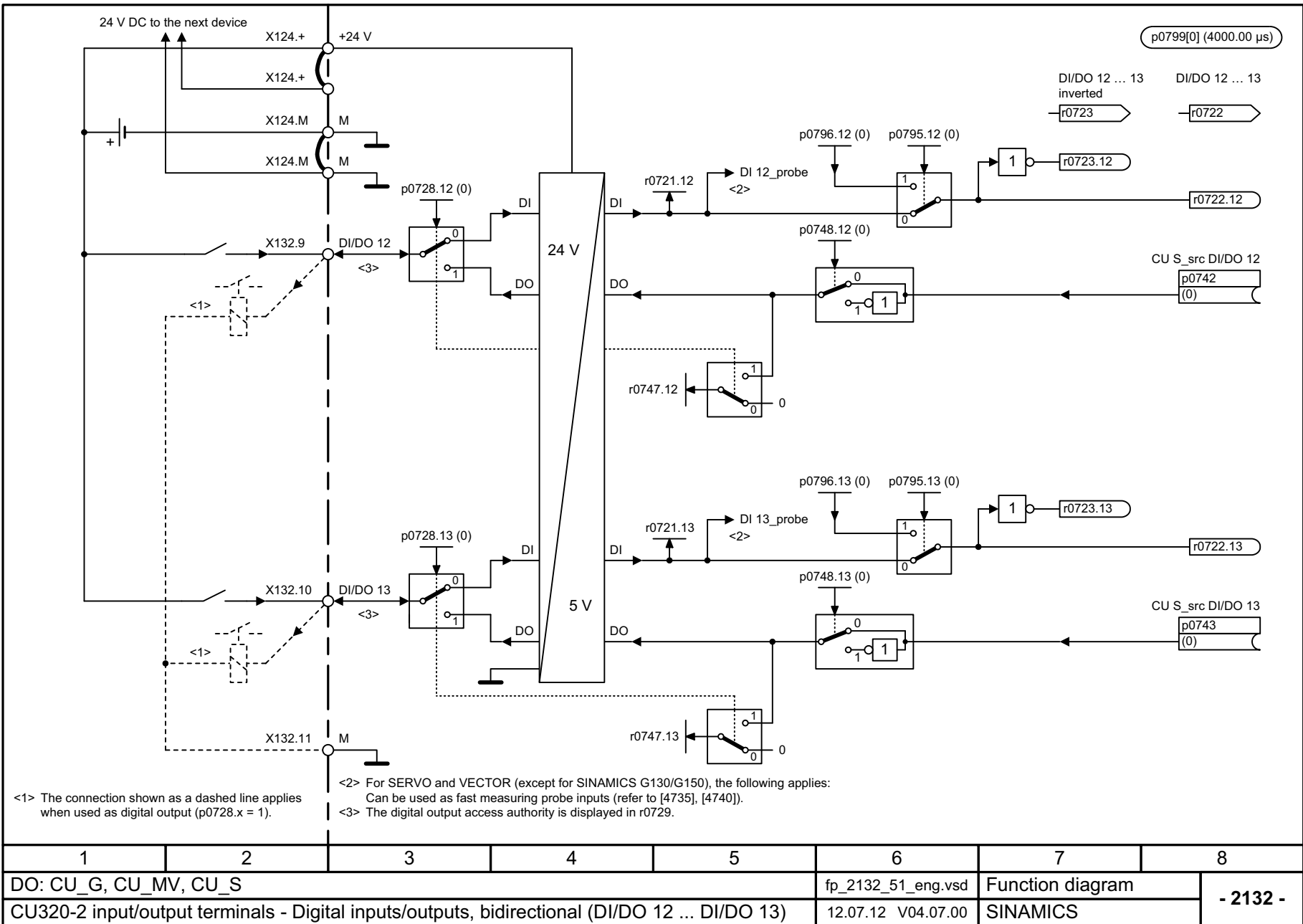
Fig. 3-10 2132 – Digital inputs/outputs, bidirectional (DI/DO 12 ... DI/DO 13)
