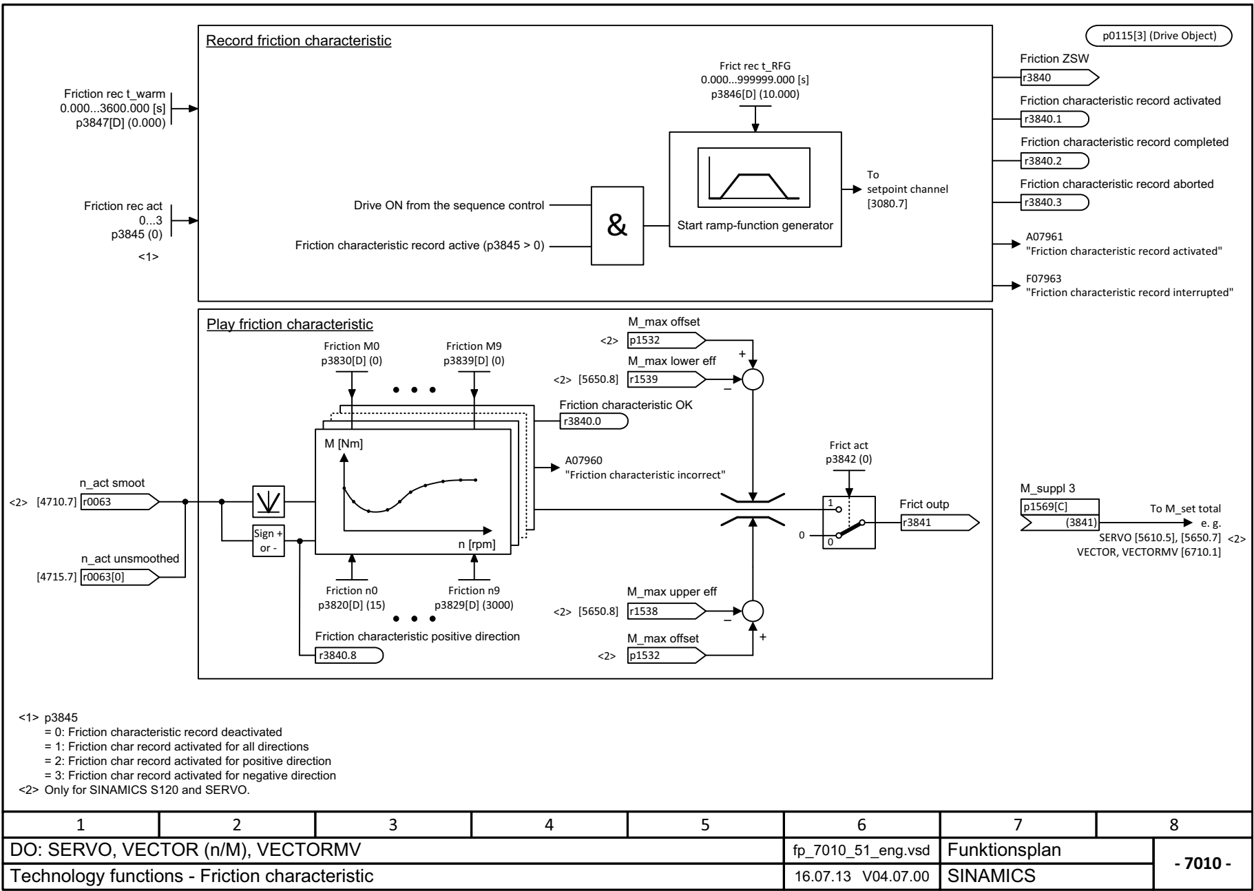
Fig. 3-142 7010 – Friction characteristic
