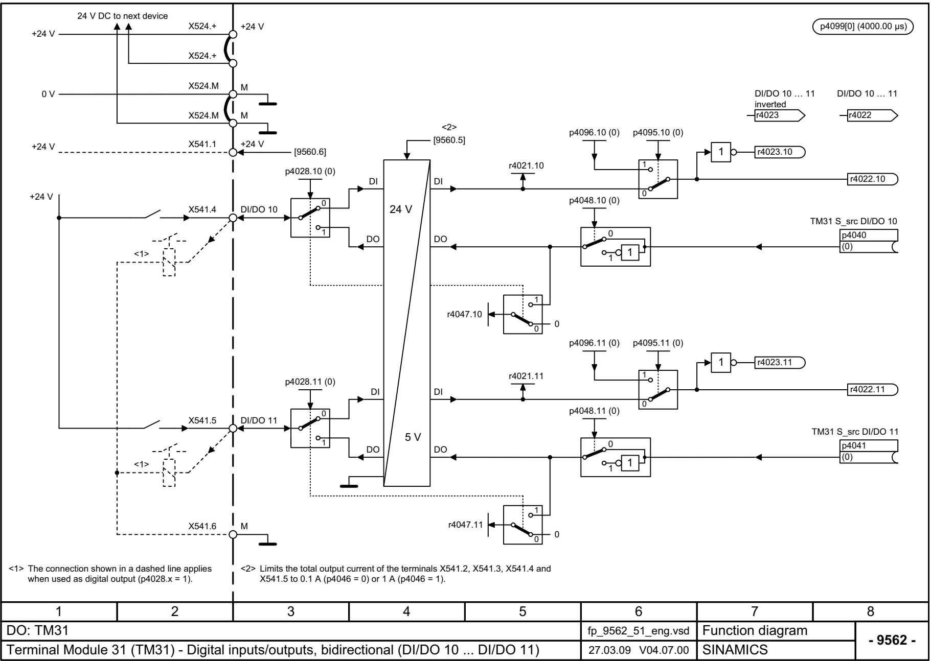
Fig. 3-195 9562 – Digital inputs/outputs, bidirectional (DI/DO 10 ... DI/DO 11)
