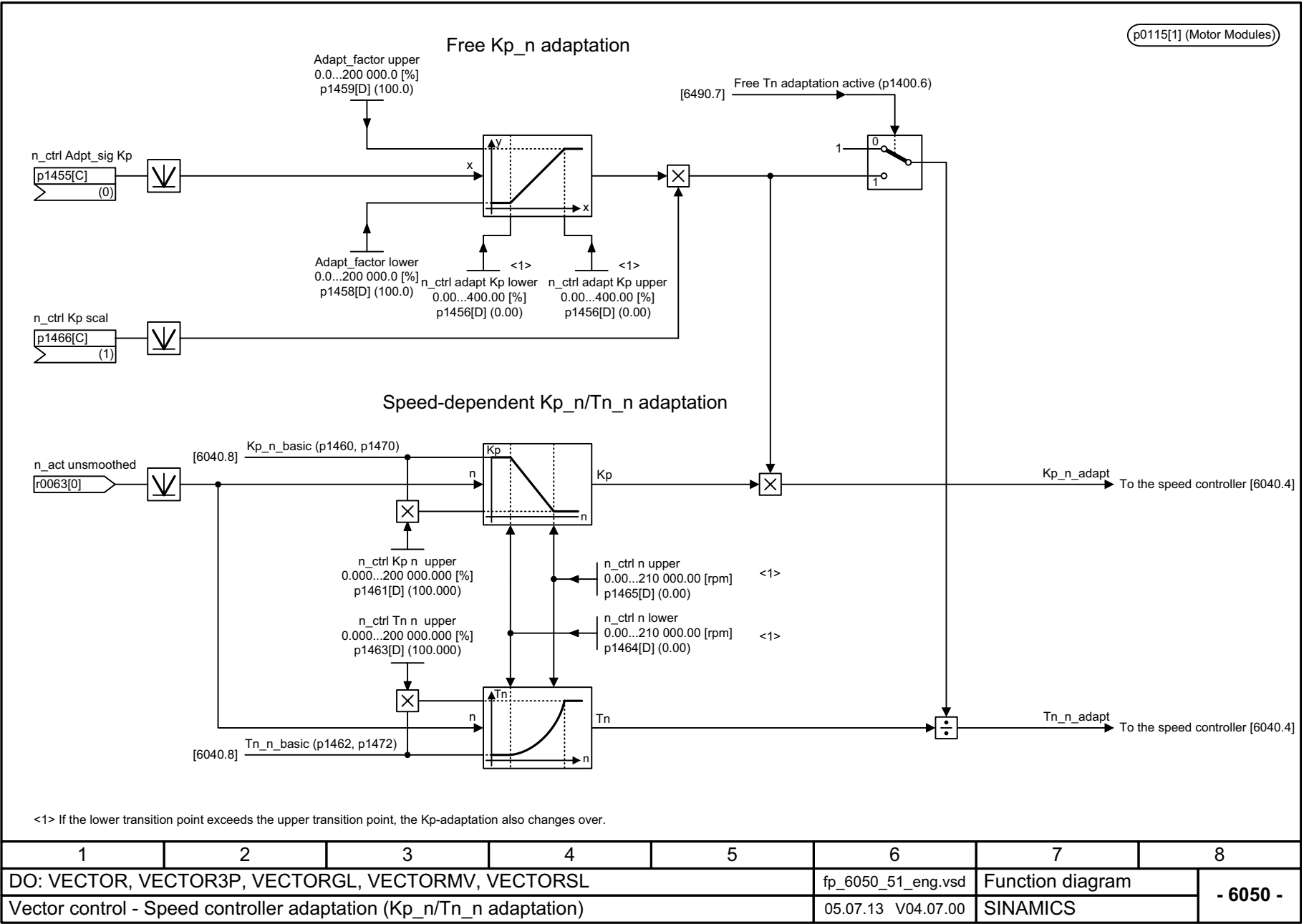
Fig. 3-121 6050 – Speed controller adaptation (Kp_n/Tn_n adaptation)
