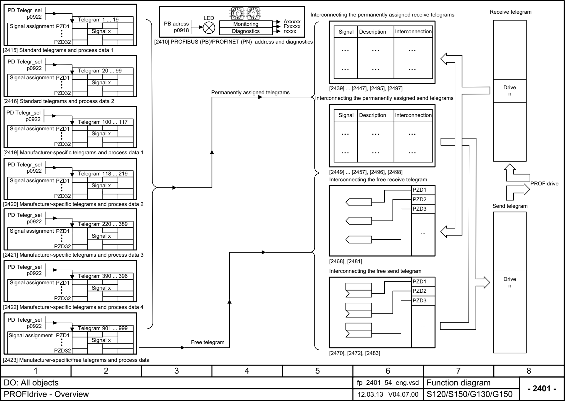
Fig. 3-14 2401 – Overview
