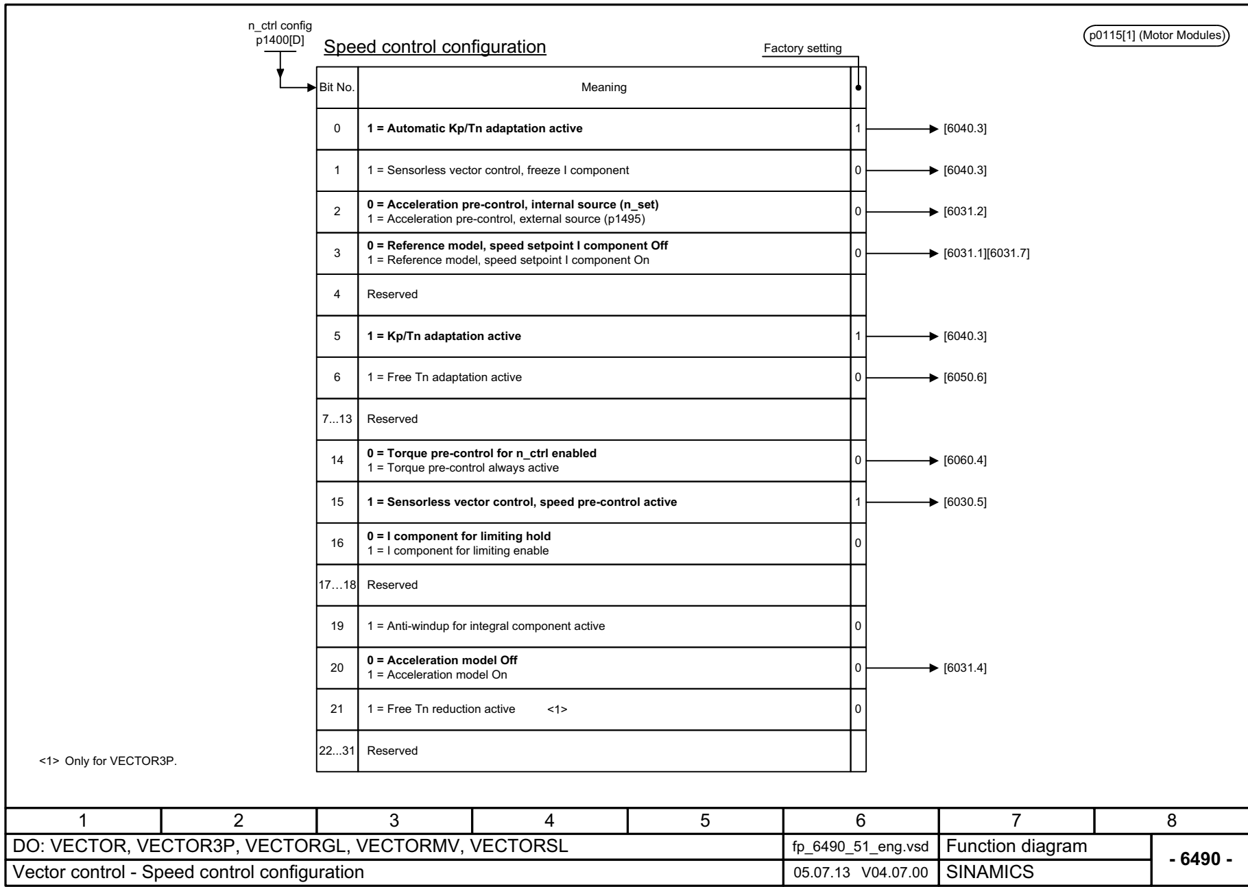
Fig. 3-128 6490 – Speed control configuration SINAMICS G130/G150 List Manual (LH2), 04/2014, A5E03263479A
