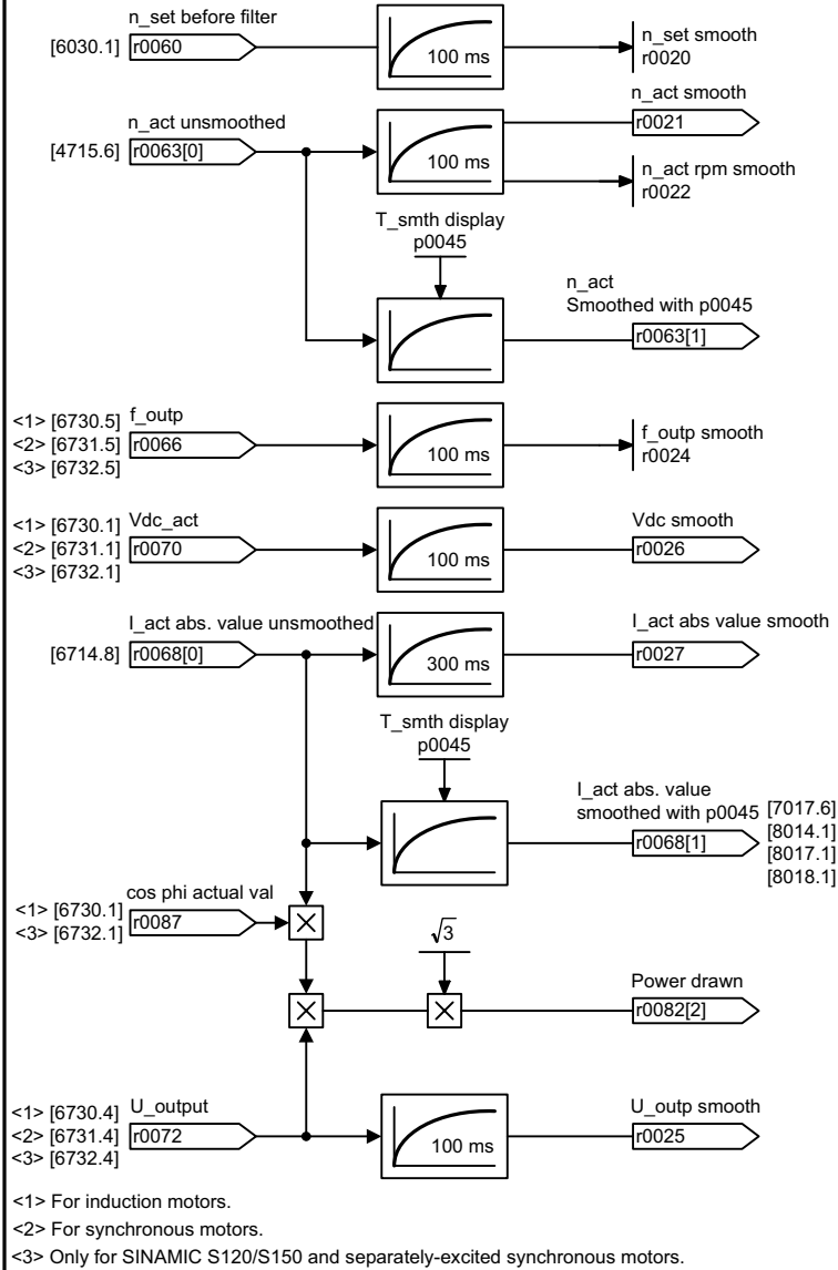
Fig. 3-141 6799 – Display signals
