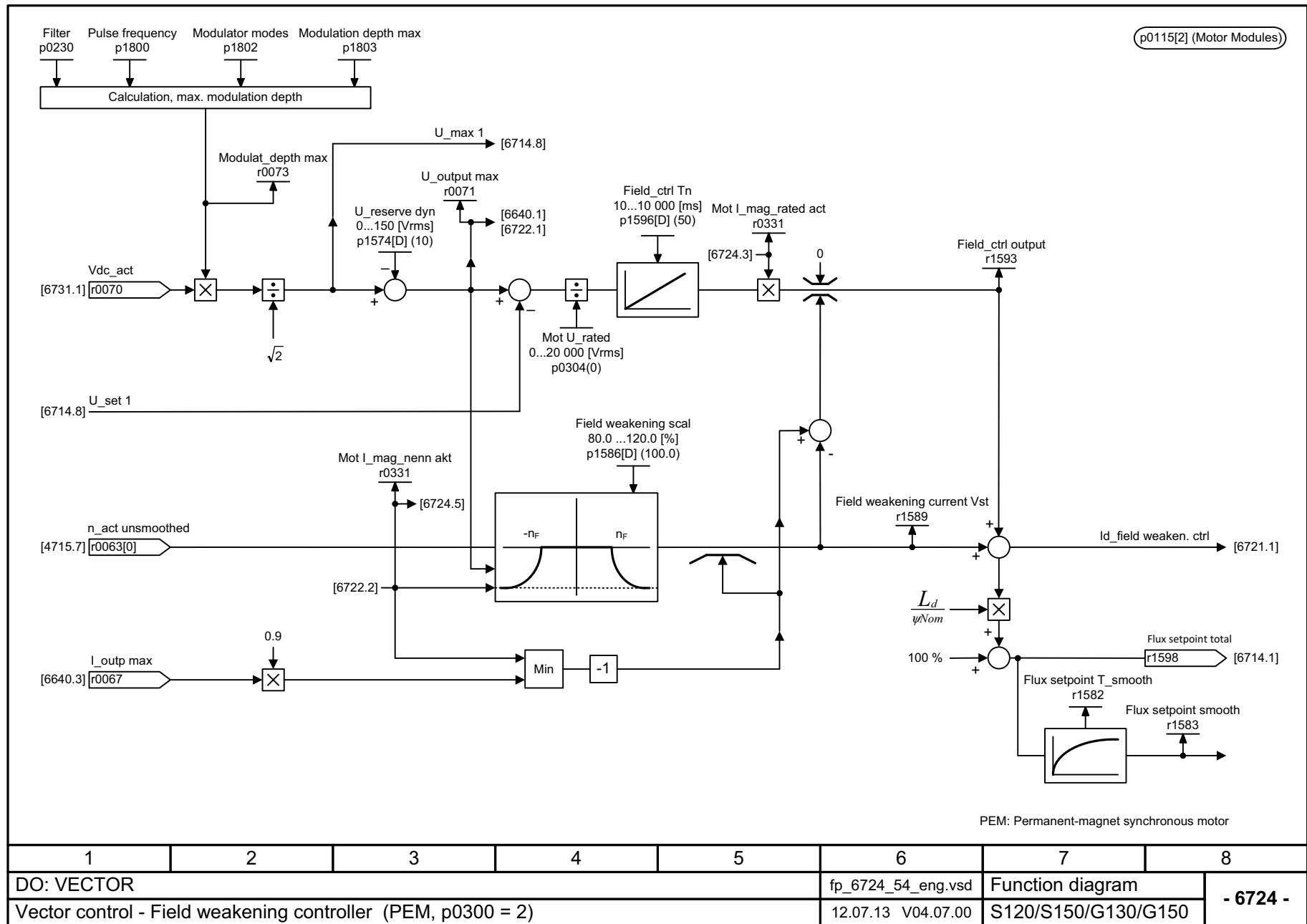
Fig. 3-138 6724 – Field weakening controller (PEM, p0300 = 2)
