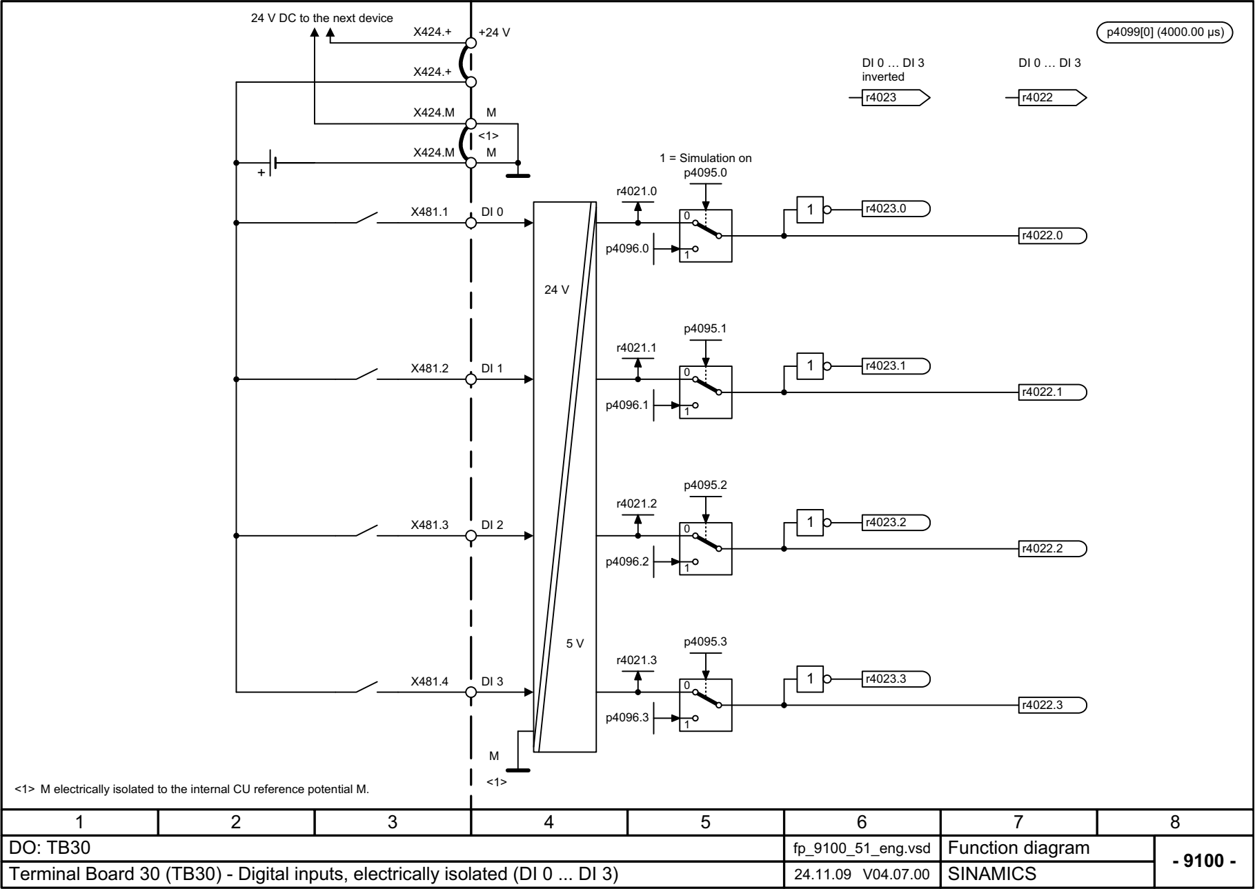
Fig. 3-180 9100 – Digital inputs, electrically isolated (DI 0 ... DI 3)
