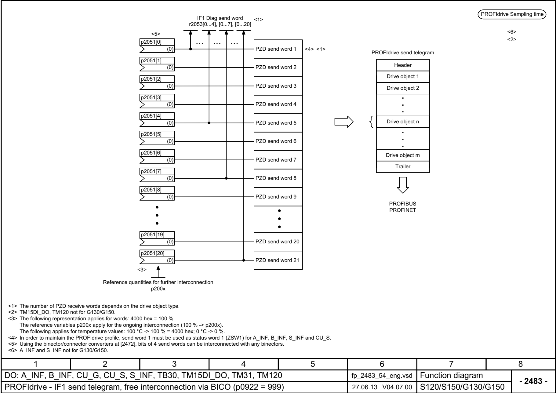
Fig. 3-45 2483 – IF1 send telegram, free interconnection via BICO (p0922 = 999)
