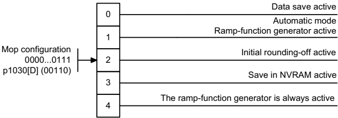
3020 – Motorized potentiometer
