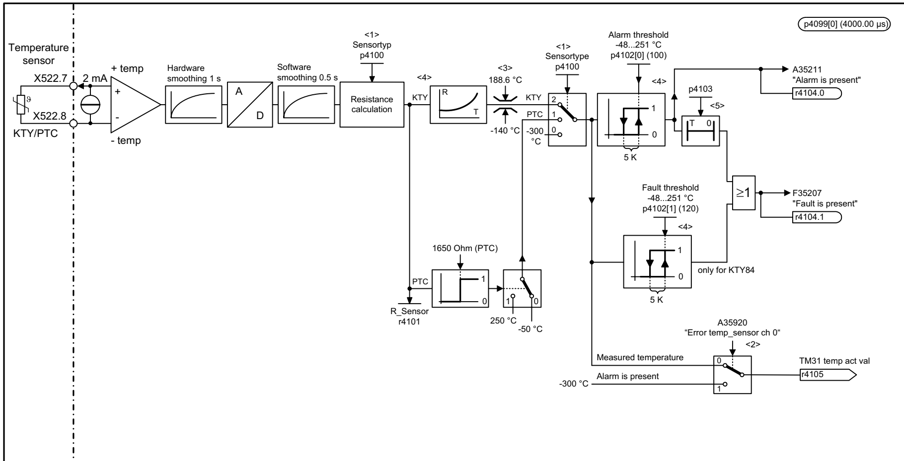
Fig. 3-199 9576 – Temperature evaluation (KTY/PTC)
