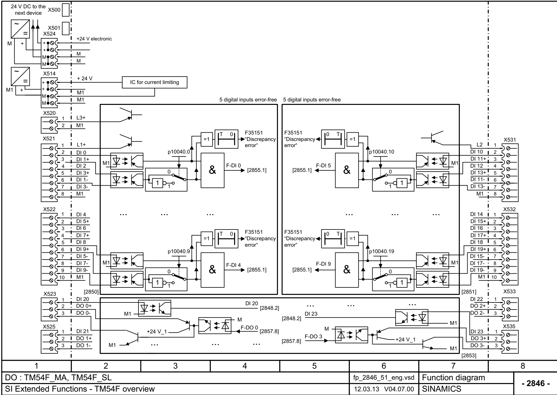
Fig. 3-94 2846 – TM54F overview
