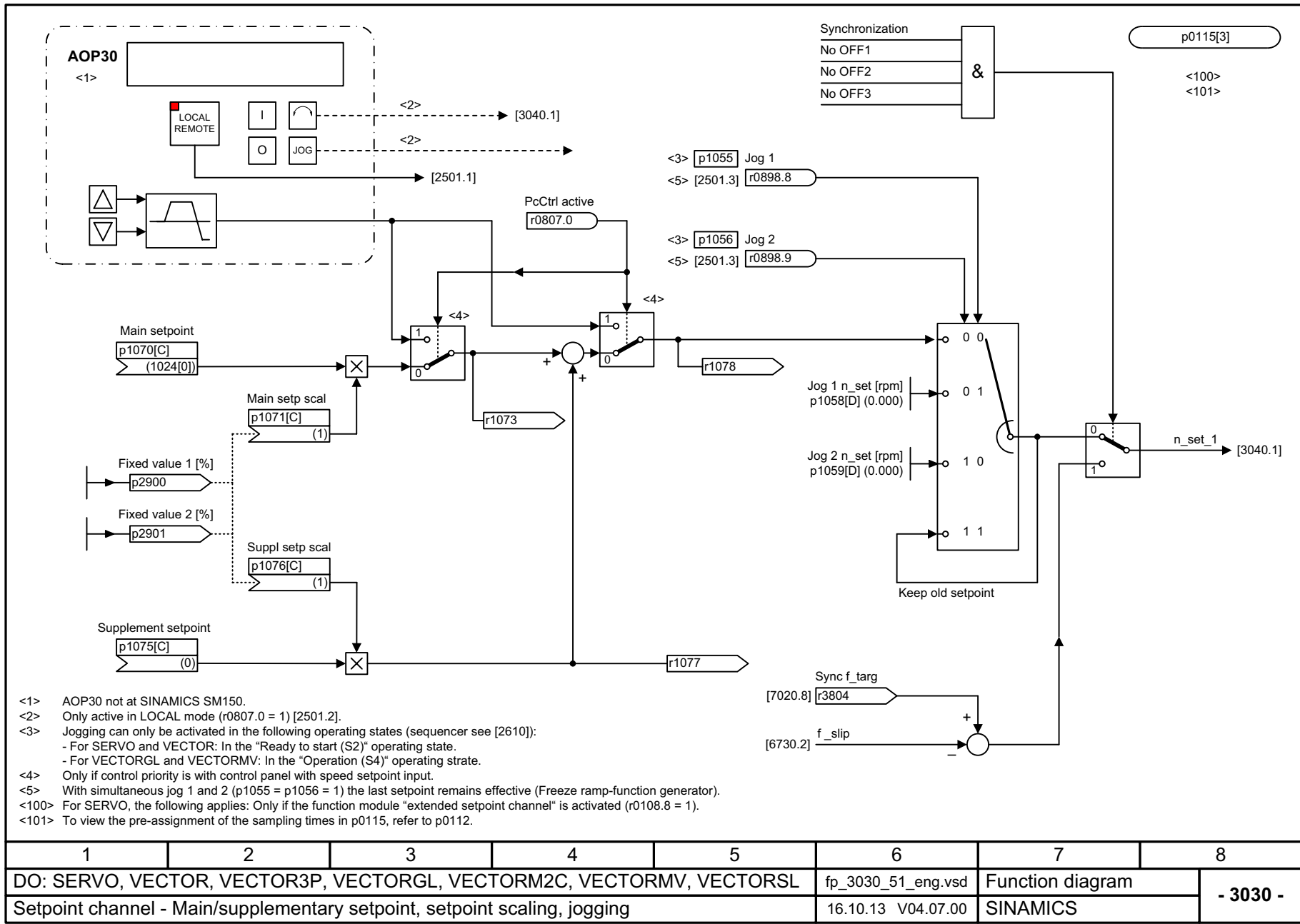
Fig. 3-108 3030 – Main/supplementary setpoint, setpoint scaling, jogging
