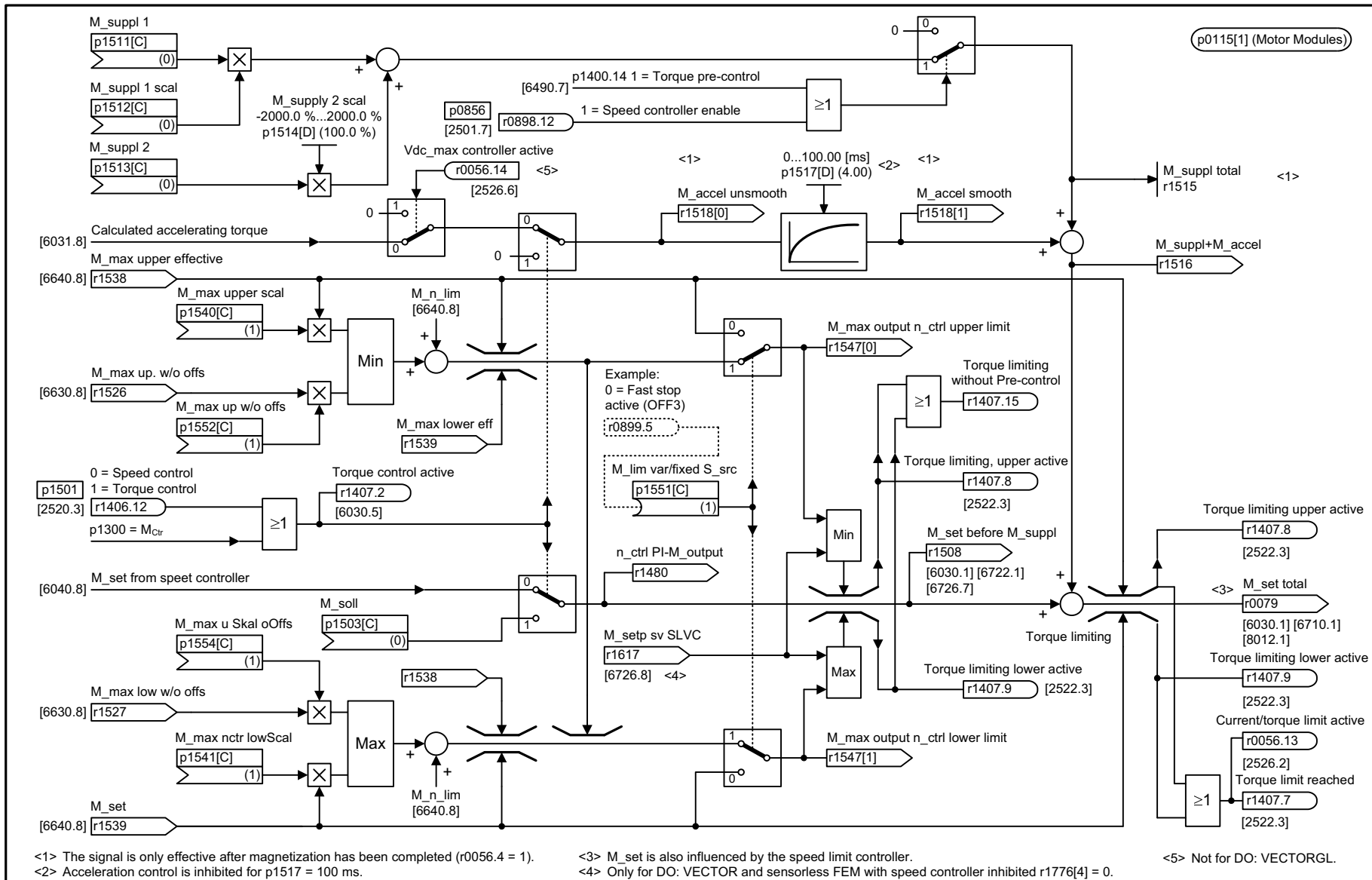
Fig. 3-122 6060 – Torque setpoint
