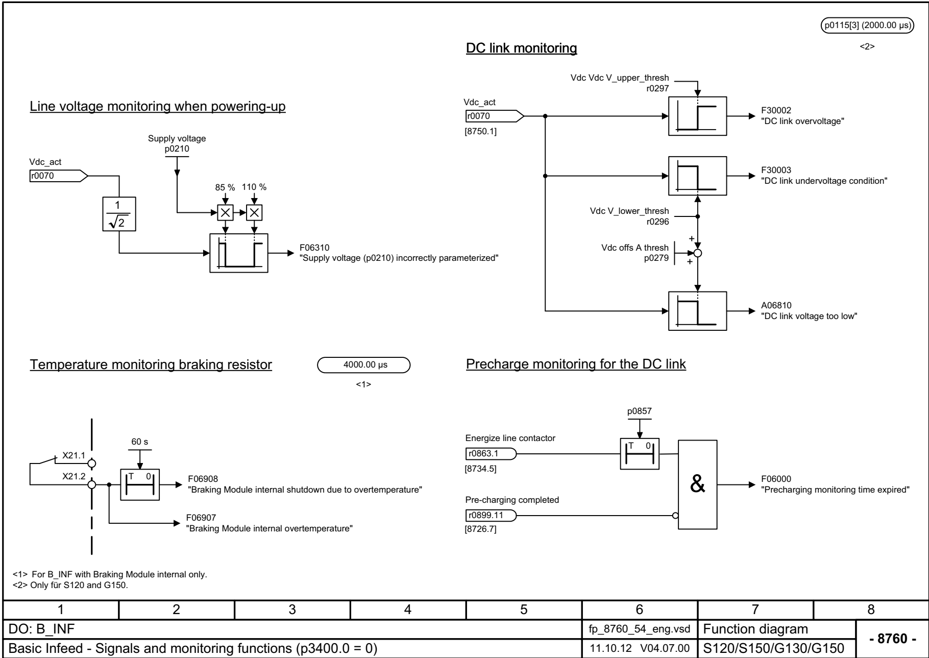
Fig. 3-178 8760 – Signals and monitoring functions (p3400.0 = 0)
