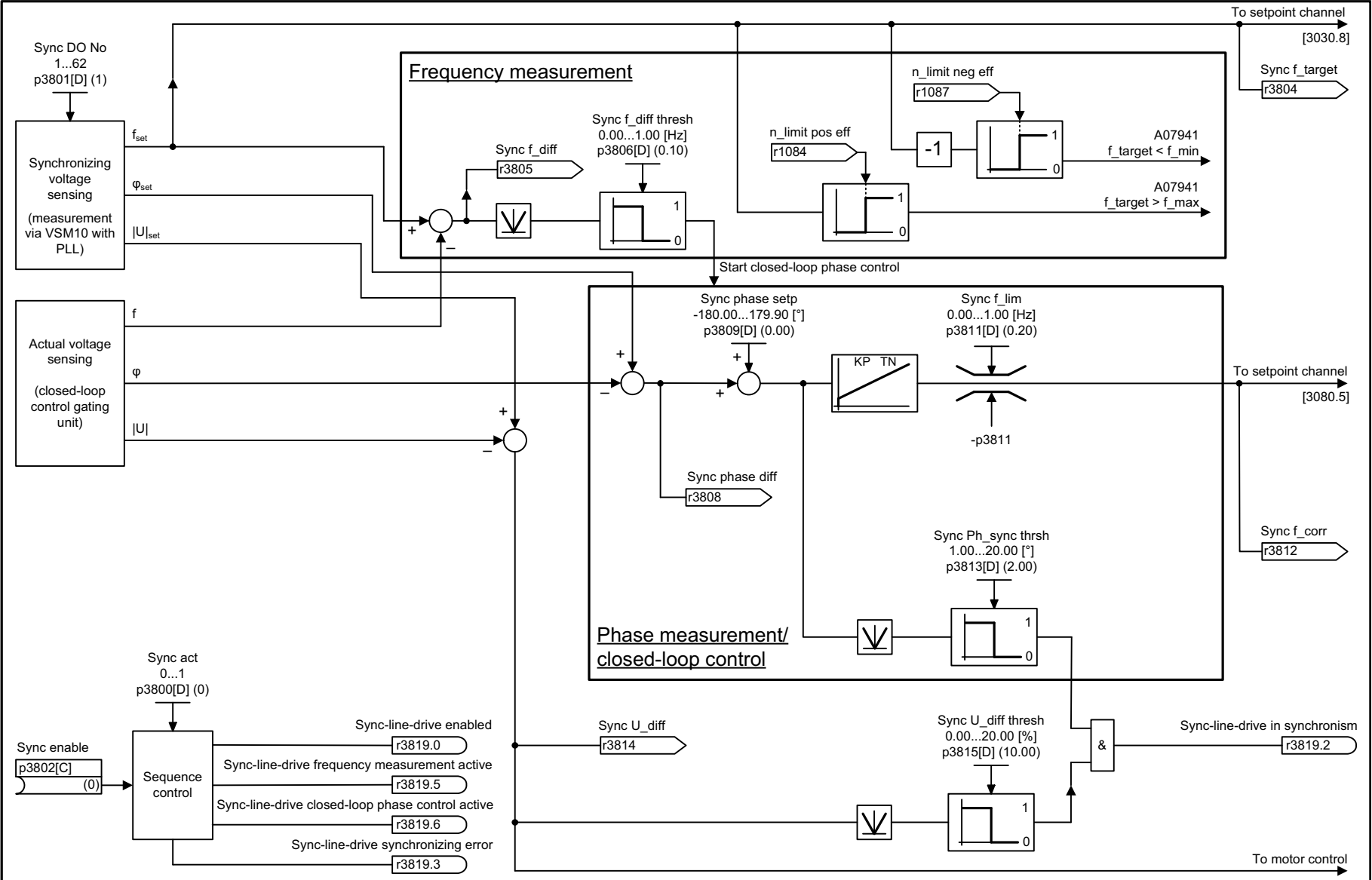
Fig. 3-146 7020 – Synchronization
