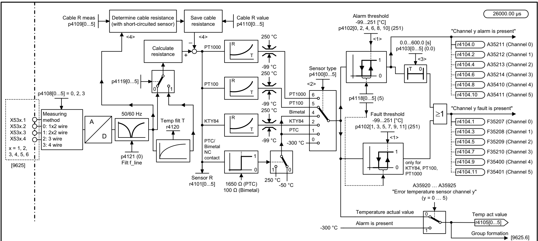
Fig. 3-201 9626 – Temperature evaluation 1x2, 3, 4 wire (channels 0 ... 5)
