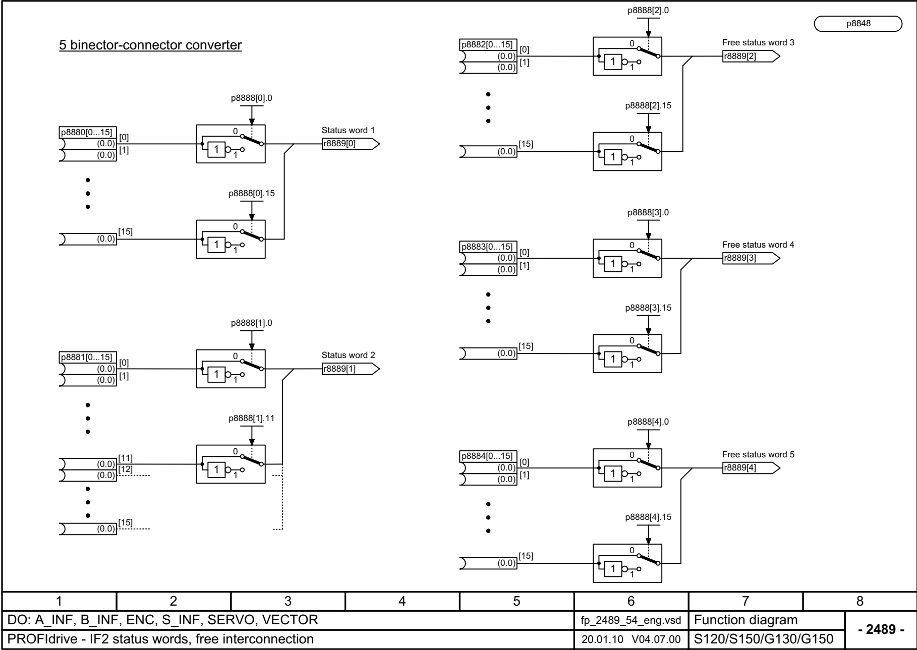
Fig. 3-48 2489 – IF2 status words, free interconnection
