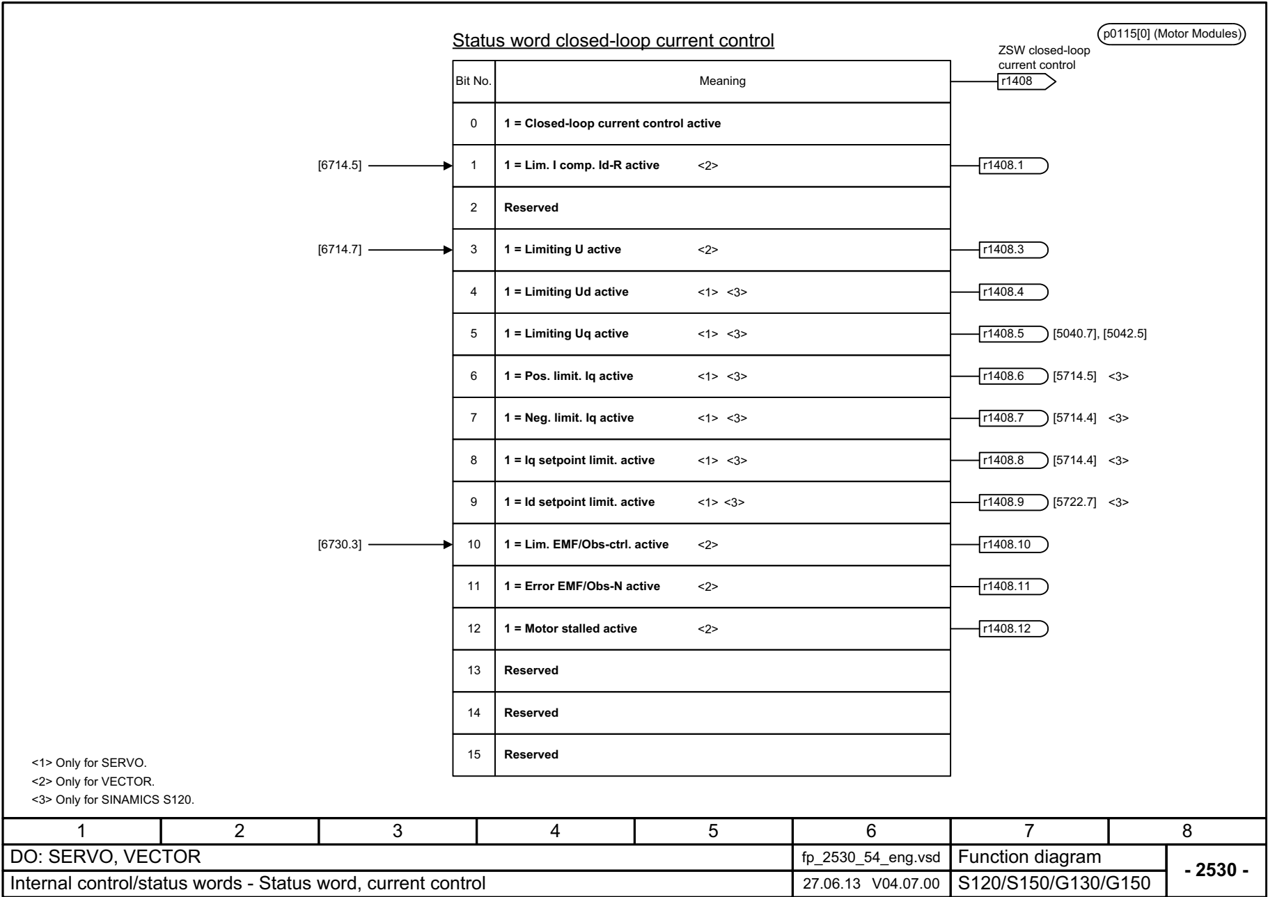
Fig. 3-63 2530 – Status word, closed-loop current control
