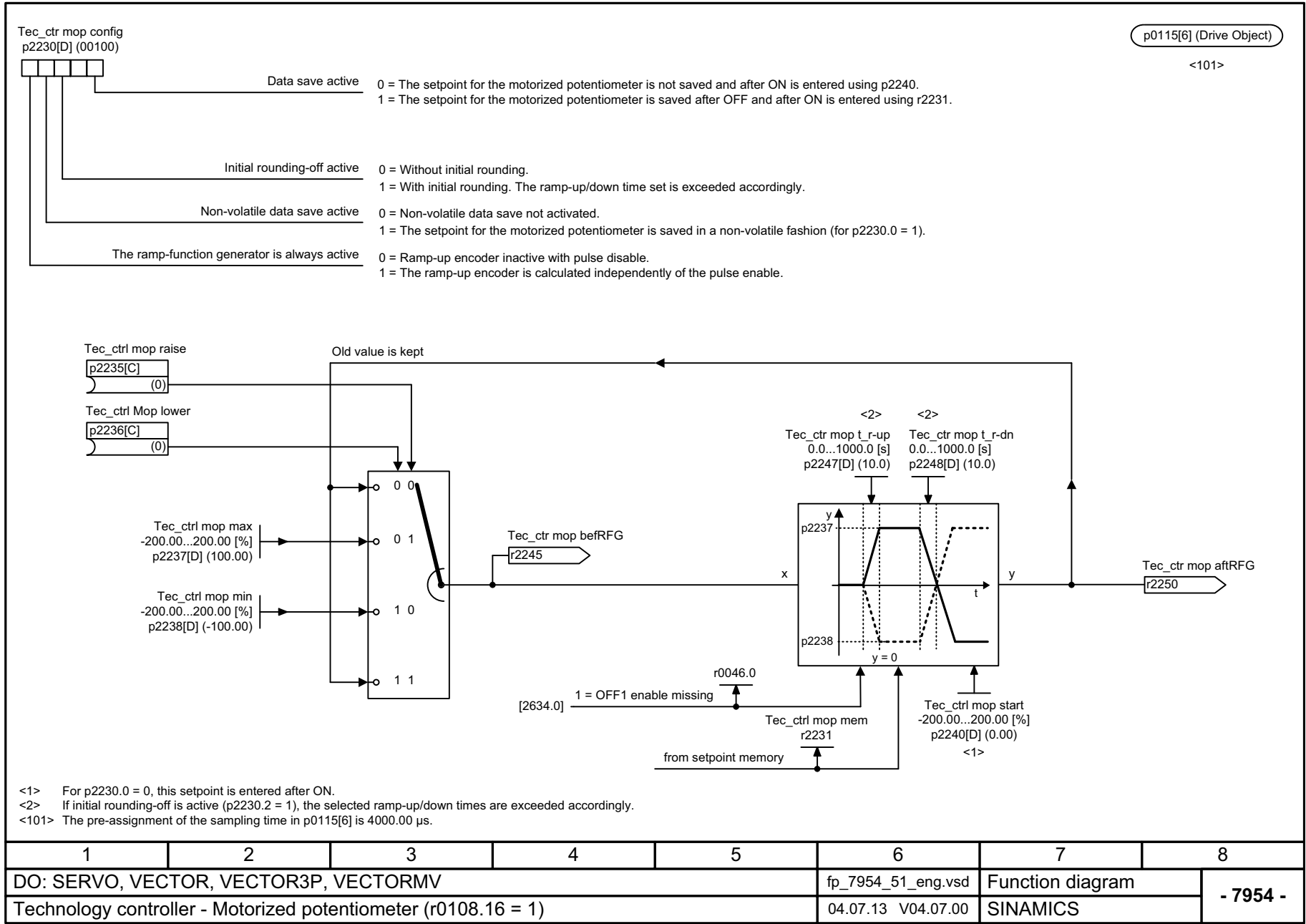
Fig. 3-150 7954 – Motorized potentiometer (r0108.16 = 1)
