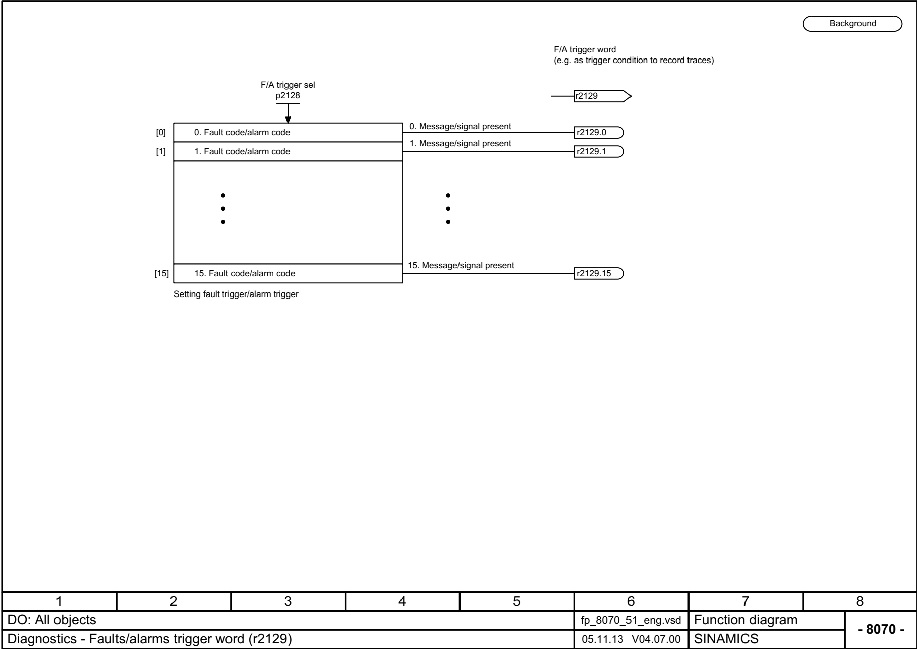
Fig. 3-164 8070 – Faults/alarms trigger word (r2129) SINAMICS G130/G150 List Manual (LH2), 04/2014, A5E03263479A
