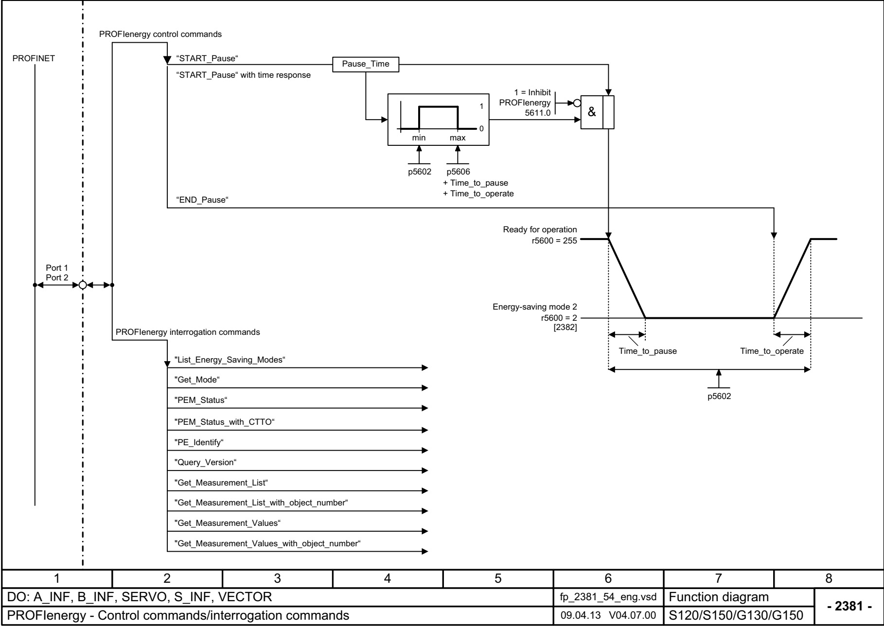
Fig. 3-12 2381 – Control commands / interrogation commands
