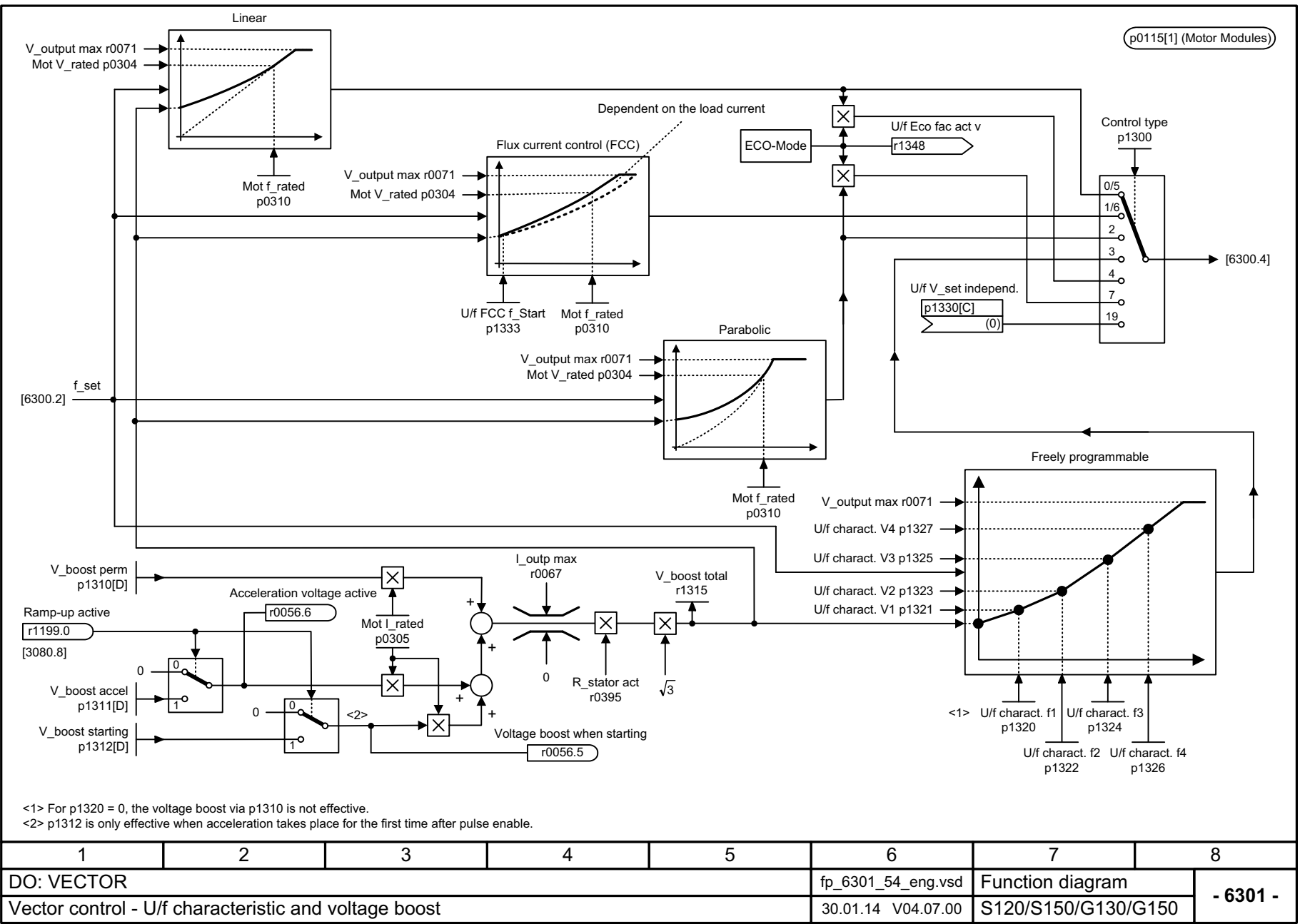
Fig. 3-125 6301 – U/f characteristic and voltage boost
