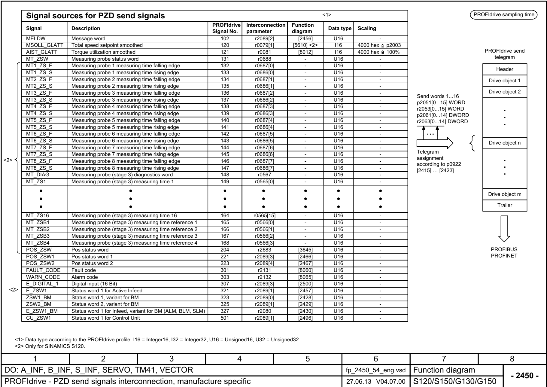
Fig. 3-36 2450 – PZD send signals interconnection, manufacturer-specific
