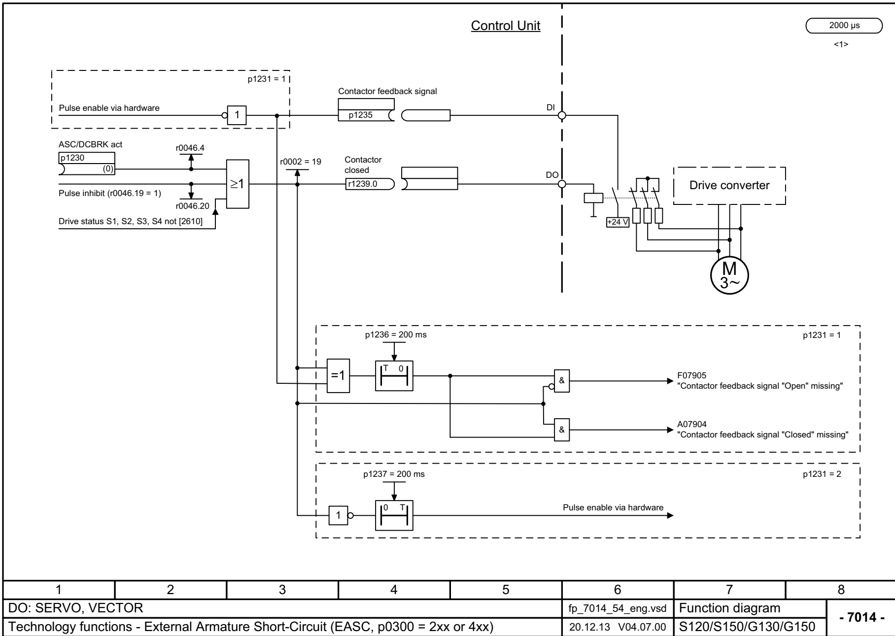
Fig. 3-143 7014 – External Armature Short-Circuit (EASC, p0300 = 2xx or 4xx)
