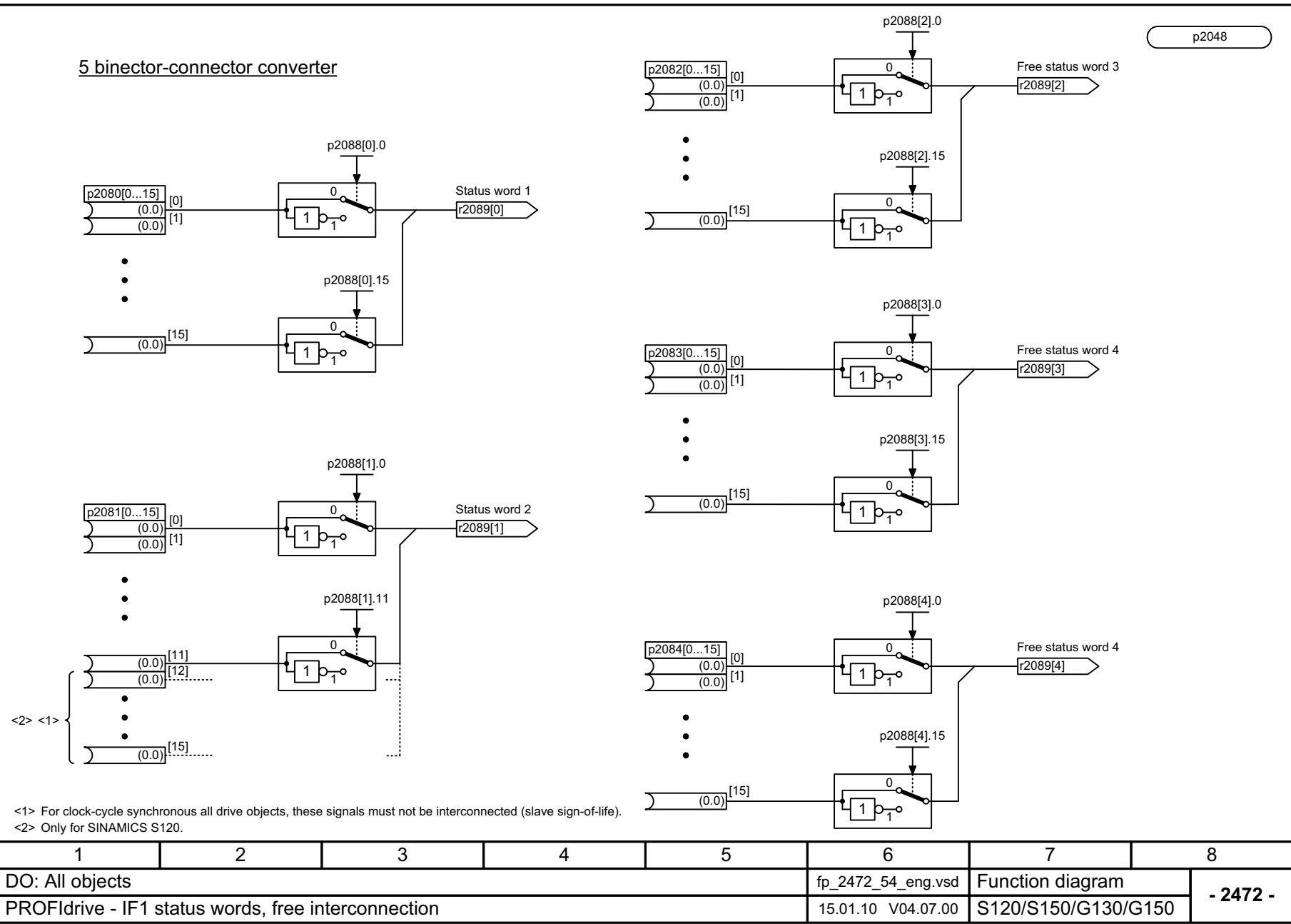
Fig. 3-43 2472 – IF1 status words, free interconnection
