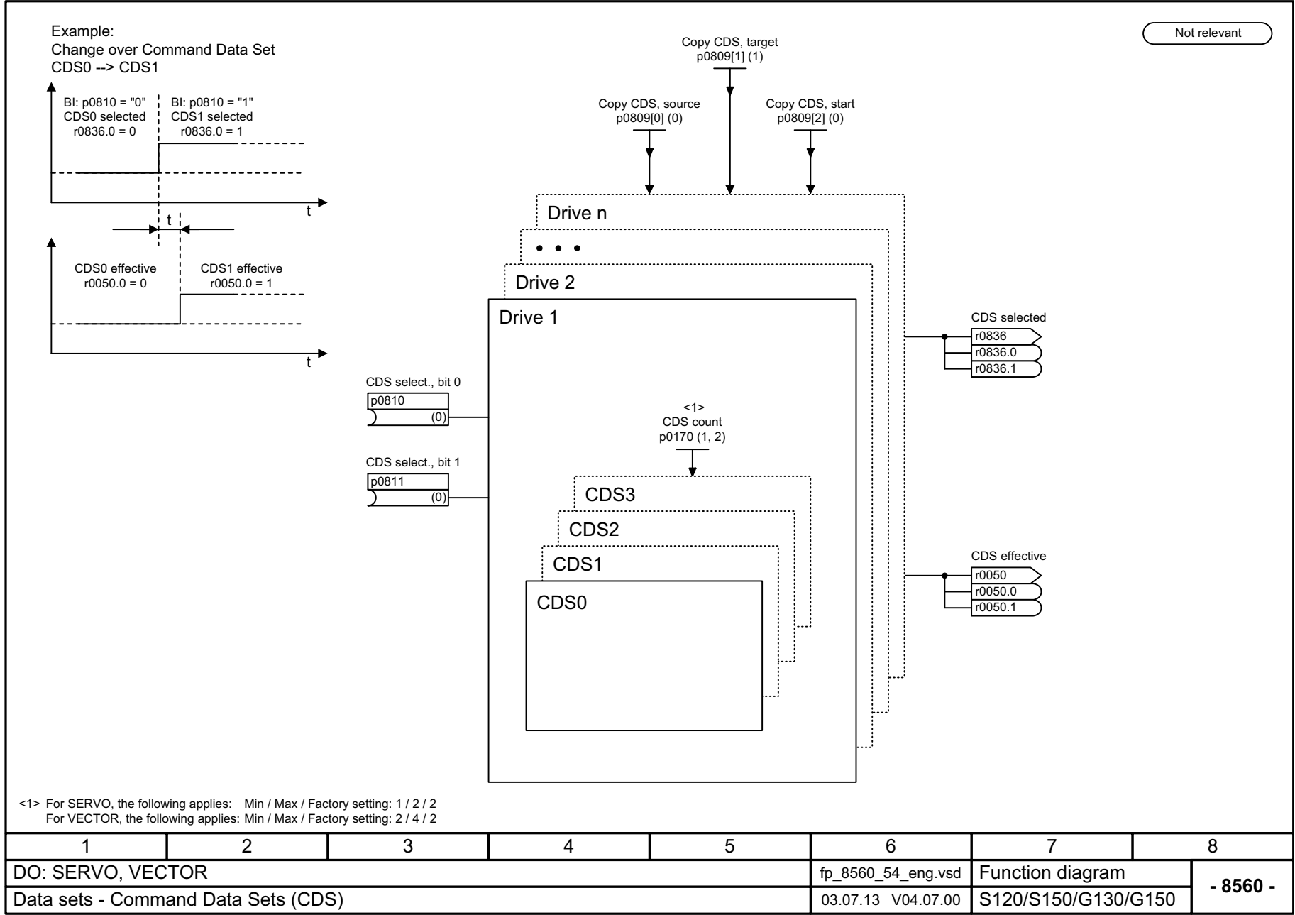
Fig. 3-167 8560 – Command Data Sets (CDS)
