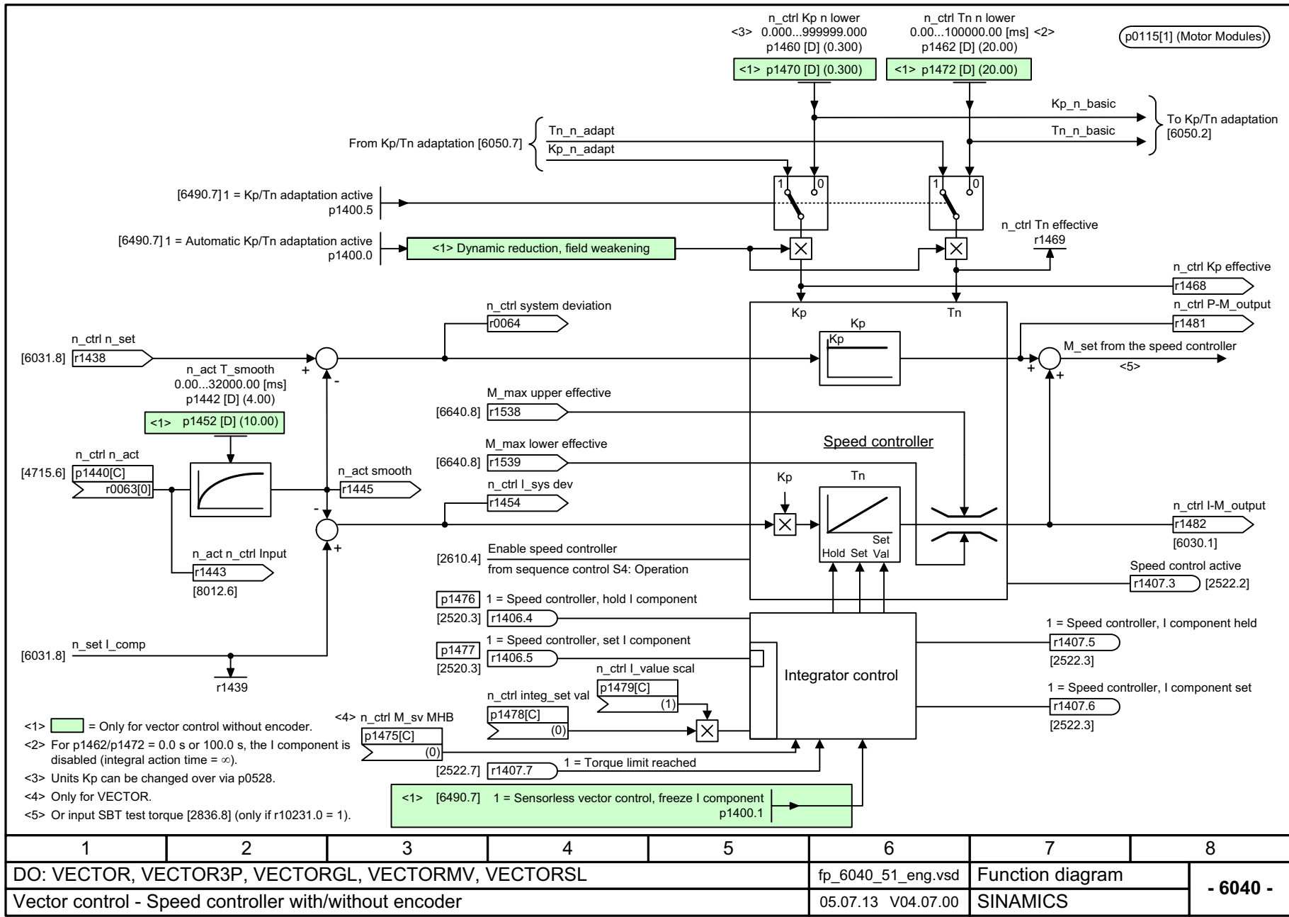
Fig. 3-120 6040 – Speed controller with/without encoder
