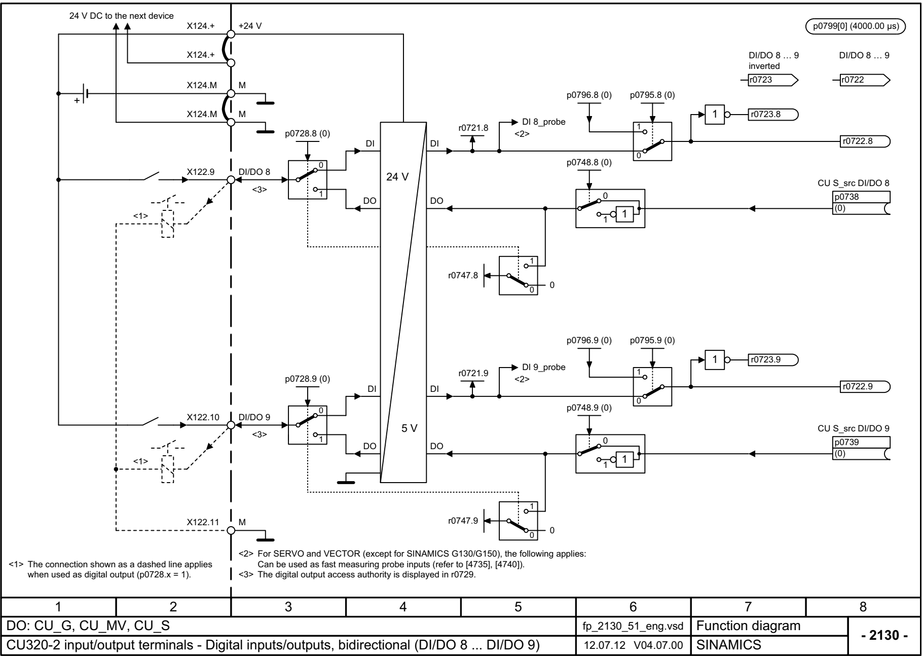
Fig. 3-8 2130 – Digital inputs/outputs, bidirectional (DI/DO 8 ... DI/DO 9)
