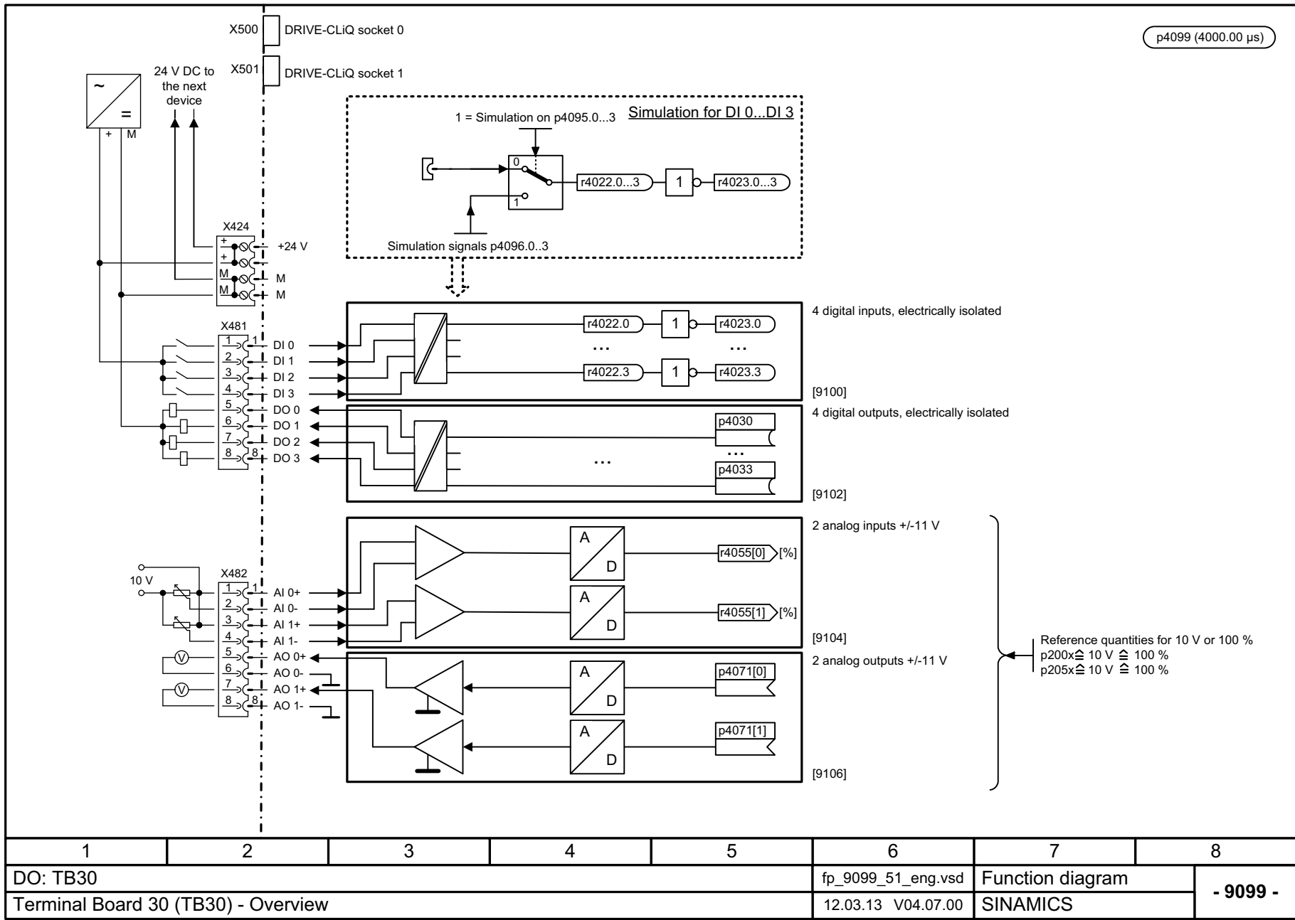
Fig. 3-179 9099 – Overview
