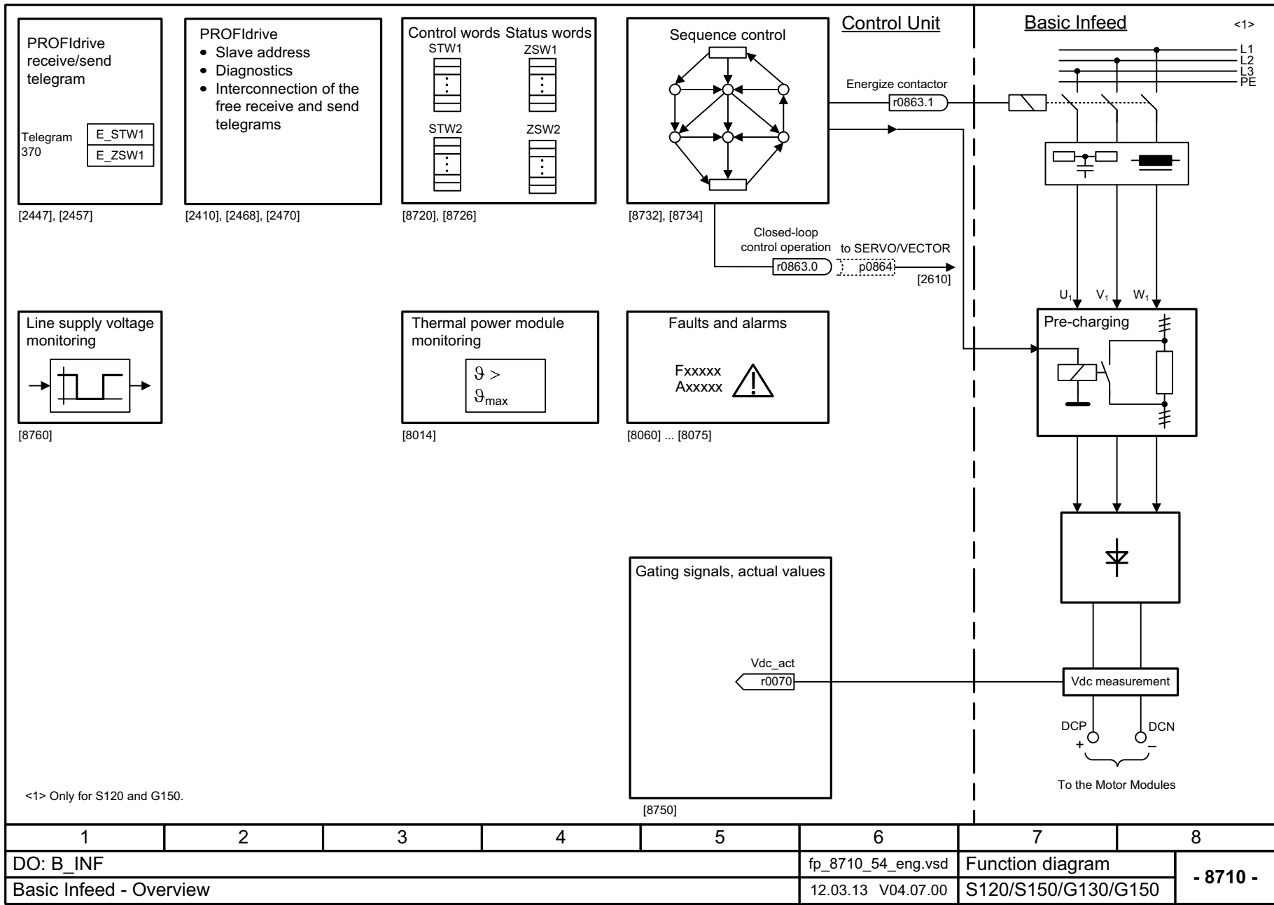
Fig. 3-172 8710 – Overview
