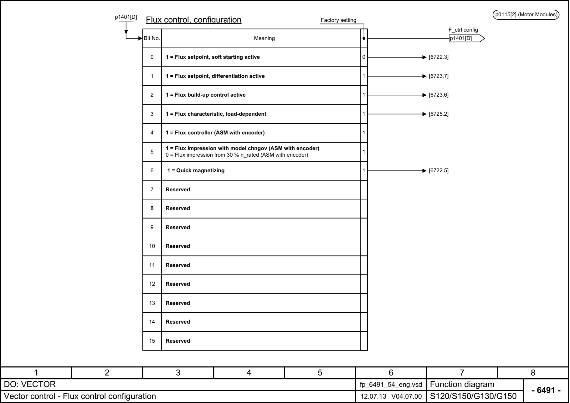
Fig. 3-129 6491 – Flux control configuration
