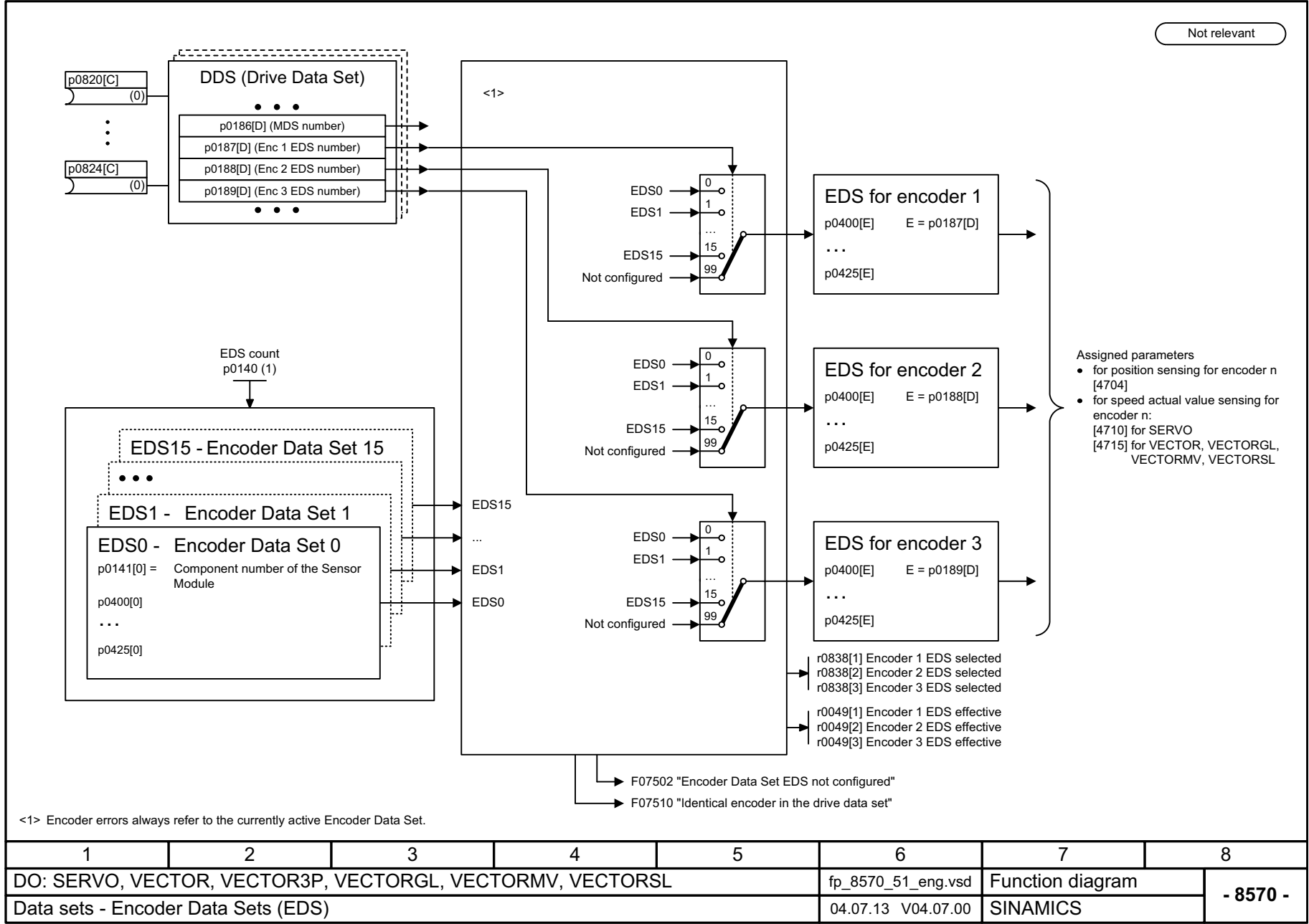
Fig. 3-169 8570 – Encoder Data Sets (EDS)
