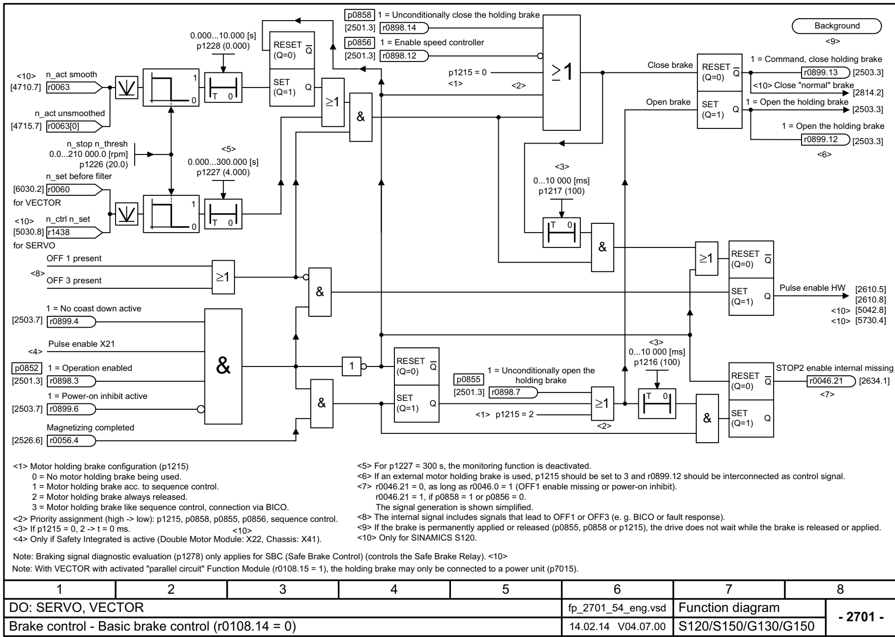
Fig. 3-71 2701 – Basic brake control (r0108.14 = 0)
