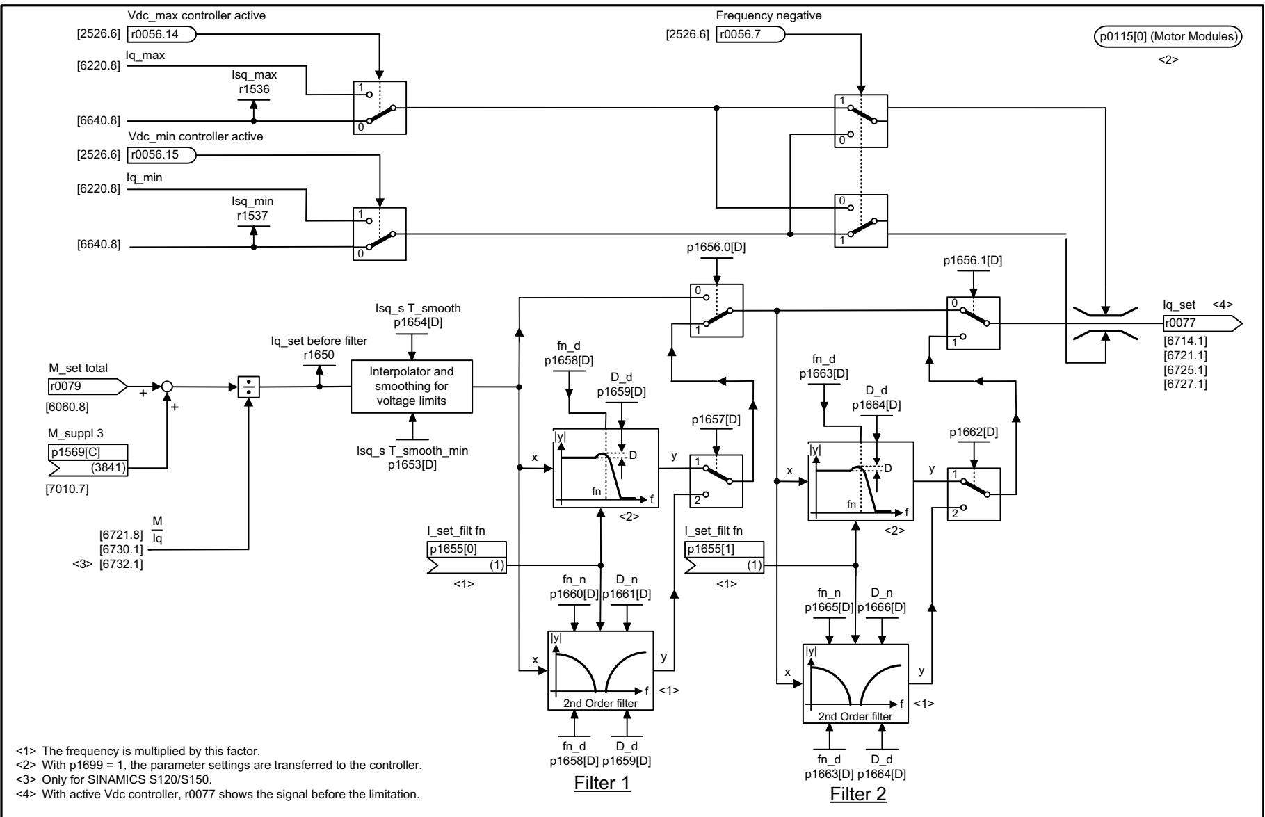
Fig. 3-133 6710 – Current setpoint filter
