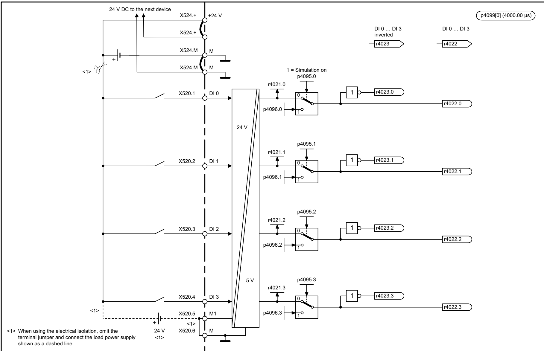
Fig. 3-191 9550 – Digital inputs, electrically isolated (DI 0 ... DI 3)
